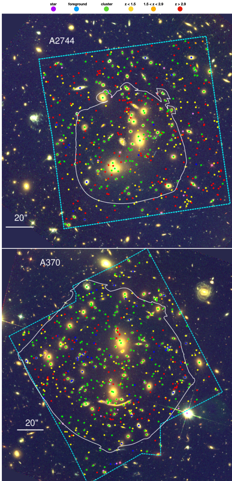
Fig. 7. Location of MUSE spectroscopic redshifts over HST F606W-F814W-F160W color composites. North is up and East is left. The cyan dashed lines represent the limits of the MUSE datasets, while the solid white contour highlights the region where strongly-lensed multiple images are expected.
