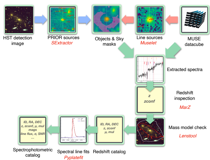
Fig. 4. Flowchart presenting the process of building the MUSE spectroscopic catalogues, based on the input HST images and MUSE datacube. Sect. 3 presents each step of the procedure in detail.
