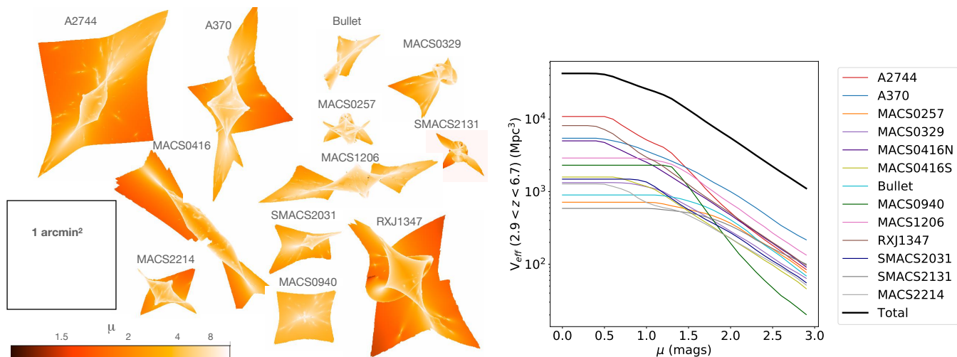
Fig. 11. (Left panel) Source plane coverage of each cluster at z = 4 , as a function of the strong lensing magnification of the brightest image. The black square shows a 1 \text{ arcmin}^2 for scale. (Right panel) Effective volume surveyed at 2.9 < z < 6.7 with MUSE for Lyman- \alpha emitters, as a function of the magnification of the brightest image. Presented are individual volumes behind each cluster and the total over all fields.
