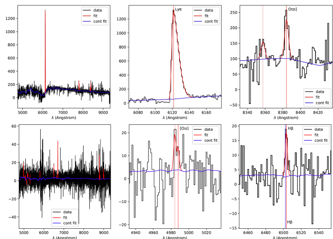
Fig. 6. Examples of PYPLATEFIT spectral fitting, for two sources in our catalogs. Top row shows the case of the bright z = 4.03 galaxy in MACS0940 (Claeysens et al. 2019) with z_{\text{conf}} = 3 and the bottom row a MUSELET-selected galaxy at z = 0.337 and z_{\text{conf}} = 2 in the same cluster field (M364). The left panel gives an overview of the spectrum, while the middle and right panels zoom in on specific spectral line fits. The best-fit spectrum and global continuum fit are plotted in red and blue, respectively.
