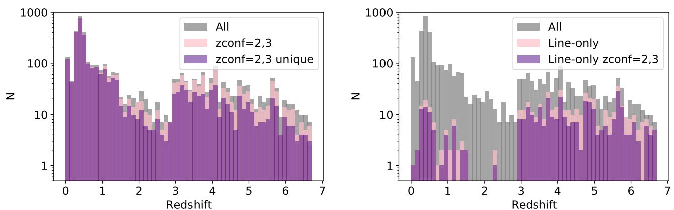
Fig. 8. Global redshift distribution of MUSE sources in the lensing cluster fields. Left panel: comparison between the overall distribution and sources with high confidence redshifts ( zconf = 2, 3 ), the latter before and after ("unique") accounting for image multiplicity. Right panel: comparison between the overall distribution and the line-only sources (pure line emitters without any HST counterpart, see Sect. 3.9).
