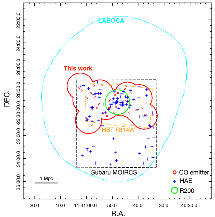
Fig. 5. The footprints of this work and previous studies, overlaid by CO sources (red circles) in this work and HAEs (blue crosses) in Koyama et al. (2013) and Shimakawa et al. (2018). The R_{200} radius (Shimakawa et al. 2014) is shown in a green circle centering on the MRC1138-262.
