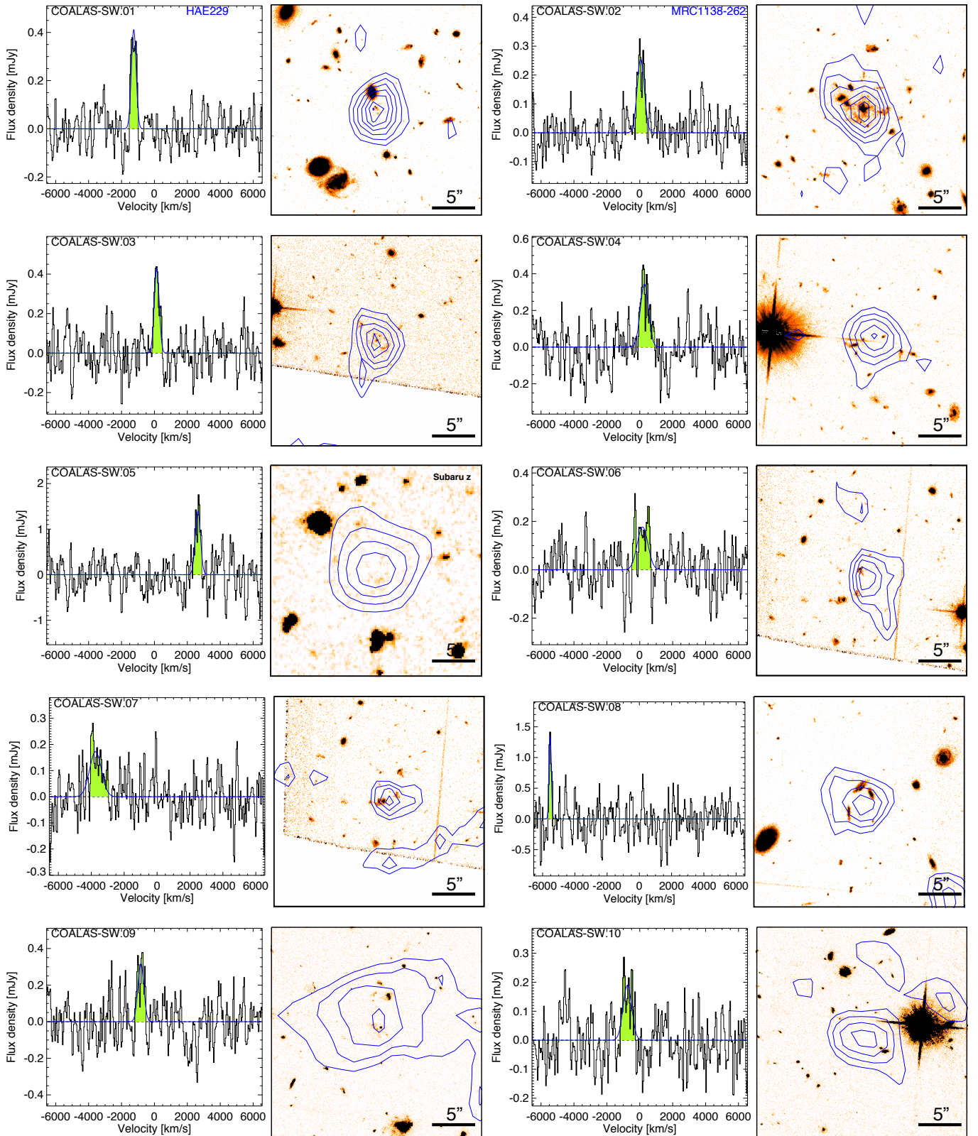
Fig. 3. The ATCA spectra and integrated CO maps for detections with \text{SNR} > 5 . Spectra panels: CO(1-0) lines are highlighted in green and fitted by a single Gaussian profile shown in red curve. Reference names in Emonts et al. (2016) and Dannerbauer et al. (2017) are highlighted in blue when available. Image panels: Optical images in 25'' \times 25'' size overlaid with CO(1-0) intensity contours. In general, images are taken from the HST F814W data (Miley et al. 2006), while VLT K_s (Dannerbauer et al. 2014) and Subaru z-band images (Koyama et al. 2013) are indicated as text on upper-right corner. Contours start at 2\sigma in steps of 1\sigma .
