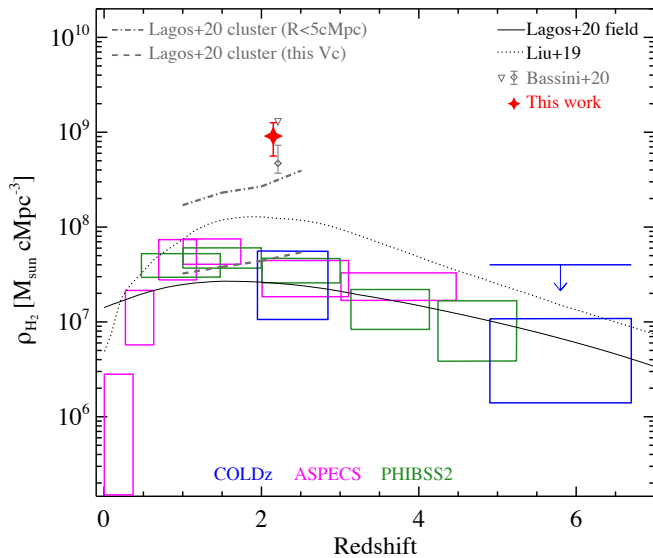
Fig. 9. H_2 density of this study (the red star) compared to results from COLDz (Riechers et al. 2019), ASPECS (Decarli et al. 2020) and PHIBSS2 (Lenić et al. 2020) overlaid by fitting of field galaxy samples from Liu et al. (2019) and Lagos et al. (2020). Gas density in galaxy clusters from simulations are shown in gray curves for SHARK (Lagos et al. 2020) in two volumes, and gray diamond with a bar for DIANOGA (Bassini et al. 2020), respectively. The gray diamond with error bar shows the median, and the downward triangle marks the maximum values for cluster structures in DIANOGA simulations. The gas density in this work is significantly higher than observed in blank fields and also higher than predictions for clusters in simulations.
