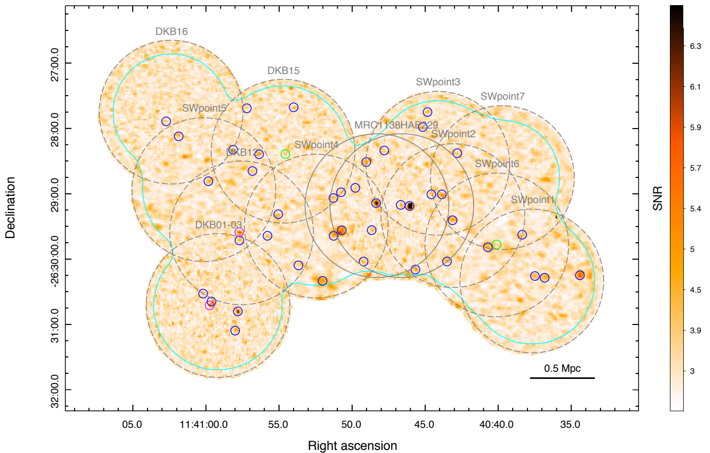
Fig. 1. The SNR map of line candidates (Sec. 3.1) in the ATCA mosaic. The SNR is the maximum signal-to-noise ratio computed in the 1D spectrum on each pixel by our algorithm MaxFinder (see details in Sec. 3.1). The color bar values are limited in 1.5 < \text{SNR} < 6.5 for fair visibility of detections. ATCA pointings are shown in grey circles with a radius of 0.9' . Grey solid circles mark the pointings MRC1138 in Emonts et al. (2016) and HAE229 in Dannerbauer et al. (2017), respectively. Cyan contour encloses the area with \text{rms} < 1 \text{ mJy bm}^{-1} . Detected sources are marked by solid circles in colors, blue: category A; magenta: category B; green: category C (see details in Sec. 3.3).
