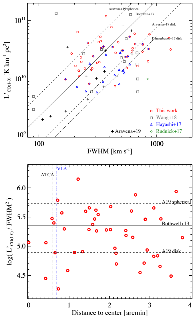
Fig. 7. Top panel: CO luminosity vs. FWHM. CO detections in this study are shown in red circles with HAEs marked by blue crosses. The dashed lines are from Aravena et al. (2019) where the upper line represents a spherical model and the bottom line a disk model. ASPECS galaxies (Aravena et al. 2019) are shown in black pluses which lie mostly along the disk model line. The solid line shows the relation from Bothwell et al. (2013), dot dashed line presents the disk model from Dannerbauer et al. (2017). Bottom panel: CO luminosity normalized by \text{FWHM}^2 vs. distance to the center galaxy. Vertical lines mark the half FWHM of ATCA (black) and VLA (blue) primary beams, respectively. This figure shows that CO emitters in Spiderweb cluster are more likely to be starbursts (mergers) compared to other high- z clusters, and these starbursts are beyond the FoV of the single pointing focusing on the central galaxy.
