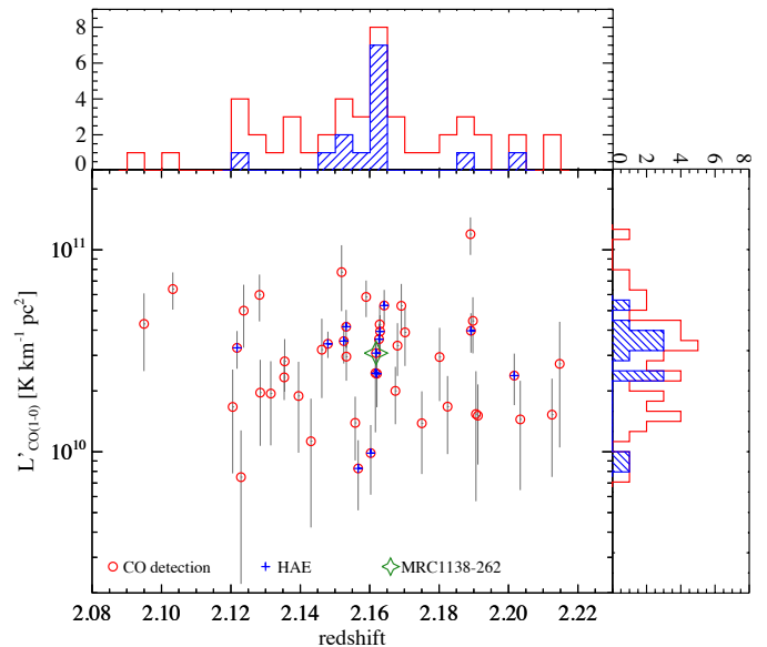
Fig. 4. CO luminosities vs. redshifts for CO detections in this study. Top and right panels show the redshift and CO luminosity distribution of our detections, respectively. In histograms, all CO emitters are shown in red, and HAEs with CO detections are shown in blue.
