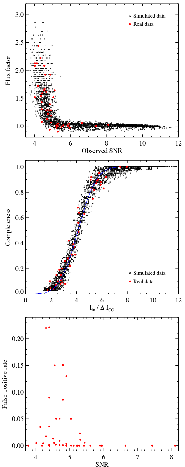
Fig. 2. Top panel: The flux boosting factor vs. observed SNR for simulated data (open circle) and real detections (red filled circle). Central panel: The completeness as a function of the injected line flux I_{in} over the measured flux uncertainty \Delta I_{CO} . The I_{in} for real detections are line fluxes that have been corrected for flux boosting factors in the top panel. The blue curve shows the best fit to the simulated data (see Eq. 3). The completeness decreases with decreasing integrated flux normalized by noise, indicating that sources are more difficult to detect at low SNR. This analysis allows us to correct CO luminosity functions for the completeness of our search algorithm. Bottom panel: The false positive rate vs. SNR for CO detections in this study.
