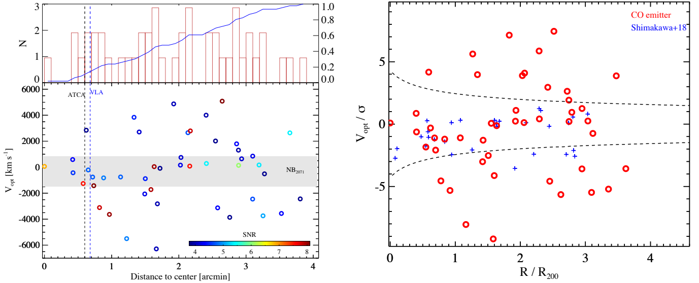
Fig. 6. Left panel: Distribution of CO emitters vs. their sky distances to the central radio galaxy MRC1138-262. Top panel shows histogram (red) and cumulative fraction (blue) of CO emitters as a function of the distances to the center galaxy. In the bottom panel, CO emitters are color-coded with their SNR. Grey shaded area marks the redshift range observed by the narrow band N_{2071} (Shimakawa et al. 2018) of MOIRCS at Subaru. Blue and black dashed lines mark the field of view of VLA and ATCA single pointing, respectively. Right panel: Normalized velocity vs. distance to center galaxy for CO emitters in this study and HAEs with a spectroscopic redshift (Shimakawa et al. 2018). The normalization factors are \sigma = 683 \text{ km s}^{-1} and R_{200} = 0.53 \text{ Mpc} (Table 2 in Shimakawa et al. 2014). The two dashed curves show the escape velocity (positive and negative) as a function of distance from the cluster mass 1.71 \times 10^{14} M_{\odot} (Shimakawa et al. 2014) using prescription in Rhee et al. (2017). Half of the CO emitters in this work have velocities outside of the region enclosed by these two curves which are not expected to be gravitationally bound to the central mass.
