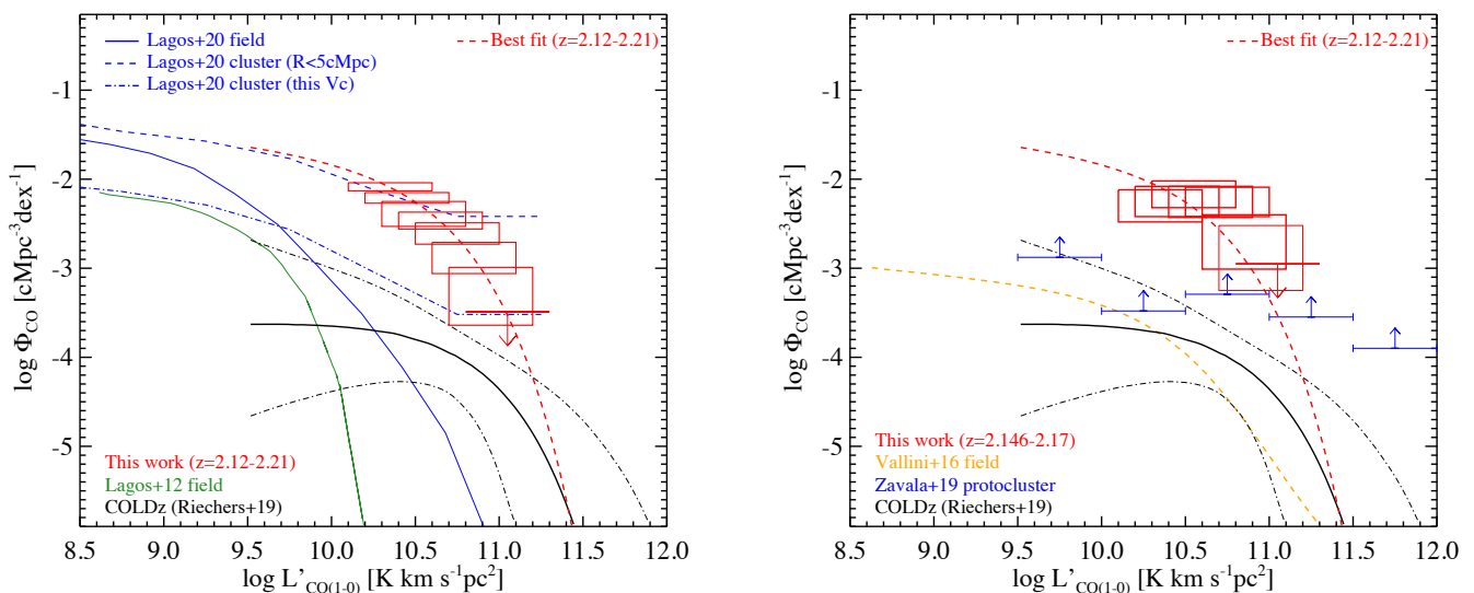
Fig. 8. The CO(1-0) luminosity functions for the Spiderweb cluster and samples from the literature. Left: CO(1-0) luminosity density in each luminosity bins at z = 2.12\text{--}2.21 in this work, compared with the results at z \sim 2 from the COLDz (Riechers et al. 2019), and predictions from semi-analytic SHARK models (Lagos et al. 2012, 2020). The dotted-dashed black lines mark the 5th and 95th percentile of the COLDz LF. Red dashed curve shows the best fit to our data. We show CO luminosity functions for protoclusters derived from SHARK models within two different volumes. One (blue dashed curve) is calculated in a spherical volume with radius R < 5 cMpc and the other one (blue dot-dashed curve) is in the identical volume to where the observed CO LF is measured, respectively. Right: Same as the left panel, but boxes are shown for CO luminosity density in a narrow redshift range z = 2.146\text{--}2.17 . Blue arrows mark the lower limits for protoclusters in Zavala et al. (2019), and orange curve shows the results from Vallini et al. (2016).
