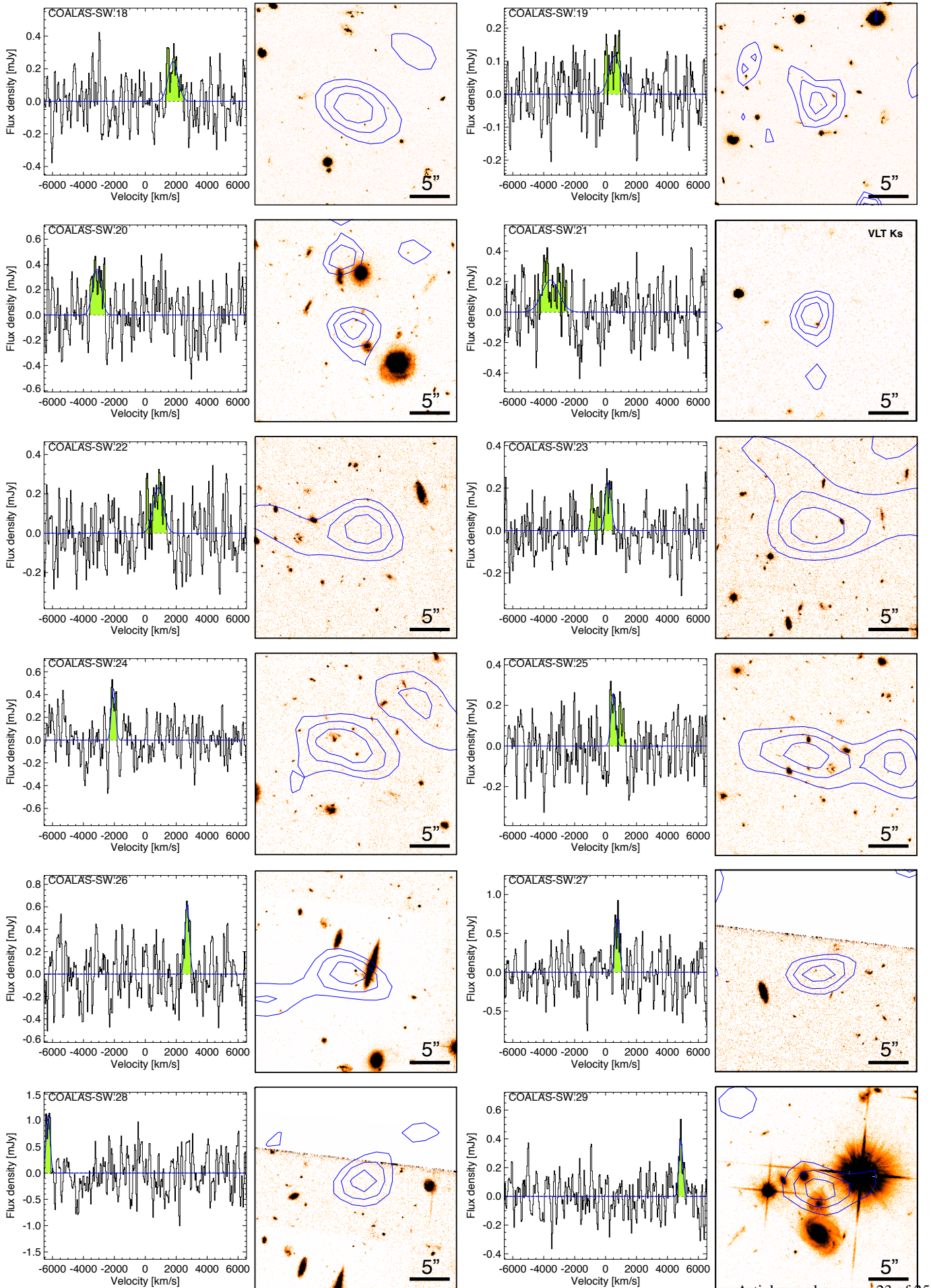
Fig. A.1. Spectra of SNR= 4–5 detections in category A. This figure shares caption in Fig. 3.
