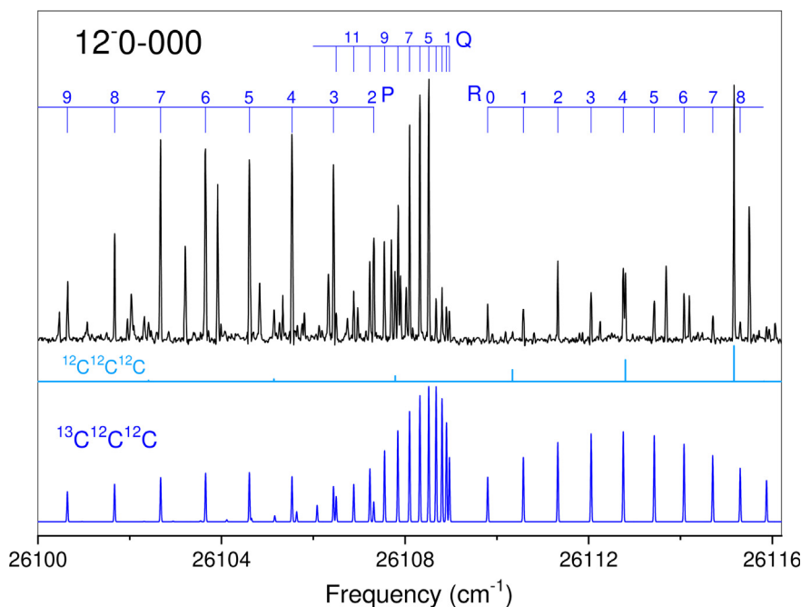
Fig. 9. The experimental (upper black trace) and simulated (lower blue trace) spectra of ^{13}C^{12}C^{12}C 12^-0-000 band. The rotational assignments are given by blue thin sticks on top of the experimental spectrum. A Gaussian linewidth of 0.02\text{ cm}^{-1} and a rotational temperature of \sim 30\text{ K} are used in the spectral simulation. Middle cyan trace is the simulated spectrum of ^{12}C_3 .
