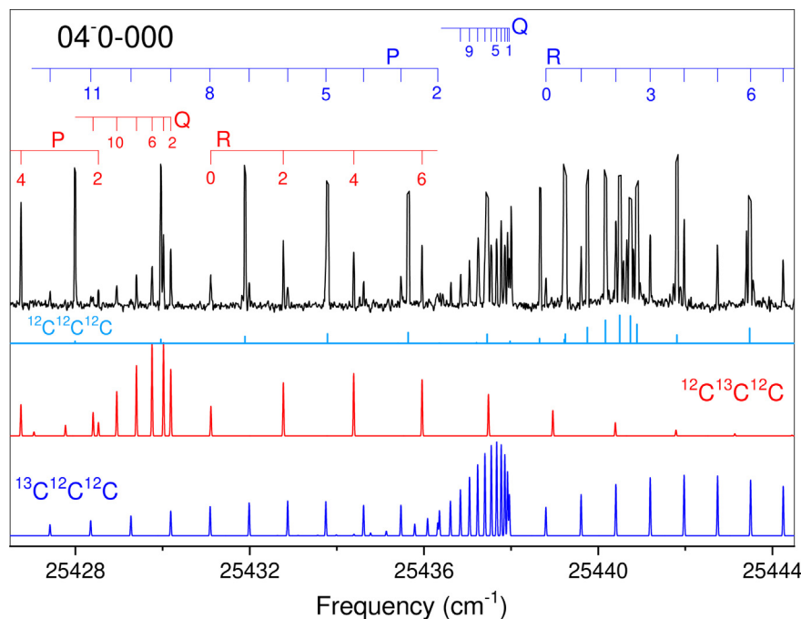
Fig. 8. The 04^-0-000 \Pi_u^- - \Sigma_g^+ band. Upper black trace is the recorded LIF spectrum, with ^{12}C_3 transitions being truncated. The rotational assignments of ^{12}C^{13}C^{12}C and ^{13}C^{12}C^{12}C are given by red and blue thin ticks, respectively, on the top of the spectrum. Lower traces are simulated spectra, with cyan for ^{12}C_3 , red for ^{12}C^{13}C^{12}C and blue for ^{13}C^{12}C^{12}C . A Gaussian linewidth of 0.02\text{ cm}^{-1} and a rotational temperature of \sim 30\text{ K} are used in the spectral simulations.
