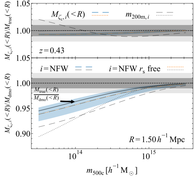
Figure 10. Top panel: The ratio of the total aperture mass within R < 1.5 h^{-1} \text{ Mpc} derived from mock weak lensing observations, to the true aperture mass. The coloured, dashed and dotted lines show the ratio of the aperture masses inferred for the best-fitting NFW density profiles, with fixed and free scale radius, respectively, to the true aperture mass using the statistic from Eq. (24). The gray dashed and dotted lines show the ratio of the measured and true deprojected masses, m_{200m, \text{NFW}}/m_{200m, \text{true}} , for the same NFW fits. For the aperture masses, there is practically no difference between using a fixed or free NFW scale radius, indicating insensitivity to the assumed density profile. The derived aperture mass is within 1 per cent of the true aperture mass for all halo masses. Bottom panel: The ratio of the total aperture mass within R < 1.5 h^{-1} \text{ Mpc} derived from mock weak lensing observations, to the same aperture mass of the equivalent DMO halo. Line styles are the same as in the top panel. The ratio of the true to the equivalent DMO halo aperture mass is shown as the solid, black line. The aperture masses are less biased with respect to the equivalent DMO masses than the deprojected masses, m_{200m} , which are shown as the gray lines.
