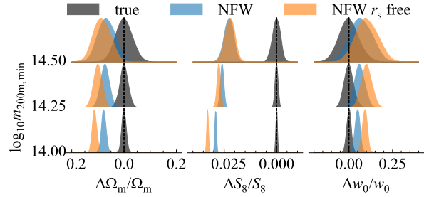
Figure 9. The marginalized maximum a-posteriori probability density functions for \Omega_m , S_8 = \sigma_8(\Omega_m/0.3)^{0.2} and w_0 for 1000 independent stage IV-like cluster abundance surveys with different mass cuts m_{200\text{m},\text{min}} . Gray PDFs show the results for a halo sample with no mass bias. Blue (orange) PDFs include a mass bias due to baryonic effects resulting from an NFW fit to mock weak lensing observations of the reduced shear, with a fixed (free) scale radius, r_s . The bias in S_8 is reduced by a factor of \approx 8 if the mass cut is increased from m_{200\text{m},\text{min}} = 10^{14} h^{-1} M_{\odot} to m_{200\text{m},\text{min}} = 10^{14.5} h^{-1} M_{\odot} , but is still highly significant, while the bias in \Omega_m and w_0 is reduced to within 2.5\sigma .
