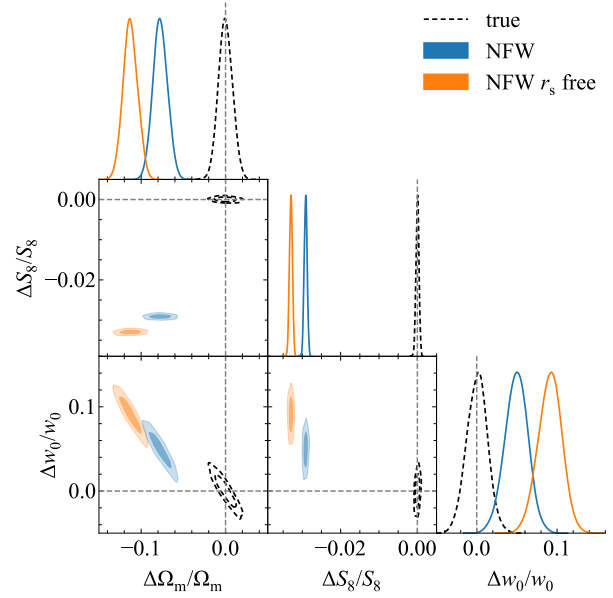
Figure 8. The distribution of the maximum a-posteriori probabilities in (\Omega_m, S_8 = \sigma_8(\Omega_m/0.3)^{0.2}, w_0) for 1000 independent stage IV-like cluster abundance surveys. Dashed contours show the results for a halo sample with no mass bias. Blue (orange) contours include a mass bias due to an NFW fit to mock weak lensing observations of the reduced shear, with a fixed (free) scale radius, r_s . Relative constraints on S_8 are very highly biased for both NFW fitting methods to the cluster density profiles including baryons. Similarly, \Omega_m and w_0 are biased by up to 14\sigma and 6\sigma , respectively.
