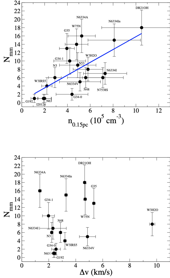
Fig. 5.— Top: Fragmentation level vs density averaged within the same field of view where fragmentation, line width and PA dispersion were assessed (0.15 pc of diameter). Bottom: Fragmentation level vs line width of the \text{H}^{13}\text{CO}^+ (4–3).
