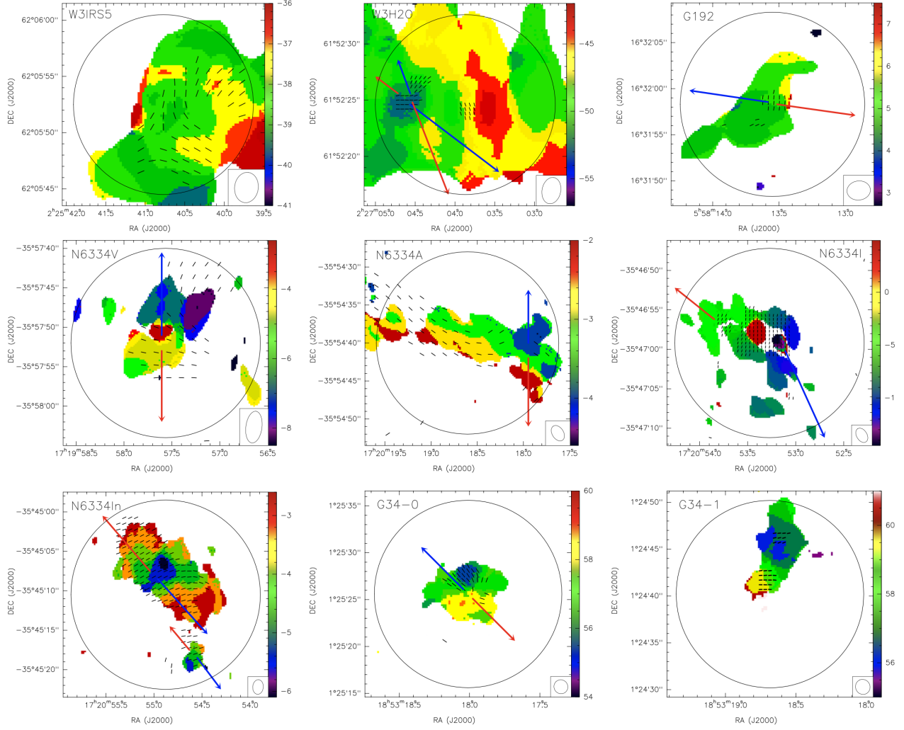
FIG. 14A.— First-order moments for \text{H}^{13}\text{CO}^+ (4–3) data with the magnetic field segments (black) overplotted. Red and blue arrows indicate the approximate orientations of the redshifted and blueshifted outflow emission according to Zapata et al. (2011), and Zhang et al. (2014). The synthesized beam is shown in the bottom-right corner. The circle corresponds to the field of view of 0.15 pc of diameter used in this work to assess the magnetic field strength. Wedge units are \text{km s}^{-1} .
