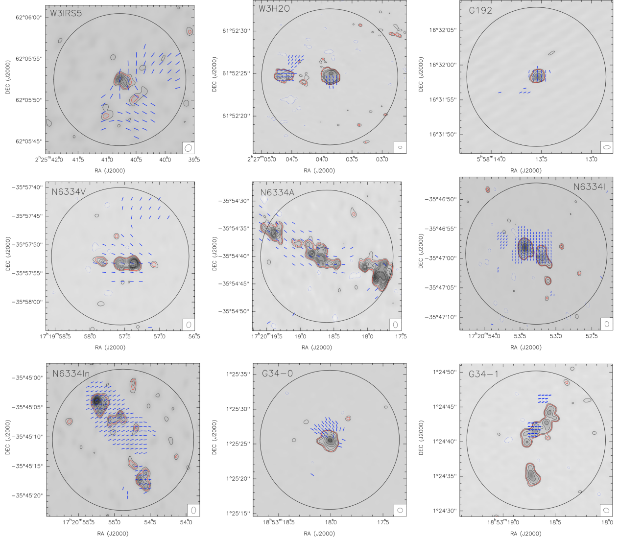
FIG. 2A.— 0.87 or 1.3 mm continuum high angular resolution maps with the magnetic field segments overplotted in blue. Contours for all regions are -4, 4, 8, 12, 16, 20, 24, 28, 36, 40, 50, 60, 70, 80, 100 and 120 times the rms noise, listed in Table 1, except for G192, N6334I, G34-0, and G34-1, for which contours are -4, 4, 8, 16, 32, 64 , and 128 times the rms noise. For W3H2O contours are -4, 4, 8, 16, 24, 32, 64, 120 times the rms noise. Synthesized beams are plotted in the bottom-right corner of each panel, and the black circle corresponds to a field of view of 0.15 pc diameter (the field of view common to all the regions, given their primary beams).
