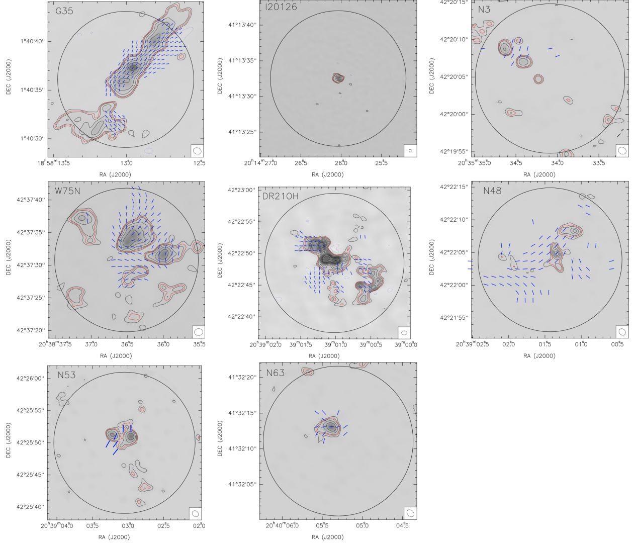
FIG. 2B.— 0.87 or 1.3 mm continuum high angular resolution maps with the magnetic field segments overplotted in blue. Contours for all regions are -4, 4, 8, 12, 16, 20, 24, 28, 36, 40, 50, 60, 70, 80, 100 and 120 times the rms noise, listed in Table 1, except for G35, I20126, W75N, N53 and N63 for which contours are -4, 4, 8, 16, 32, 64 , and 128 times the rms noise. Synthesized beams are plotted in the bottom-right corner of each panel, and the black circle corresponds to a field of view of 0.15 pc diameter (the field of view common to all the regions, given their primary beams).
