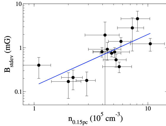
FIG. 15.— Magnetic field strength vs density averaged within 0.15 pc. The blue line corresponds to a linear fit in the log-log scale with a slope of 1.2.
