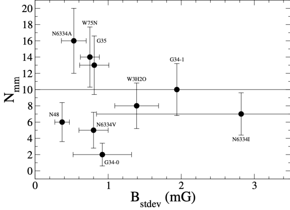
FIG. 11.— Fragmentation level vs magnetic field strength for regions with density in the range (4\text{--}8)\times 10^5 \text{ cm}^{-3} .
