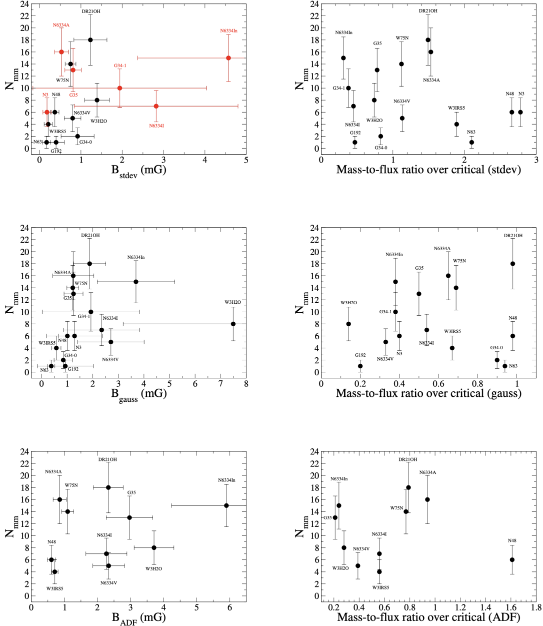
FIG. 10.— The three panels on the left show the plots of N_{\text{mm}} vs the magnetic field strength for the different approaches used in this work: ‘standard deviation’ ( B_{\text{stdev}} , top), ‘multiple gaussian’ ( B_{\text{gauss}} , middle), and ADF ( B_{\text{ADF}} , bottom). In the top-left panel, the red dots correspond to the cores classified as ‘aligned fragmentation’. The three panels on the right show the plots of N_{\text{mm}} vs the ratio of mass-to-flux to critical mass-to-flux for the same three approaches.
