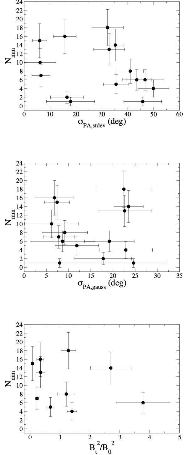
Fig. 6.— Top: Fragmentation level vs polarization PA intrinsic standard deviation of the weighted mean (Section 4.3.1). Middle: Fragmentation level vs polarization PA dispersion after fitting multiple PA components in the PA histograms (Section 4.3.2). Bottom: Fragmentation level vs energy ratio between the perturbed magnetic field and the large-scale ordered magnetic field (Section 4.4).
