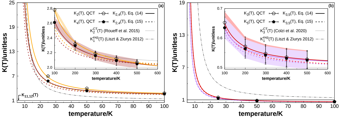
Fig. 4. Equilibrium constants and associated error bars for the reactions (a) ^{13}\text{C}(^3\text{P}) + ^{12}\text{C}_2(X^1\Sigma_g^+) \rightleftharpoons ^{13}\text{C}^{12}\text{C}(X^1\Sigma_g^+) + ^{12}\text{C}(^3\text{P}) (Eq. (2), K_2 = k_2/k_{-2} ) and ^{13}\text{C}(^3\text{P}) + ^{12}\text{C}_2(a^3\Pi_u) \rightleftharpoons ^{13}\text{C}^{12}\text{C}(a^3\Pi_u) + ^{12}\text{C}(^3\text{P}) (Eq. (4), K_4 = k_4/k_{-4} ); (b) ^{13}\text{C}(^3\text{P}) + ^{13}\text{C}^{12}\text{C}(X^1\Sigma_g^+) \rightleftharpoons ^{13}\text{C}_2(X^1\Sigma_g^+) + ^{12}\text{C}(^3\text{P}) (Eq. (3), K_3 = k_3/k_{-3} ) and ^{13}\text{C}(^3\text{P}) + ^{13}\text{C}^{12}\text{C}(a^3\Pi_u) \rightleftharpoons ^{13}\text{C}_2(a^3\Pi_u) + ^{12}\text{C}(^3\text{P}) (Eq. (5), K_5 = k_5/k_{-5} ) at temperatures up to 600 K. Points and solid thick lines are obtained from Eq. (14) using the QCT thermally averaged rates and their analytic forms in Eq. (13), respectively, while dashed thick lines represent theoretical estimates based on statistical mechanics (Eq. (15)). Also shown are the corresponding values predicted via capture theory (Roueff et al. 2015; Colzi et al. 2020) for reactions (2) and (3) and experimental data (exp) for ^{13}\text{C}^+ + ^{12}\text{CO} \rightleftharpoons ^{13}\text{CO} + ^{12}\text{C}^+ (Eq. (1), K_1 = k_1/k_{-1} ) as taken from Liszt & Ziurys (2012). For clarity, the K values for the thermoneutral reactions (11) and (12) are also indicated. High-temperature limits are represented by gray solid lines.
