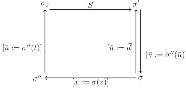
Fig. 3. Construction of a computation of P(\bar{i}) .
