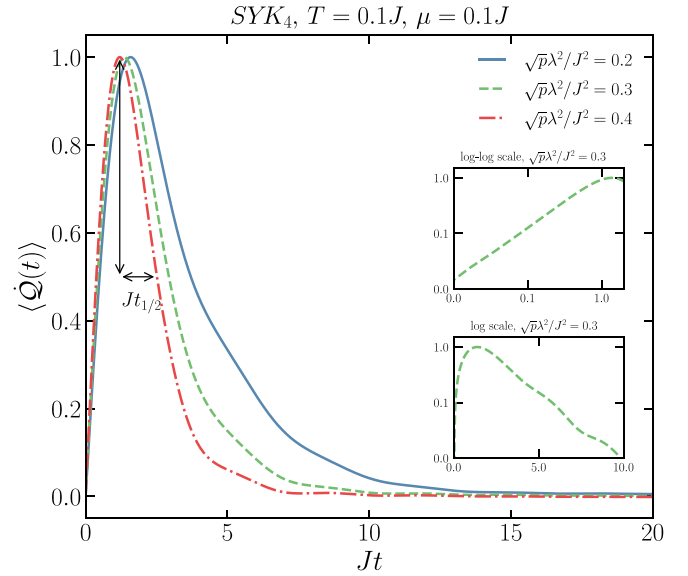
FIG. 4. Tunneling current as a function of time normalized on its maximum value. The insets show time dependence of the current in log-log and log scales for \sqrt{p}\lambda^2/J^2 = 0.3 . The log-log plot reveals the initial power-law increase of the tunneling current, while the log plot is consistent with the exponential decay. We illustrate the current's half-life t_{1/2} for \sqrt{p}\lambda^2/J^2 = 0.4 .
