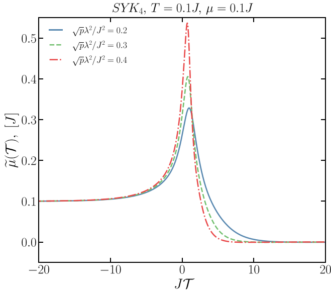
FIG. 2. Effective chemical potential in the SYK quantum dot coupled to a large reservoir with T_{\text{res}} = 0 and \mu_{\text{res}} = 0 .
