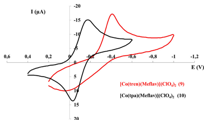
Fig. 6. Cyclic voltammetry curves registered for [\text{Co}(\text{tren})(\text{MeFlav})](\text{ClO}_4)_2 ( 9 ) and [\text{Co}(\text{tpa})(\text{MeFlav})](\text{ClO}_4)_2 ( 10 ) in \text{H}_2\text{O}:\text{MeOH} = 1:1 , referenced to Ag/AgCl electrode at a potential sweep rate of 200 \text{ mVs}^{-1} , I = 0.20 \text{ M KNO}_3 and c = 1.0 \text{ mM} .
