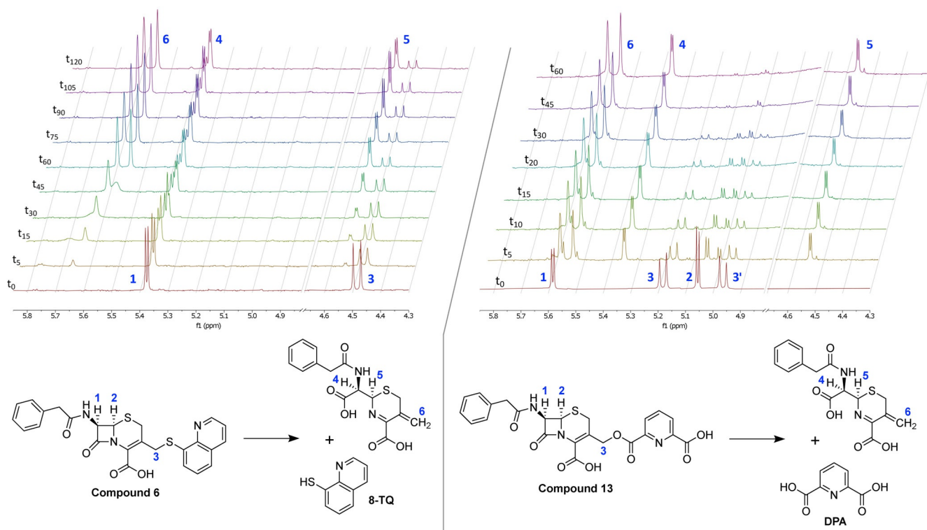
Figure 2. ^1\text{H} NMR spectra showing the MBL-mediated hydrolysis of compounds 6 (left panel) and 13 (right panel) over time. For both compounds, the hydrolysis by NDM-1 leads to the clean formation of the vinylic product and release of the zinc binding compound. For clarity, the region of the spectra including the suppressed water signal has been removed. In the case of compound 6 , the signals for the proton at position 2 and one of the protons at position 3 overlap with the suppressed water signal and are therefore not visible (full NMR spectra provided in the Supporting Information).
