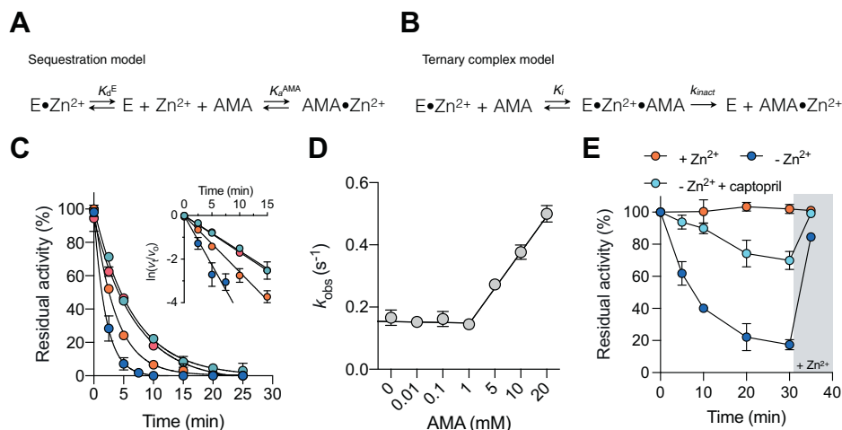
Figure 3. Kinetic analyses reveal a dual mechanism of NDM-1 inhibition in vitro . A, minimal kinetic scheme for inhibition by sequestration, where E = MBL, K_d^E = [E][Zn^{2+}]/[E \cdot Zn^{2+}] , and K_d^{AMA} = [AMA \cdot Zn^{2+}]/[AMA][Zn^{2+}] . B, minimal kinetic scheme for inhibition by ternary complex formation, where E = MBL, K_i = [E \cdot Zn^{2+}][AMA]/[E \cdot Zn^{2+} \cdot AMA] and k_{inact} is the rate constant for the breakdown of the ternary complex to E and AMA \cdot Zn^{2+} . C, representative time courses for NDM-1 inhibition by AMA. Rates of inhibition were measured at fixed time intervals with 2 (blue), 5 (orange), 1 (magenta), and 0.1 mM (cyan) AMA. Inset, natural log transformation of the inhibition plot, where v_t/v_o = residual activity. D, observed rate constants ( k_{obs} ) determined from the previous panel relative to AMA concentration. E, spontaneous inactivation of NDM-1 in metal-free buffer (blue), metal-free buffer containing L-captopril (100 \mu M; cyan), and ZnSO_4 (10 \mu M) supplemented buffer (orange). The gray bar denotes the addition of ZnSO_4 to each mixture at t = 35 min. Metal-free buffer was produced by treating 25 mM Hepes–NaOH, 1% (v/v) with Chelex-100 resin. All data are representative of the mean value of two independent replicates, and error bars indicate SD. AMA, aspergillomarasmine A; MBL, metallo- \beta -lactamase; NDM-1, New Delhi MBL-1.
