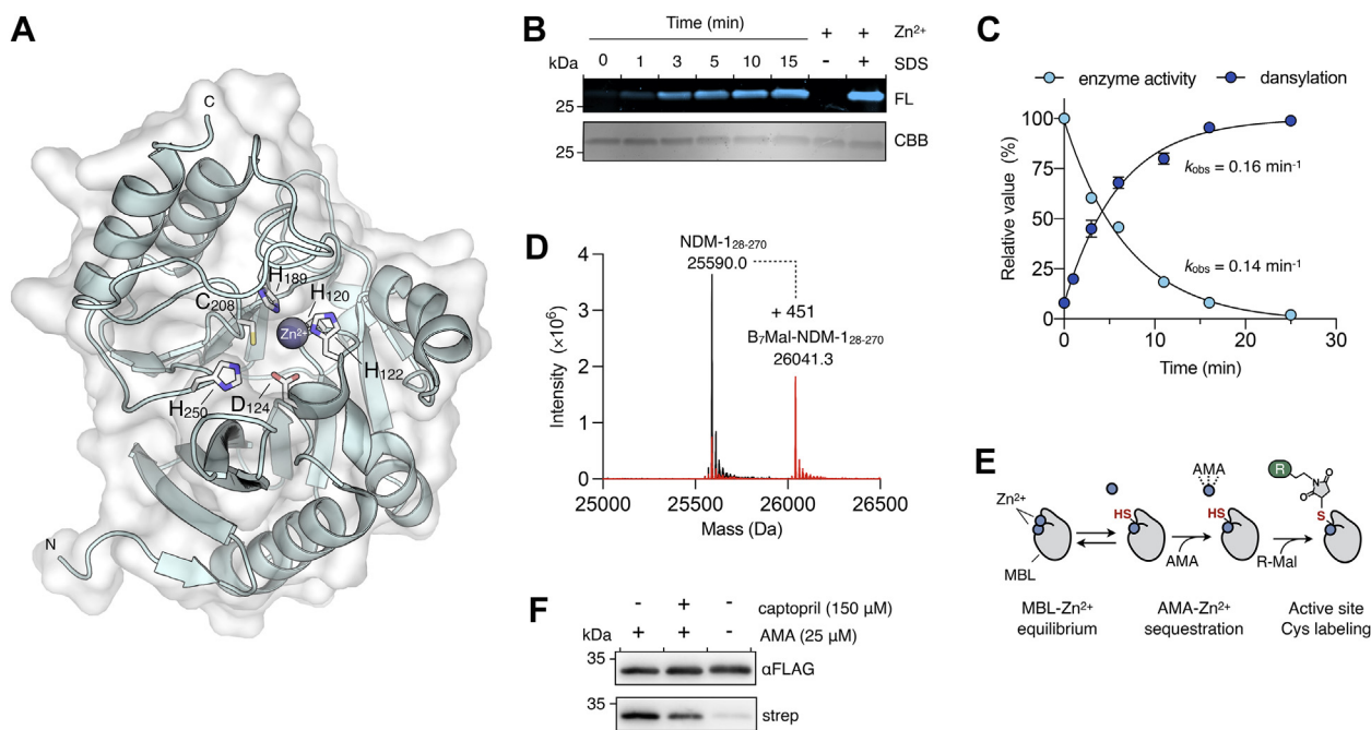
Figure 4. Maleimide probes detect mononuclear MBLs through the action of AMA both in vitro and in live bacteria. A , structure of mono-Zn 2+ NDM-1 illustrating the Zn 2+ binding sites (Protein Data Bank ID: 3SFP). The Zn 1 and Zn 2 sites are defined by H 122 , H 120 , and H 189 and D 124 , C 208 , and H 250 , respectively. B , representative in vitro time course of NDM-1 (1 \mu\text{M} ) dansylation in assay buffer (25 mM Hepes–NaOH, 1% [v/v] PEG 4000, 10 \mu\text{M} ZnSO 4 , and pH 7.5) with AMA (0.1 mM) at 37 °C. At the end of the time course, ZnSO 4 (0.11 mM) or ZnSO 4 and SDS (2% w/v) were added to separate aliquots of the reaction. Top , SDS-PAGE analysis with fluorescence detection (FL) shows the increasing labeling of NDM-1 (1 \mu\text{M} ) in the presence of DM (0.5 mM) and AMA (0.1 mM). NDM-1 is not labeled in the presence of ZnSO 4 and entirely labeled when denatured with SDS. Bottom , Coomassie brilliant blue (CBB) staining of total protein. C , quantitative analysis of maleimide labeling (blue) in panel ( B ) relative to enzyme activity loss under the same conditions without DM present (cyan). The data are representative of two replicates, and the error bars represent SD. D , intact protein LC ESI–MS analyses of NDM-1 (1 \mu\text{M} ) treated with B 7 –Mal following incubation (1 h) in buffer either lacking (black trace) or containing (red trace) AMA (0.5 mM). E , schematic diagram of a maleimide-based method to enable detection of mononuclear MBLs. AMA causes protein-bound Zn 2+ to dissociate exposing the side chain of Cys 208 that is involved in metal coordination in class B1 MBLs. A maleimide probe then modifies the Cys 208 allowing for detection through reporter molecules (R = dansyl or biotin). F , in situ BM labeling and immunoprecipitation of NDM-1 FLAG . Escherichia coli –producing NDM-1 FLAG was treated (15 min) with (+) or without (–) AMA (25 \mu\text{M} ) and L-captopril (0.15 mM) for 15 min. Following this, cells were incubated with BM (0.5 mM; 15 min). Biotinylated protein and total NDM-1 were detected with streptavidin–HRP (strep) and anti-FLAG–HRP IgG ( \alpha\text{FLAG} ), respectively. Panel F is representative of two independent experiments. AMA, aspergillomarasmine A; B 7 –Mal, biotin–maleimide; DM, N -[2-(dansylamino)ethyl]maleimide; ESI–MS, electrospray ionization–MS; FL, fluorescence; HRP, horseradish peroxidase; MBL, metallo- \beta -lactamase; NDM-1, New Delhi MBL-1.
