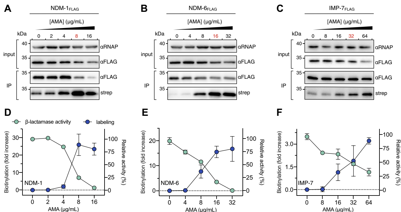
Figure 5. In situ inactivation of MBLs is related to Zn^{2+} binding strength and protein stability. A–C, titration of AMA into cultures of live Escherichia coli producing A, NDM-1 FLAG , B, NDM-6 FLAG , or C, IMP-7 FLAG (15 min) followed by BM labeling (0.5 mM; 15 min). E. coli lysates (input; top panel) were analyzed by immunoblot analysis with anti-FLAG-HRP IgG ( \alpha FLAG) and anti-RNAP IgG ( \alpha RNAP) as a loading control. Immunoprecipitated MBLs (IP; bottom panel) were detected with \alpha FLAG. The blot was reprobed with streptavidin–HRP (strep) to detect the extent of biotinylation of each protein (bottom panel). The AMA concentration colored red represents the amount needed to restore meropenem activity to its breakpoint concentration (2 \mu g \cdot ml ^{-1} ). Blots are representatives of at least two independent experiments. D–F, semiquantitative analysis of biotinylation normalized to the total amount of D, NDM-1, E, NDM-6, and F, IMP-7 (cyan; left axes). Residual \beta -lactamase activity of the cell lysates prior to IP analysis (input) was measured with the substrate nitrocefin (blue; right axes). In all experiments, data are represented by at least two independent biological replicates; data represent mean values \pm SD. AMA, aspergillomarasmine A; HRP, horseradish peroxidase; IMP, imipenemase; IP, immunoprecipitation; MBL, metallo- \beta -lactamase; NDM, New Delhi MBL.
