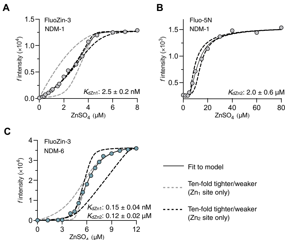
Figure 6. \text{Zn}^{2+} affinities of NDM-1 and NDM-6. A , representative fluorescence of FluoZin-3 (2 \mu\text{M} ) in competition for \text{Zn}^{2+} with NDM-1 (2.4 \mu\text{M} ). B , representative fluorescence of Fluo-5N (1 \mu\text{M} ) in competition for \text{Zn}^{2+} with NDM-1 (5.5 \mu\text{M} ). C , representative fluorescence of FluoZin-3 (2 \mu\text{M} ) in competition for \text{Zn}^{2+} with NDM-6 (4.6 \mu\text{M} ). The solid line represents the fit to a 2:1 \text{Zn}^{2+} :MBL binding model, and dashed lines represent simulations with 10-fold higher and lower K_d values relative to the fitted mean when either the \text{Zn}_1 (gray) or \text{Zn}_2 (black) K_d values are fixed. All assays were performed using 20 mM Hepes–NaOH, 100 mM NaCl, and pH 7.5 in duplicate. MBL, metallo- \beta -lactamase; NDM, New Delhi MBL.
