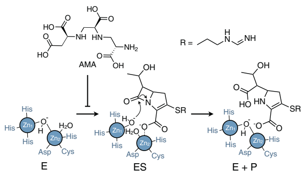
Figure 1. Mechanism for the hydrolysis of imipenem by class B1 MBLs and inhibition by aspergillomarasmine A (AMA). Catalysis by binuclear MBLs involves two \text{Zn}^{2+} cofactors bound in the \text{Zn}_1 and \text{Zn}_2 sites. E, ES, and P represent the free enzyme, enzyme-substrate complex, and product, respectively. AMA interferes MBL catalysis by removing one of the \text{Zn}^{2+} cofactors. MBL, metallo- \beta -lactamase.
