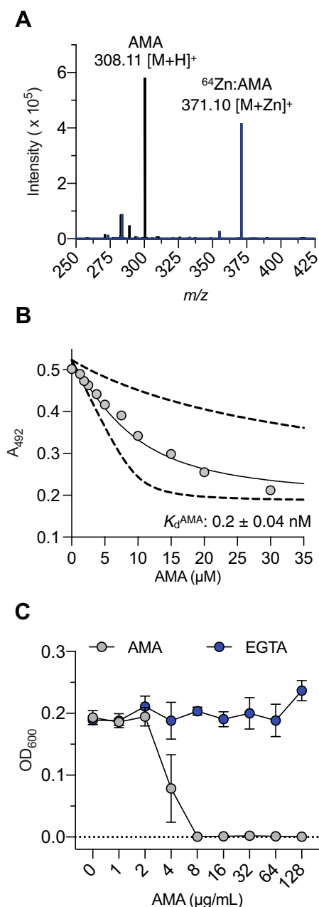
Figure 2. NDM-1 inhibition by AMA is related to both its binding affinity and selectively for Zn 2+ . A , mass spectra of AMA in its free and complexed forms. B , representative ZnPAR 2 (10 μM) absorbance in competition for Zn 2+ with varying concentrations of AMA in 20 mM Hepes, 100 mM NaCl, and pH 7.4. The solid line represents the fit to a 1:1 Zn 2+ :AMA binding model, and dashed lines represent simulations with 10-fold higher and lower K_d values relative to the fitted mean. C , microdilution assay for the reversal of meropenem resistance in Escherichia coli producing NDM-1. AMA (cyan) or EGTA (blue) were titrated into cells in the presence of meropenem (2 μg·mL -1 ) and grown overnight at 37 °C. Absorbance values at 600 nm were recorded after 18 h of incubation. Data represent mean values of two replicates \pm SD. AMA, aspergillomarasmine A; NDM-1, New Delhi MBL-1; PAR, 4-(2-pyridylazo)resorcinol.
