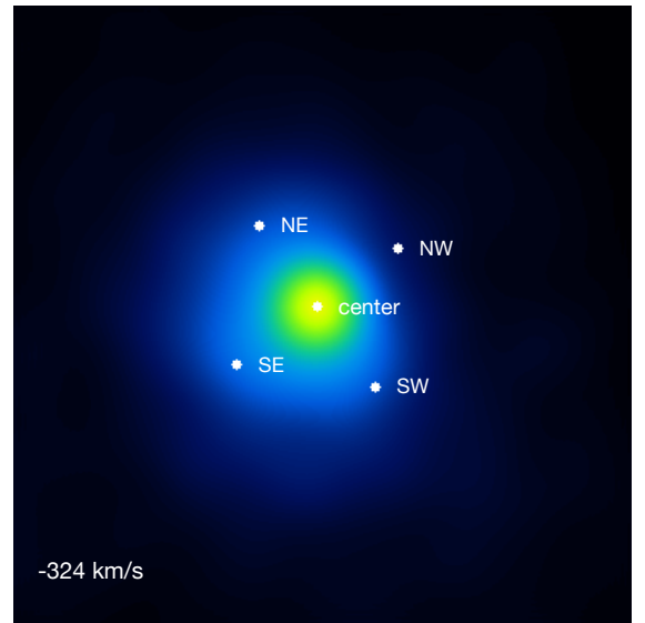
Fig. 3. Extraction of spectra from the 3D data cube in Fig. 1. Top : five spectra extracted at five selected positions from the 11 iso-velocity images in Fig. 1. Bottom : five positions chosen in the images in Fig. 1 to extract five spectra (top) from the 3D data cube of Fig. 1, shown by the dots at center, NE, SE, SW, and NW (same color table as in Fig. 1).
