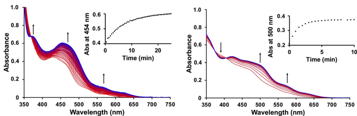
Fig. 3 Evolution of the UV–vis absorption spectra of a solution of [2](PF 6 ) 2 (left) and [3](PF 6 ) 2 (right) upon green light irradiation in water. Conditions: [Ru]=0.074 and 0.061 mM for [2](PF 6 ) 2 and [3](PF 6 ) 2 , respectively, T=37 °C, light source: λ=517 nm,
