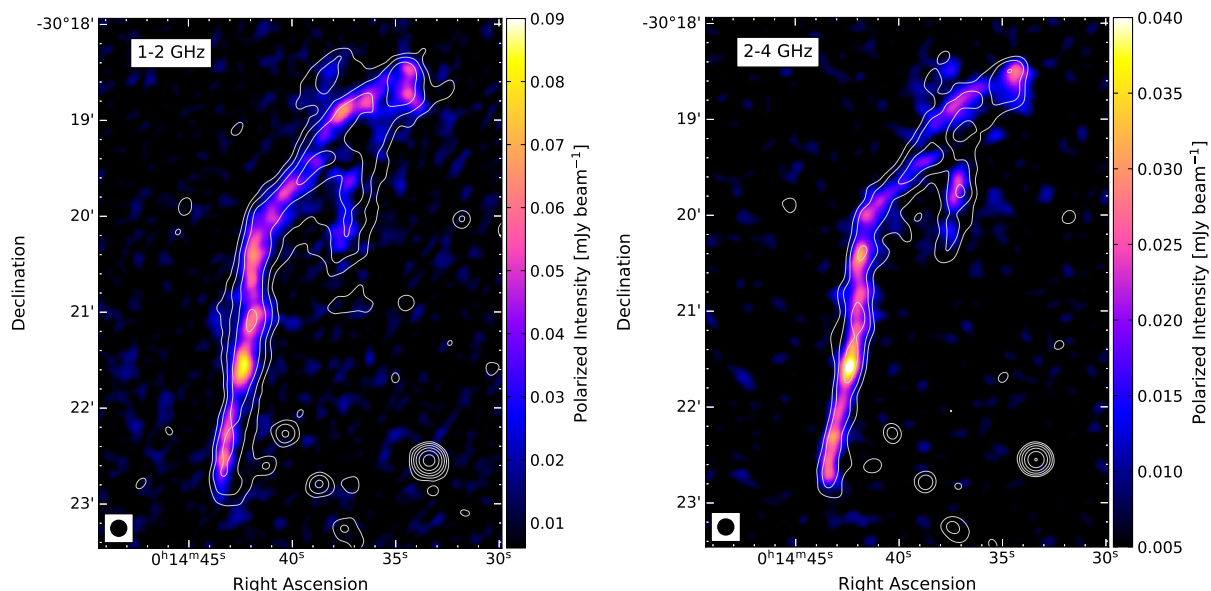
Fig. 16. Polarization intensity images of the main relic R1 at 10'' resolution. The images show that the relic is polarized over its entire length from 1 to 4 GHz. Contour levels are drawn at [1, 2, 4, 8, \dots] \times 5\sigma_{\text{rms}} and are from the Stokes I images. The beam sizes are indicated in the bottom left corner of the each image.
