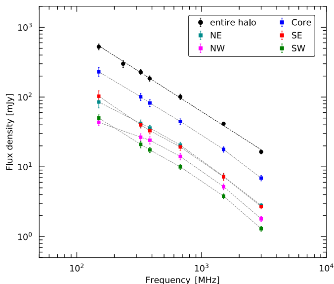
Fig. 6. Left: Integrated radio spectra of the entire halo and its subregions. The radio spectrum of the halo can be described by a power-law (dashed black line) between 150 MHz and 3 GHz. Unlike the halo, its subregions show different spectra also featuring high frequency spectral steepening. Right: The flux density of the entire halo was extracted from the red region, labeled as halo. Green regions were used to extract the flux density from the halo subregions. The blue annuli are used to compute the radio and X-ray surface brightness profiles. These annuli have widths of 15'' , similar to the radio beam size.
