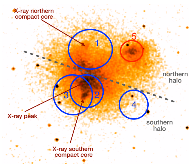
Fig. 1. Chandra 0.5 – 2.0 keV band image, smoothed with a Gaussian full width at half maximum (FWHM) of 2'' . The cluster is rich in X-ray with several substructures near the center. Blue circles mark four subclusters detected in weak/strong lensing analysis (Golovich et al. 2019). A fifth subcluster detected only in X-ray observations is shown with a red circle. The dashed line represents the division between the northern (subclusters 1 and 5) and the southern (subclusters 2, 3, and 4) parts of the halo.
