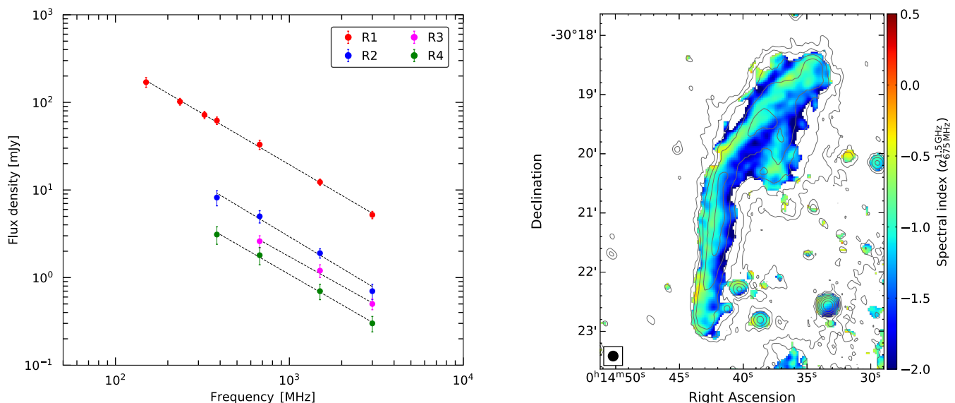
Fig. 7. Left: Integrated radio spectra of relics R1, R2, R3, and R4. Dashed lines are the fitted power-law with indices given in Table 2. Regions used to obtain the integrated flux densities of all four relics are shown in the right panel of Fig. 7. Right: Spectral index map of the main relic R1 between 675 MHz and 1.5 GHz at 10'' resolution, showing a clear spectral index gradient across the entire relic. Contour levels are drawn at [1, 2, 4, 8, \dots] \times 4.0 \sigma_{\text{rms}} , and are from the uGMRT Band 4 image.
