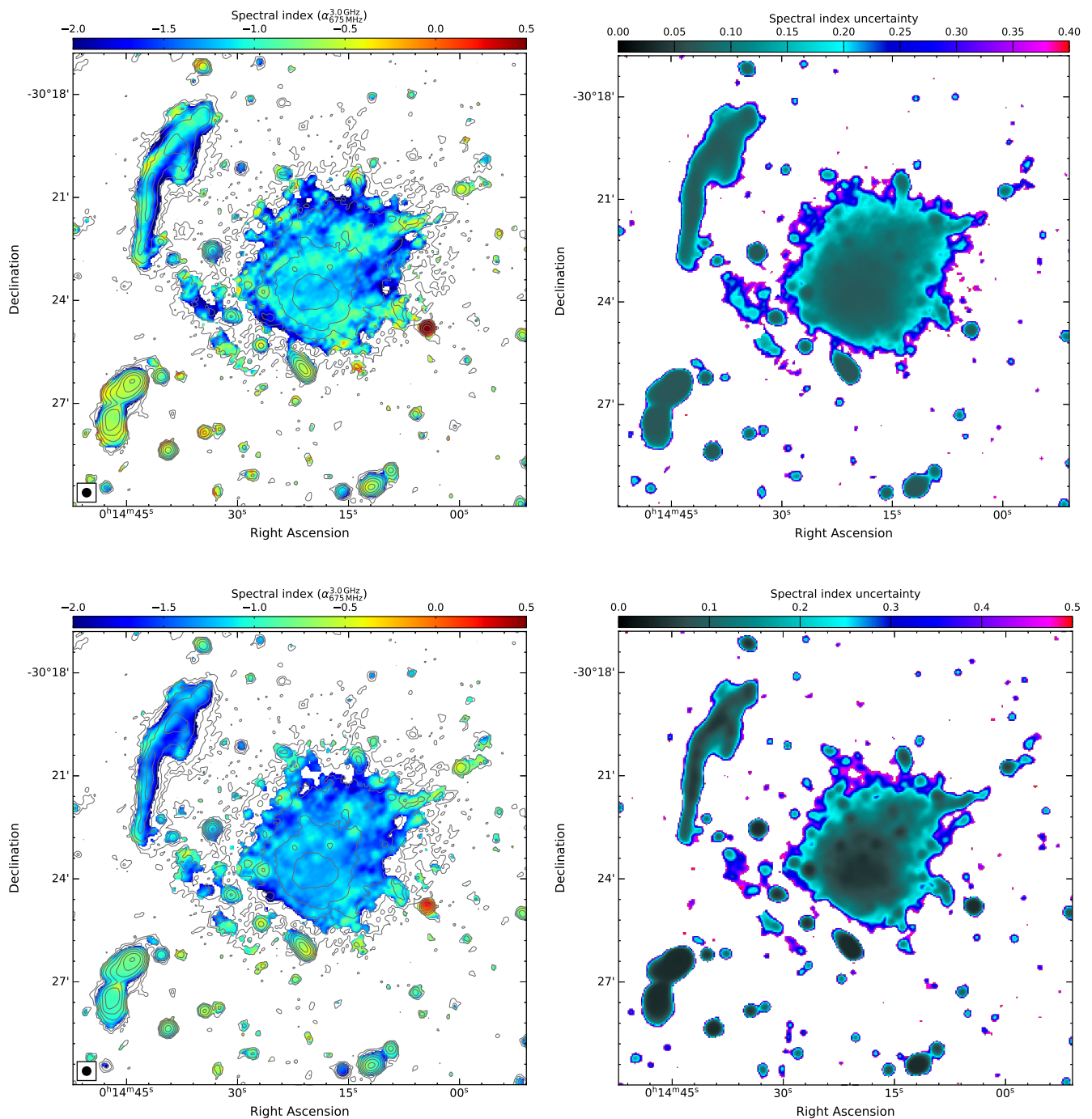
Fig. 9. Left: Spectral index maps of the halo between 675 MHz and 1.5 GHz (top) and 675 MHz and 3.0 GHz (bottom) at 15'' resolution. Contour levels are drawn at [1, 2, 4, 8, \dots] \times 3.5 \sigma_{\text{rms}} , and are from the uGMRT Band 4 image. These maps show the presence of steeper spectral indices in outermost regions of the halo, in particular to the north. Right: Corresponding spectral index uncertainty.
