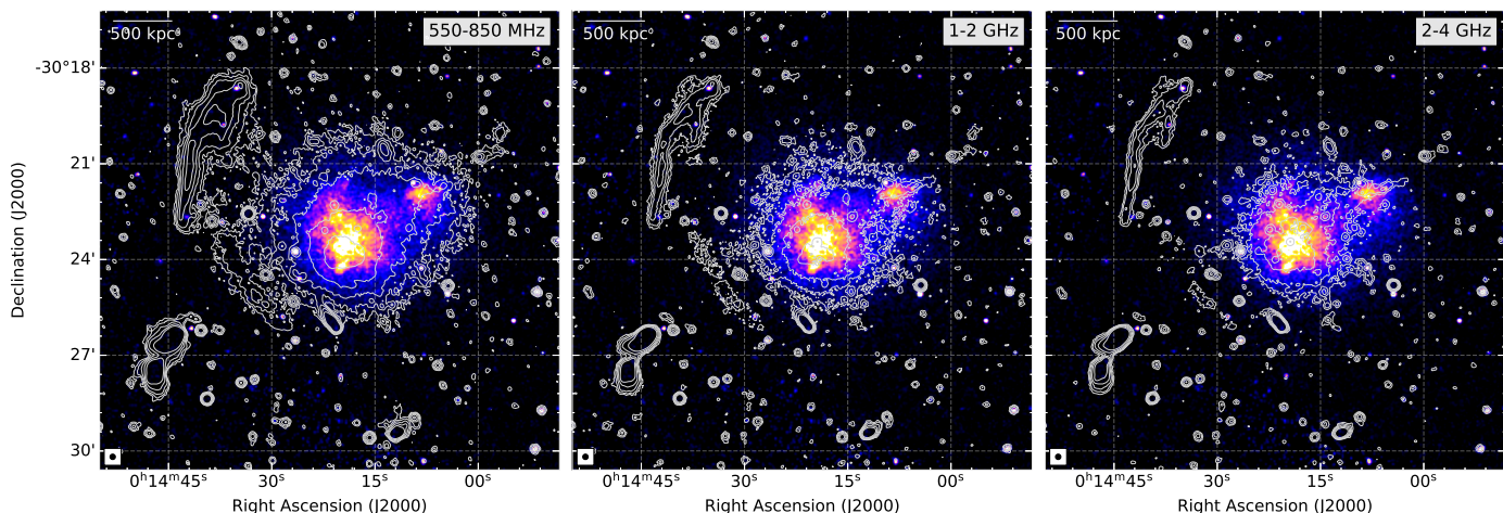
Fig. 5. Chandra (0.5 – 2.0 keV band) X-ray image overlaid with radio contours at 675 MHz, 1.5 GHz, and 3.0 GHz. All radio images are created at a common resolution of 10'' . The radio images are obtained using Briggs weighting with robust=0 . The halo emission is apparently more extended toward low frequencies, in particular to the northeast direction. Contour levels are drawn at [1, 2, 4, 8, \dots] \times 3.5 \sigma_{\text{rms}} , where \sigma_{\text{rms, uGMRT}} = 9 \mu\text{Jy beam}^{-1} , \sigma_{\text{rms, L-band}} = 7.4 \mu\text{Jy beam}^{-1} , and \sigma_{\text{rms, S-band}} = 4.6 \mu\text{Jy beam}^{-1} . In all three images there is no region below -3.5 \sigma_{\text{rms}} . The beam size is indicated in the bottom left corner of the each image.
