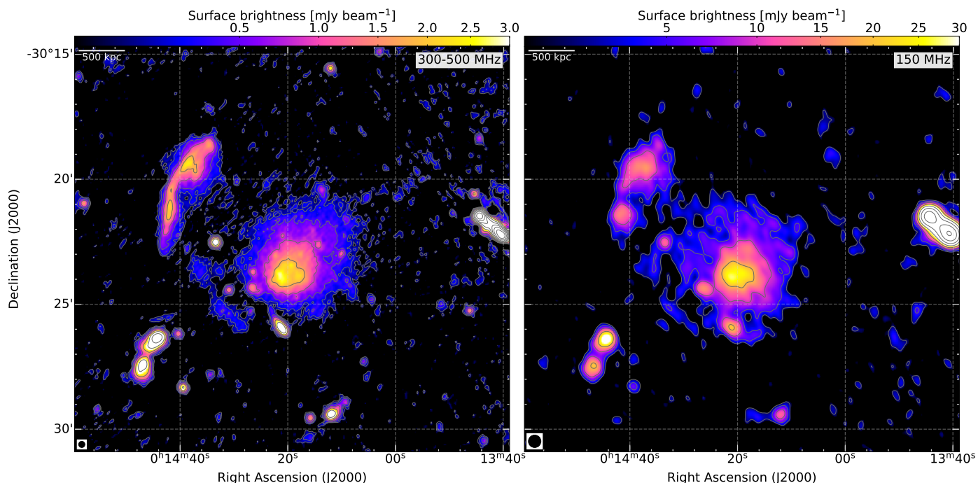
Fig. 4. uGMRT Band 3 (left) image at 15'' resolution and GMRT 150 MHz (right) narrow band image at 30'' resolution. Contour levels are drawn at [1, 2, 4, 8, \dots] \times 3.5 \sigma_{\text{rms}} , where \sigma_{\text{rms}, 385\text{MHz}} = 41 \mu\text{Jy beam}^{-1} and \sigma_{\text{rms}, 150\text{MHz}} = 589 \mu\text{Jy beam}^{-1} . In both images there is no region below -3.5 \sigma_{\text{rms}} . The halo and the main relic R1 are recovered well at both frequencies. Images are created with Briggs weighting with robust=0 . The beam size is indicated in the bottom left corner of the each image.
