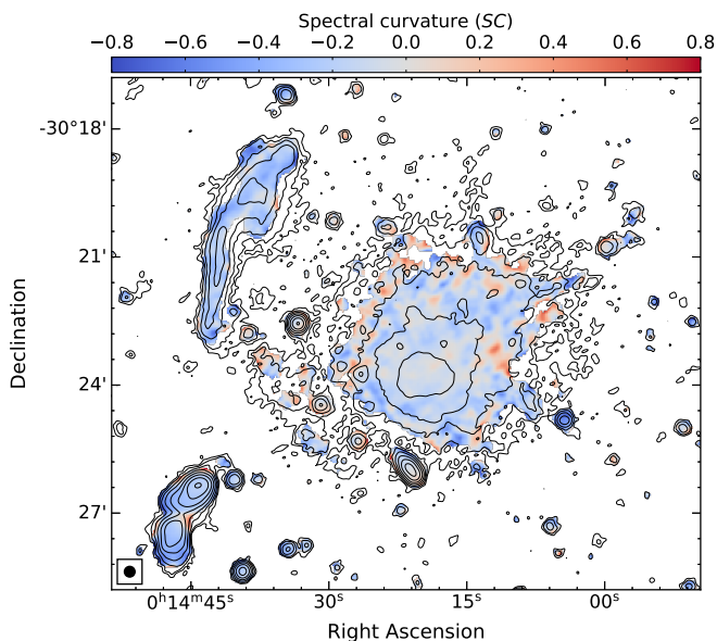
Fig. 11. Left: Three frequency spectral curvature map of the halo at 15'' resolution, created using 675 MHz, 1.5 GHz, and 3 GHz radio maps. The halo shows a hint of spectral curvature. The SC is negative for a convex spectrum. Contour levels are drawn at [1, 2, 4, 8, \dots] \times 3.5\sigma_{\text{rms}} , and are from the uGMRT Band 4 image. Right: Regions where the radio spectral index values were extracted between 675 MHz and 3 GHz. Each box has a width of 15'' corresponding to a physical size of about 67 kpc. The same regions are used to obtain \alpha - I_X correlation in the left panel of Fig. 15.
