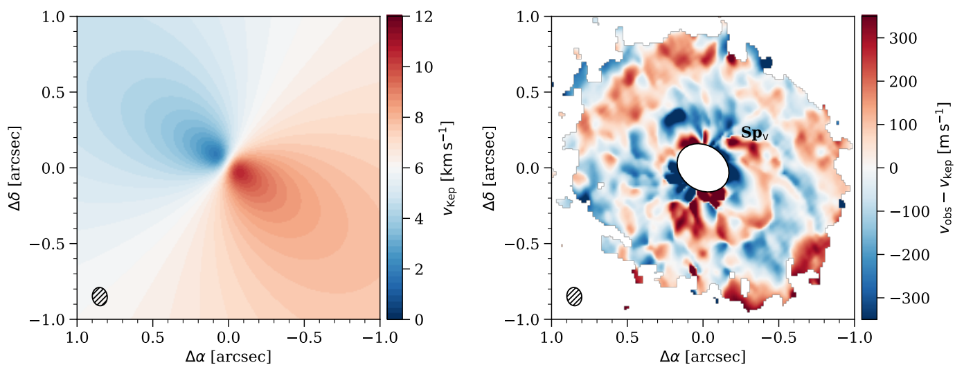
Fig. 6. Best-fit Keplerian rotation model (left panel) and the residuals calculated by subtracting the model from the observed rotation velocity (right panel), shown for ^{12}\text{CO} . The residuals inside of 1.5 the FWHM of the beam are masked out.
