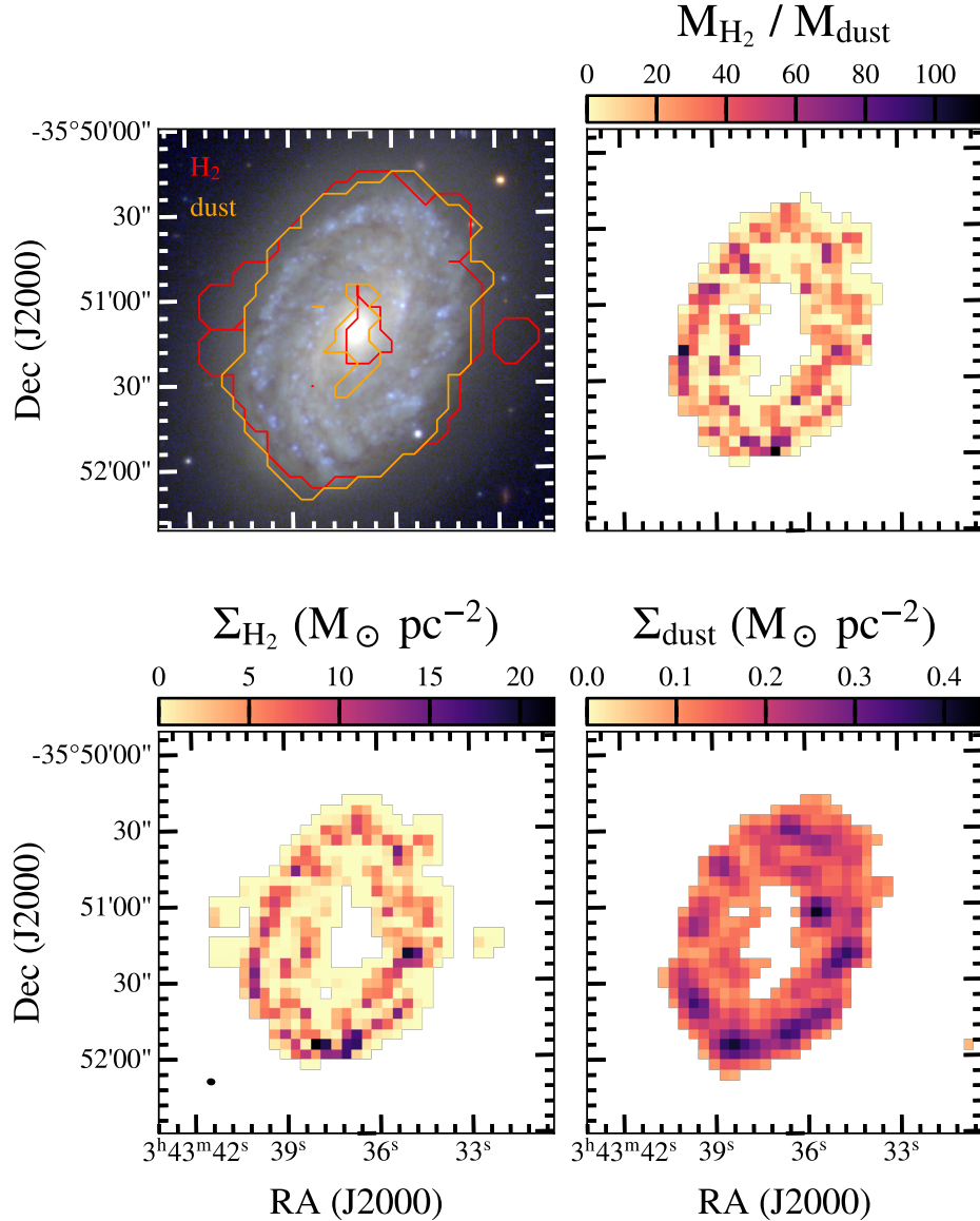
Figure 10. Resolved \text{H}_2 and dust properties in the flocculent spiral NGC1436. Upper left panel: optical ugb -image with the extent of the \text{H}_2 (red) and dust (orange) emission overplotted. Upper right panel: resolved \text{H}_2 -to-dust ratios. Lower-left panel: \text{H}_2 surface density at the resolution of the PACS 100\ \mu\text{m} emission. Bottom-right panel: dust surface density at the PACS 100\ \mu\text{m} resolution from PPMAP. The beam of the CO observations is shown in the bottom-left corner of the bottom-left panel. There is no clear spatial trend in the \text{H}_2 -to-dust ratios in this galaxy.
