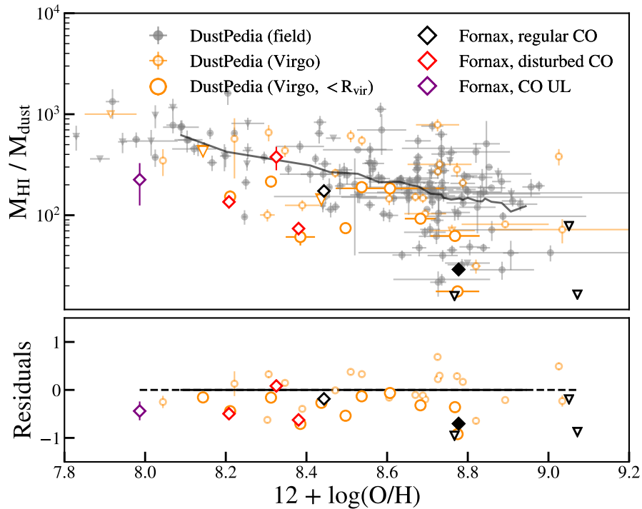
Figure 6. Similar to Figure 2, but showing Hi-to-dust ratios as a function of metallicity. These are systematically lower in Fornax cluster galaxies and Virgo galaxies inside R_{\text{vir}} compared to field galaxies at fixed metallicity.
