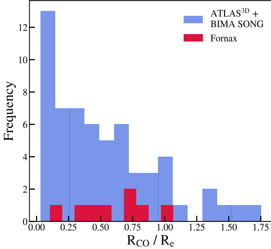
Figure 12. Histogram of R_{CO}/R_e in the Fornax cluster (crimson) compared to a field sample consisting of gas-rich early-type galaxies from ATLAS 3D (Davis et al. 2013) and spiral galaxies from BIMA SONG (Regan et al. 2001), shown in lilac. Fornax cluster galaxies do not have more significantly truncated CO than the field galaxies (a KS test is not able to reject the null-hypothesis that the Fornax and ATLAS 3D /BIMA SONG samples are drawn from the same distribution, D=0.29 , p=0.5 \sim 0.67\sigma ).
