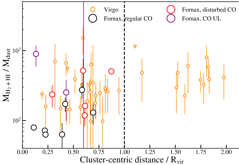
Figure 7. Total gas-to-dust ratios as a function of relative (projected) distance to the cluster centre are shown with colours and markers similar to those in Figure 3. The virial radius is indicated with a black dashed line. No significant gradient in gas-to-dust fractions is observed in any of the clusters, although there is possibly a slight increase in gas-to-dust ratio with cluster-centric radius in the Virgo cluster (a Kendall's Tau test returns a tau statistic of 0.23 and a p-value of 0.04).
