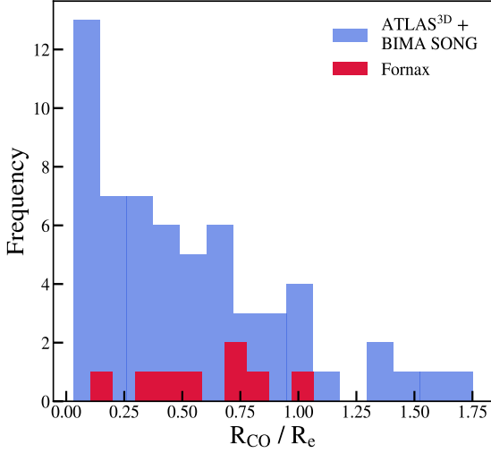
Figure 12. Histogram of R_{\text{CO}}/R_e in the Fornax cluster (crimson) compared to a field sample consisting of gas-rich early-type galaxies from ATLAS 3D (Davis et al. 2013) and spiral galaxies from BIMA SONG (Regan et al. 2001), shown in lilac. Fornax cluster galaxies do not have more significantly truncated CO than the field galaxies (a KS test is not able to reject the null-hypothesis that the Fornax and ATLAS 3D /BIMA SONG samples are drawn from the same distribution, D=0.29 , p=0.5 \sim 0.67\sigma ).
