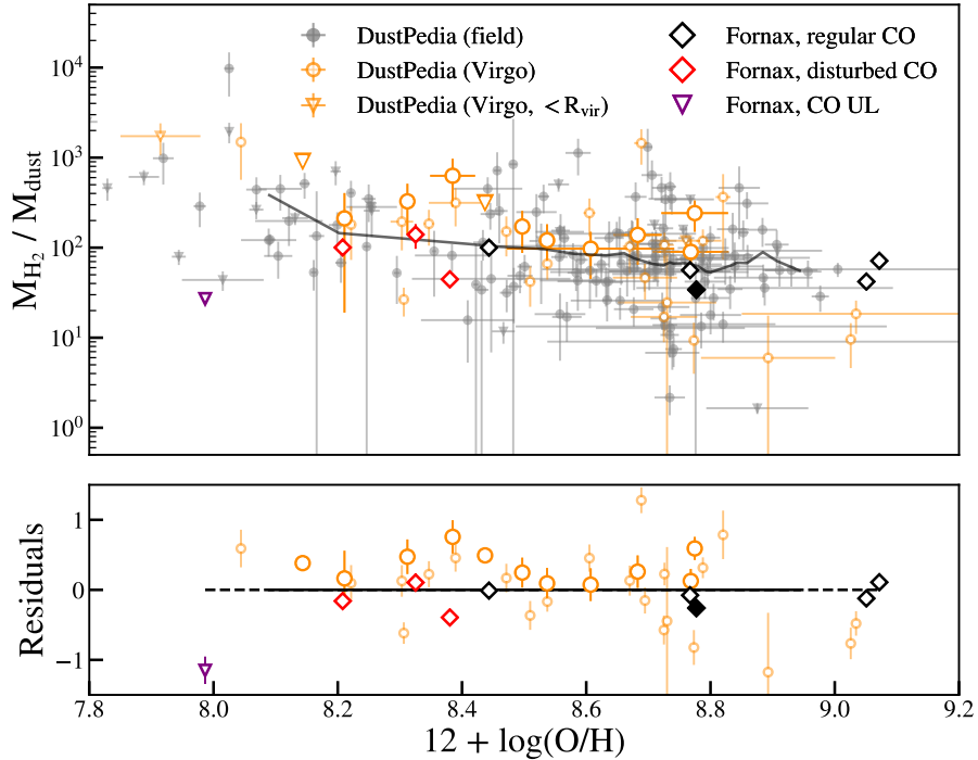
Figure 4. Similar to Figure 2, but showing molecular gas-to-dust ratios as a function of metallicity. Molecular gas-to-dust ratios of Fornax galaxies are systematically lower than those of field galaxies at fixed metallicity, while those inside the virial radius of the Virgo cluster are increased.
