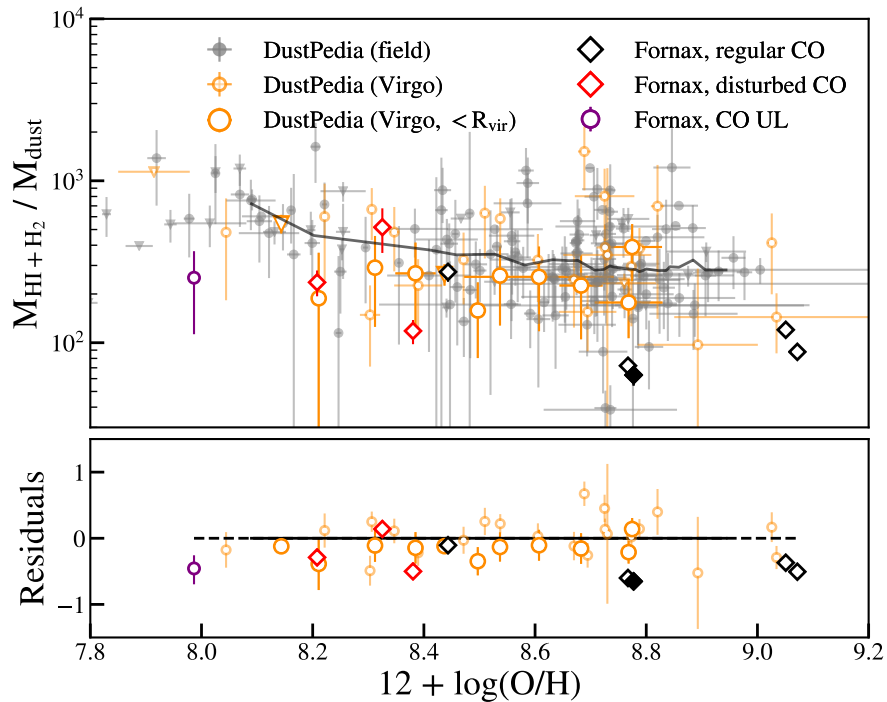
Figure 2. Similar to Figure 1, showing total gas-to-dust ratios as a function of metallicity for a sub-sample of Fornax galaxies for which MUSE data is available from F3D (see Table 1). Fornax cluster galaxies and Virgo galaxies inside R_{\text{vir}} have systematically lower gas-to-dust ratios than field samples.
