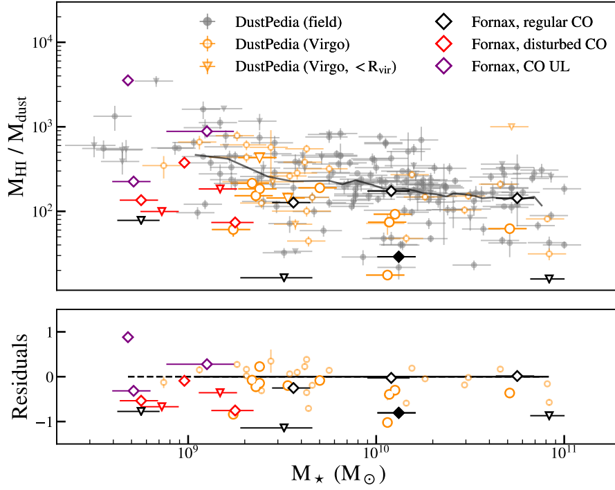
Figure 5. Similar to Figure 1, but showing H I-to-dust ratios as a function of stellar mass. Fornax galaxies and Virgo galaxies inside the virial radius have systematically lower H I-to-dust ratios than galaxies in the field at fixed stellar mass. A possible decrease is also seen in Virgo galaxies between 1 and 2 R_{\text{vir}} .
