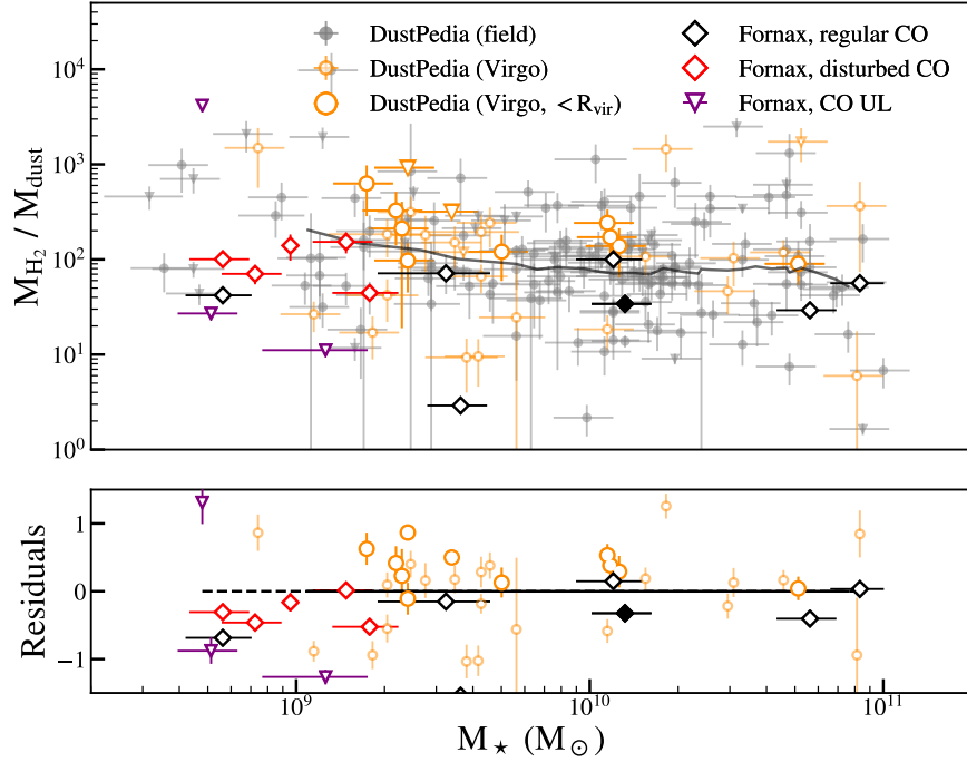
Figure 3. Similar to Figure 1, but showing molecular gas-to-dust ratios plotted as a function of stellar mass. Fornax cluster galaxies have systematically lower molecular gas-to-dust ratios than field galaxies, whereas Virgo galaxies inside R_{\text{vir}} show increased \text{H}_2 -to-dust ratios.
