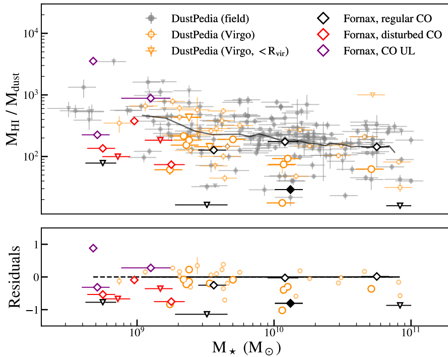
Figure 5. Similar to Figure 1, but showing Hi-to-dust ratios as a function of stellar mass. Fornax galaxies and Virgo galaxies inside the virial radius have systematically lower Hi-to-dust ratios than galaxies in the field at fixed stellar mass. A possible decrease is also seen in Virgo galaxies between 1 and 2 R_{\text{vir}} .
