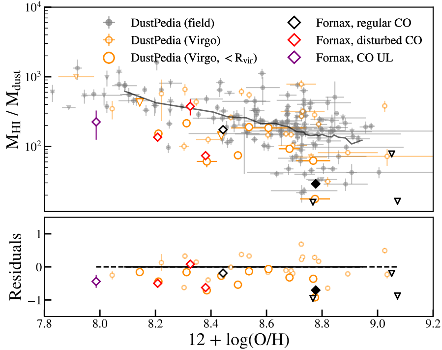
Figure 6. Similar to Figure 2, but showing H I-to-dust ratios as a function of metallicity. These are systematically lower in Fornax cluster galaxies and Virgo galaxies inside R_{\text{vir}} compared to field galaxies at fixed metallicity.
