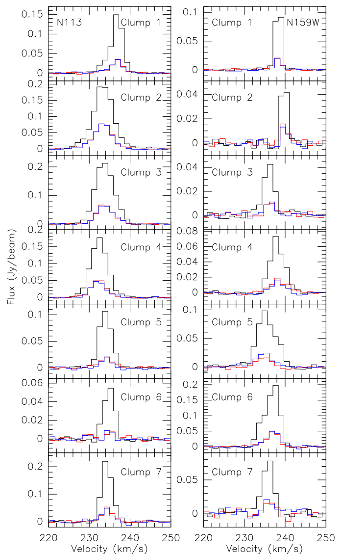
Fig. 2. Spectra towards \text{H}_2\text{CO} clumps in N113 (left panels) and N159W (right panels; see Table 2 and, for the numbering, the left panels of Figs. 3 and 4) taken from the strongest pixel obtained with ALMA. The pixel size is 0''.2 \times 0''.2 . Black: para- \text{H}_2\text{CO} 3_{03}-2_{02} , red: para- \text{H}_2\text{CO} 3_{22}-2_{21} , and blue: para- \text{H}_2\text{CO} 3_{21}-2_{20} . The spectra are not smoothed, i.e. the channel widths are those given in Table 1.
