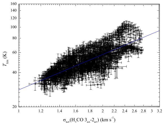
Fig. 7. Non-thermal velocity dispersion ( \sigma_{\text{NT}} ) vs. gas kinetic temperature derived from the para- \text{H}_2\text{CO} line ratio for locations (pixels) with the Mach number M \gtrsim 3.5 in N113. The blue line is the result from an unweighted linear fit, \log T_{\text{kin}} = (1.03 \pm 0.02) \times \log \sigma_{\text{NT}} + (1.45 \pm 0.01) , with a correlation coefficient, R , of 0.78.
