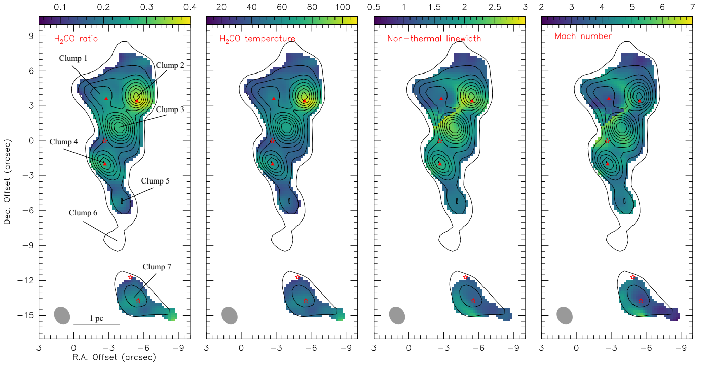
Fig. 3. Left two panels: The averaged velocity-integrated intensity ratio map of para- \text{H}_2\text{CO} 0.5 \times [(3_{22}-2_{21} + 3_{21}-2_{20})/3_{03}-2_{02}] in N113. The kinetic temperatures derived from the para- \text{H}_2\text{CO} (3–2) line ratios (color bar in units of Kelvin). Right two panels: Maps of non-thermal velocity dispersion (color bar in units of \text{km s}^{-1} ) and Mach number. Black contours show levels of integrated intensity of the para- \text{H}_2\text{CO} ( 3_{03}-2_{02} ) line (see Fig. 1). Offsets are relative to our reference position for N113 (see Fig. 1). The pixel size of each image is 0''.2 \times 0''.2 . The beam size of each image is shown in the lower left corner. Stars and triangles show the locations of YSOs (or YSO candidates) and \text{H}_2\text{O} masers (Chen et al. 2010; Ellingsen et al. 2010; Carlson et al. 2012), respectively.
