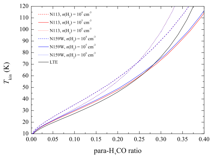
Fig. 5. RADEX non-LTE (red and blue lines) and LTE (black line) modeling of the relation between kinetic temperature and average ratio of para- \text{H}_2\text{CO } 3_{22-2_{21}}/3_{03-2_{02}} and 3_{21-2_{20}}/3_{03-2_{02}} with spatial densities of n(\text{H}_2) = 10^4, 10^5, and 10^6 \text{ cm}^{-3} (dashed, solid, and dotted lines, respectively), an averaged observed linewidth of 4.0 \text{ km s}^{-1} , and column densities of N(\text{para-}\text{H}_2\text{CO}) = 2.7 \times 10^{12} and 3.7 \times 10^{12} \text{ cm}^{-2} for N113 (red lines) and N159W (blue lines) (Tang et al. 2017b), respectively. T_{\text{kin}} -Ratio( \text{H}_2\text{CO} ) relations for N113 and N159W at density 10^4 \text{ cm}^{-3} are nearly the same, which is similar to the situation at 10^6 \text{ cm}^{-3} .
