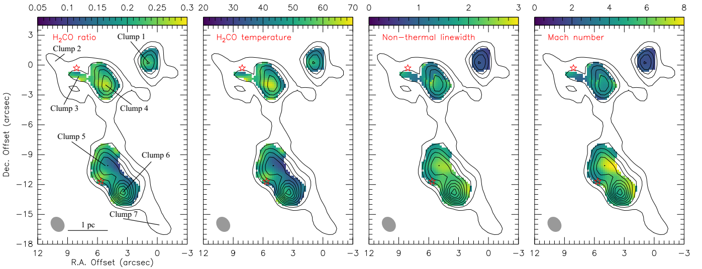
Fig. 4. Same as Fig. 3, but for N159W.
