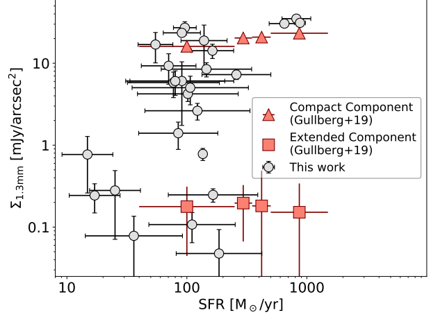
Figure 13. 1.3 mm surface brightness ( \Sigma_{1.3\text{mm}} ) versus intrinsic SFR (assuming a lensing magnification of \mu = 5 ) of resolved SMGs in our sample (grey circles with black edges). Gullberg et al. (2019) reported the existence of both compact (shown as triangles) and extended dust components (squares) of z \sim 3 SMGs through stacking. Assuming typical SED of a SMG at z = 3 , we convert the 870\mu\text{m} surface brightness in Gullberg et al. (2019) to that at 1.3 mm by dividing a factor of 2.7, which is \sim 0.2 \text{ mJy arcsec}^{-2} for extended components. This value matches those of low-surface-brightness SMGs in our sample ( \Sigma_{1.3\text{mm}} \sim 0.1 \text{ mJy arcsec}^{-2} ).
