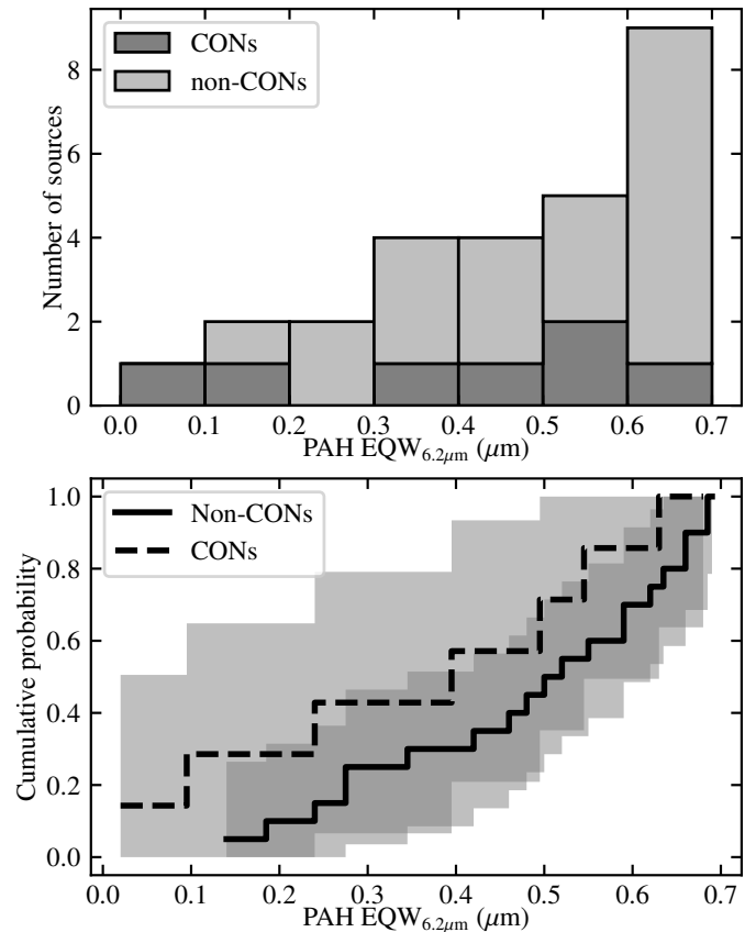
Fig. 6. Distribution of the equivalent width of the 6.2 μm PAH feature in the (U)LIRG sample of CON-quest. Top : stacked histogram of the CON-quest sample with CONs marked using a darker shade. Bottom : empirical distribution functions of the CON and non-CON parts of the sample. The 1-σ confidence intervals are marked with a gray shade.
