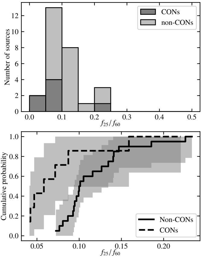
Fig. 4. Distribution of IRAS 25/60 \mu\text{m} ratios in the (U)LIRG sample of CON-quest. Top : stacked histogram of the CON-quest sample with CONs marked using a darker shade. Bottom : empirical distribution functions of the CON and non-CON parts of the sample. The 1- \sigma confidence intervals are marked with a gray shade.
