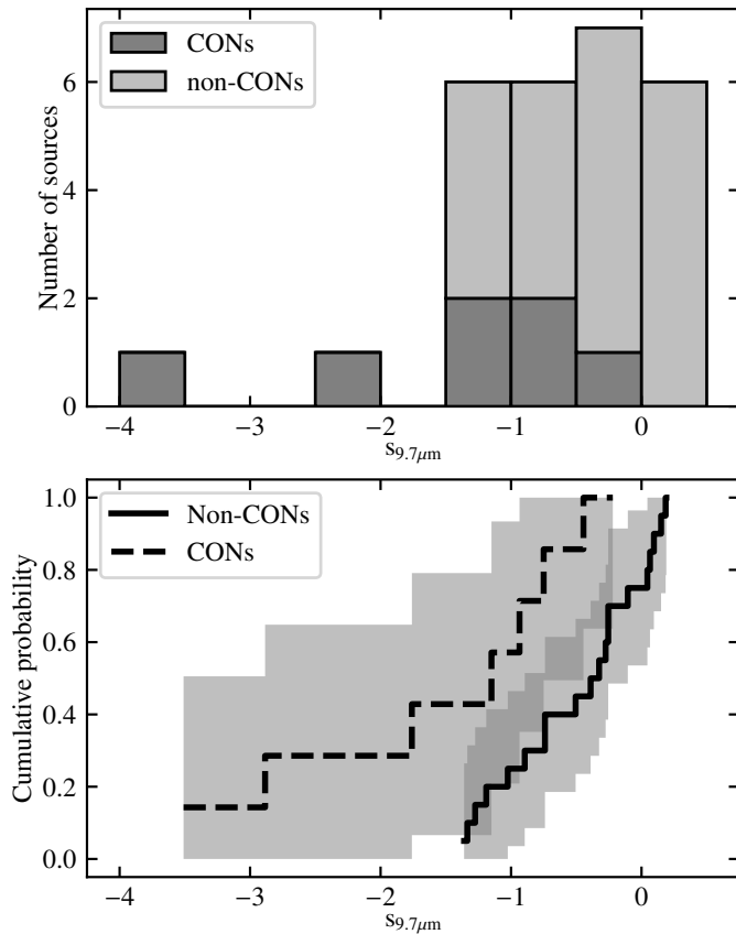
Fig. 5. Distribution of the apparent depth of the 9.7 μm silicate absorption feature in the (U)LIRG sample of CON-quest. Top : stacked histogram of the CON-quest sample with CONs marked using a darker shade. Bottom : empirical distribution functions of the CON and non-CON parts of the sample. The 1-σ confidence intervals are marked with a gray shade.
