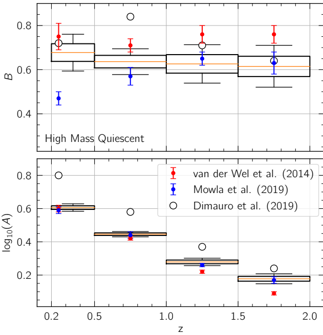
Figure 11. The evolution of the parameters B and \log_{10}(A) with redshift from the single power-law fit shown in Equation 2 for high mass quiescent galaxies (i.e., M_* \geq 10^{10.3} M_\odot ). For the posterior probability distribution in each redshift bin, we indicate the median with an orange line, the 1\sigma confidence level as a box, and the 2\sigma confidence level an error bar. The values shown here are reported in Table 3. We additionally compare these results to other high mass studies, as indicated in the legend. We find that the slope of the best-fit relation for high mass quiescent galaxies remains constant with redshift, consistent with previous works. There is a clear decrease in the intercept – \log_{10}(A) – with redshift. \log_{10}(A) describes the size at a fixed stellar mass of 5 \times 10^{10} M_\odot and its evolution with redshift indicates that quiescent galaxies at higher redshift were more compact, as expected.
