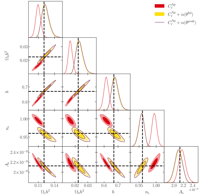
Figure 6. 68% and 95% confidence level contours, as well as one-dimensional marginalised posterior probability distribution functions, obtained by fitting the \Lambda CDM model to the mock data set. The red, filled contours correspond to the analysis where the theoretically predicted approximated spectra C_\ell^{\text{AP}} are used to fit the model to the mock data set. The yellow, filled contours show the results obtained when the debiasing term \alpha(\Theta^{\text{fid}}) is included, and the purple, empty contours correspond to the debiasing term \alpha(\Theta^{\text{peak}}) computed at the estimated maximum likelihood point \Theta^{\text{peak}} .
