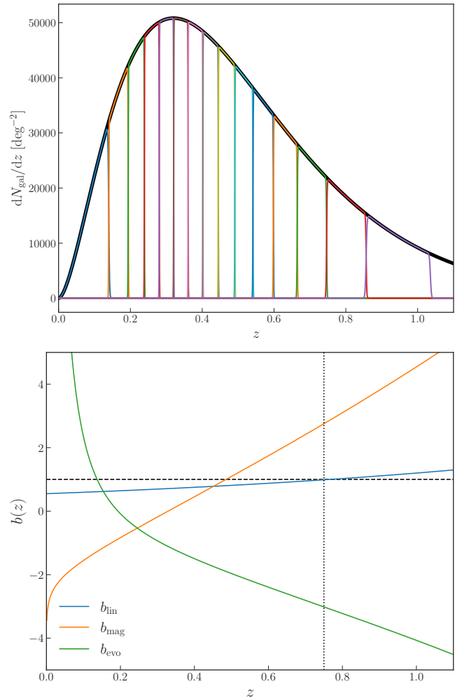
Figure 1. Upper panel: Galaxy distribution as described by Equation 20 (in black) with the limits of the equipopulated redshift bins considered in the present paper (in colour). Lower panel: Trends in redshift for the linear galaxy bias of Equation 21 (blue curve), the magnification bias of Equation 3 (orange curve) and the evolution bias of Equation 5 (green curve). The intersection between the horizontal dashed and vertical dotted black lines shows where the linear galaxy bias crosses unity.
