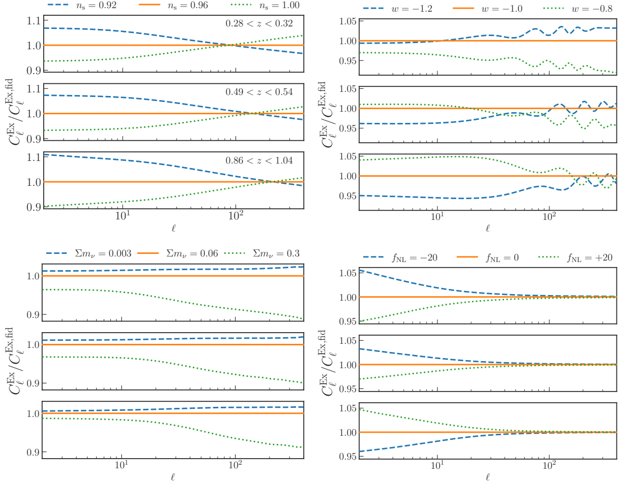
Figure 2. Effects of cosmological parameters on the angular power spectrum of observed galaxy number count fluctuations, C_\ell , on large scales. The four panels depict the effects of: the primordial scalar spectral index n_s in \Lambda CDM (upper left panel); the dark energy equation of state w in w CDM (upper right panel); the sum of the neutrino masses \sum m_\nu in \Lambda CDM+ m_\nu , with values in eV (lower left panel); and the local primordial non-Gaussianity f_{\text{NL}} in \Lambda CDM+ f_{\text{NL}} (lower right panel). All the power spectra are exact, i.e. no approximations are made in their computations, and they are shown in comparison with the fiducial \Lambda CDM spectra with n_s = 0.96 , w = -1 , \sum m_\nu = 0.06 eV and f_{\text{NL}} = 0 . Each panel contains three sets of spectra computed for the three redshift bins 5, 10 and 15, corresponding to low, medium and high redshifts (from top to bottom in each panel). The redshift range of each bin is indicated in the respective plot in the upper left panel.
