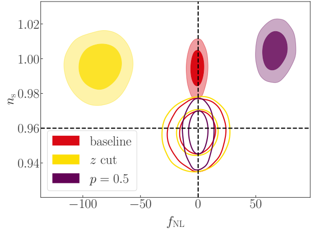
Figure 7. 68% and 95% confidence level contours obtained by fitting the approximated C_\ell^{\text{AP}} spectra, with a free f_{\text{NL}} parameter, to the data set built using the exact C_\ell^{\text{Ex}} spectra (colour-filled contours). The red and yellow contours show the results obtained with the scale-dependent bias of Equation 22, with our baseline settings and with removing the last two redshift bins, respectively. The violet contour shows instead the case where the scale-dependent bias is computed following Equation 23 with p = 0.5 . The empty contours show the results of the analysis when the debiasing term described in subsection 5.1 is included. The black dashed lines show the values of the fiducial cosmological parameters.
