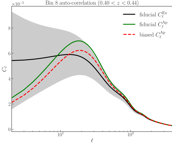
Figure 5. Angular power spectra for the eighth redshift bin auto-correlation in a \Lambda CDM cosmology using the exact C_\ell^{\text{Ex}} (black solid curve) and the approximated C_\ell^{\text{AP}} (green solid curve) obtained assuming the fiducial values for the cosmological parameters. The red dashed curve shows the C_\ell^{\text{AP}} obtained for the biased parameter estimation of Table 3. The grey area shows the errors corresponding to the experimental setup used throughout the paper.
