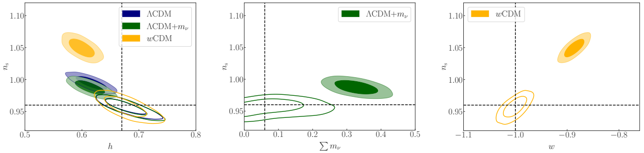
Figure 4. 68% and 95% confidence level contours obtained by fitting the approximated C_\ell^{\text{AP}} spectra to the data set built using the exact C_\ell^{\text{Ex}} spectra (colour-filled contours). The violet contours show the result when a \Lambda CDM model is assumed, while the green and orange contours correspond instead to \Lambda CDM+ m_\nu and w CDM cosmologies, respectively. The empty contours show the results of the analysis when the debiasing term described in subsection 5.1 is included. The black dashed lines show the fiducial values of the cosmological parameters.
