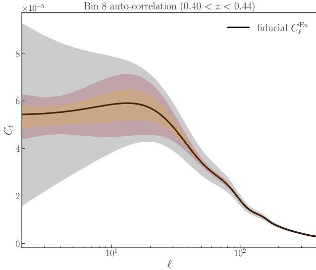
Figure 3. Effect of debiasing when different \Theta_0 points in the parameter space are used to compute the debiasing term \alpha(\Theta^0) . Here \alpha(\Theta^0) is computed at the fiducial set of parameters, \Theta^{\text{fid}} , and at 500 other points in the parameter space, randomly sampled from a Gaussian distribution centred at \Theta^{\text{fid}} with a variance of 10% for each parameter. The black solid curve shows the fiducial C_\ell^{\text{Ex}}(\Theta^{\text{fid}}) spectrum, while the grey band shows the errors corresponding to the experimental setup considered in the paper. For each of the 500 computed \alpha(\Theta^0) , the debiasing term is applied to the C_\ell^{\text{AP}}(\Theta^{\text{fid}}) spectrum. Assuming that the resulting spectra also follow a Gaussian distribution around the C_\ell^{\text{AP}}(\Theta^{\text{fid}}) + \alpha(\Theta^{\text{fid}}) spectra, the orange and red areas show the 1\sigma and 2\sigma uncertainty regions, respectively. Here the auto-correlation in the eighth bin is shown as a typical example.
