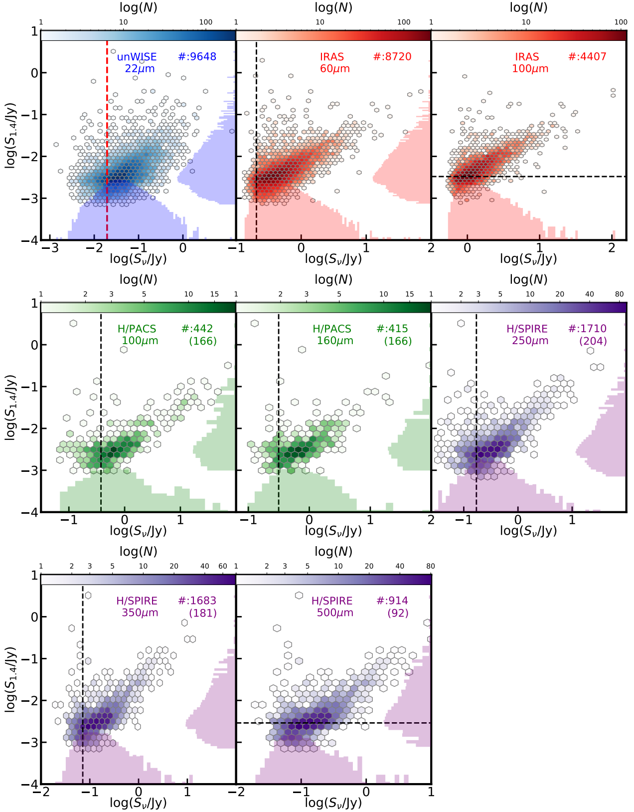
Figure 5. Radio versus infrared fluxes from unWISE ( 22\,\mu\text{m} ), IRAS ( 60 and 100\,\mu\text{m} ) and Herschel ( 100 , 160 , 250 , 350 and 500\,\mu\text{m} ) in our joint sample (i.e. before flux cuts and removing AGN and ambiguous galaxies). IR and radio flux density distributions are shown on the sides. The dashed lines in each panel illustrate the flux density cuts we applied in order to select our radio-IR depth-matched samples for measuring monochromatic IRRC properties, as described in Sect. 3.3. Table 4 contains the corresponding flux density values. We note that only the \sim 19.5\,\text{mJy} flux selection at 22\,\mu\text{m} was used for the depth-matched sample for investigating the total IRRC. In the upper right corner of each panel we display the number of sources with both radio and IR-detections at a given wavelength. For Herschel bands, values in brackets denote the size of the subset of galaxies with fluxes from the H-ATLAS catalog.
