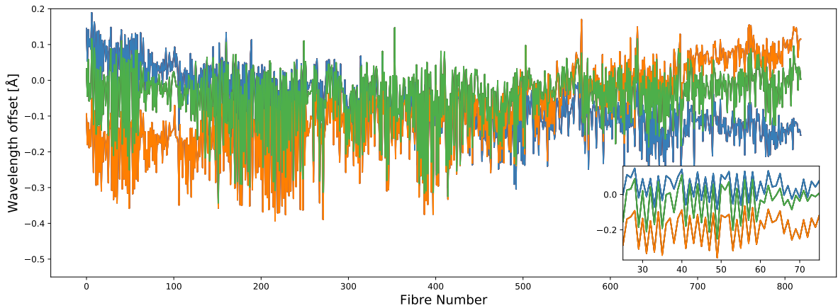
Figure 6. The measured wavelength offset with respect to a high-resolution solar spectrum in \text{\AA} as a function of fibre number for three twilight sky observations (indicated by the three different colours). The inset shows a zoom in over a small range of fibres to better illustrate the fibre-to-fibre variation.
