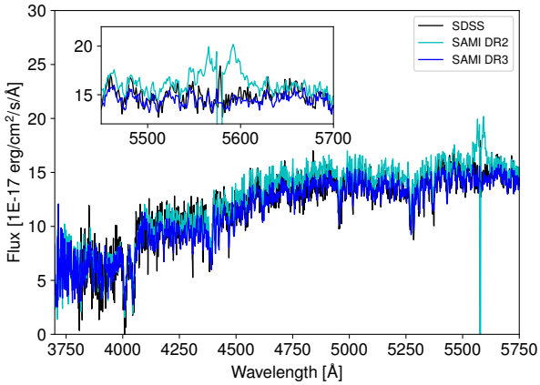
Figure 9. A comparison of SAMI blue arm spectra (3 arcsec diameter aperture) from DR2 (cyan) and DR3 (blue) for object 289198 that showed particularly strong residual scattered light around the 5577 Å night-sky line in DR2. We also compare the spectra to an SDSS spectrum of the same object (black). Inset is a close-up of the region around the 5577 Å line.
