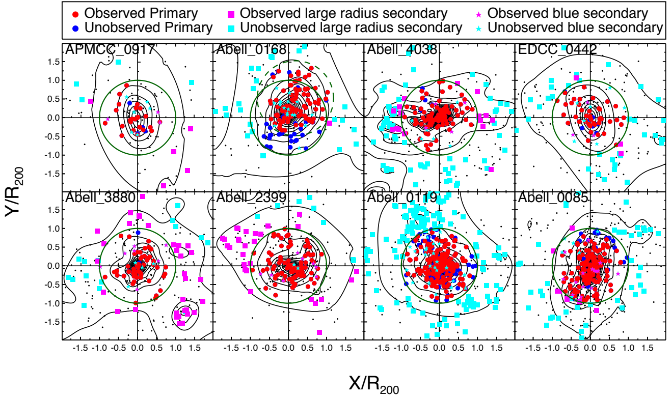
Figure 2. The distribution of SAMI targets in the cluster regions. The small gray points show cluster members selected from the SAMI Cluster Redshift Survey, which are used to define the galaxy surface density isopleths shown as black contours. Large circles show observed (red) and unobserved (blue) primary targets. The magenta (cyan) points show observed (unobserved) secondary targets. These secondary targets are indicated by either squares (for galaxies at large radius) or stars (for blue colour-selected galaxies). The green circles show R_{200} . For Abell 168, the dashed green circle shows the off-centre region used to include targets within R_{200} of the northern BCG, which was used to define the cluster centre during the early parts of the survey.
