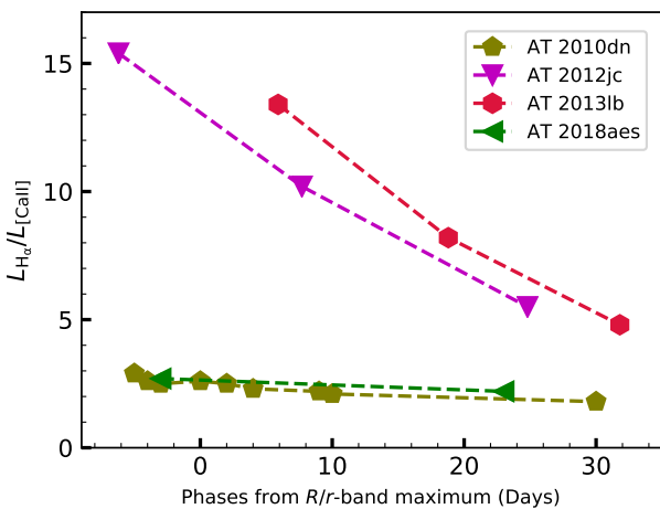
Fig. 14: Ratio of H \alpha to [Ca II] (total profiles at \lambda \approx 7300 Å) luminosities until phase \sim 30 d.
