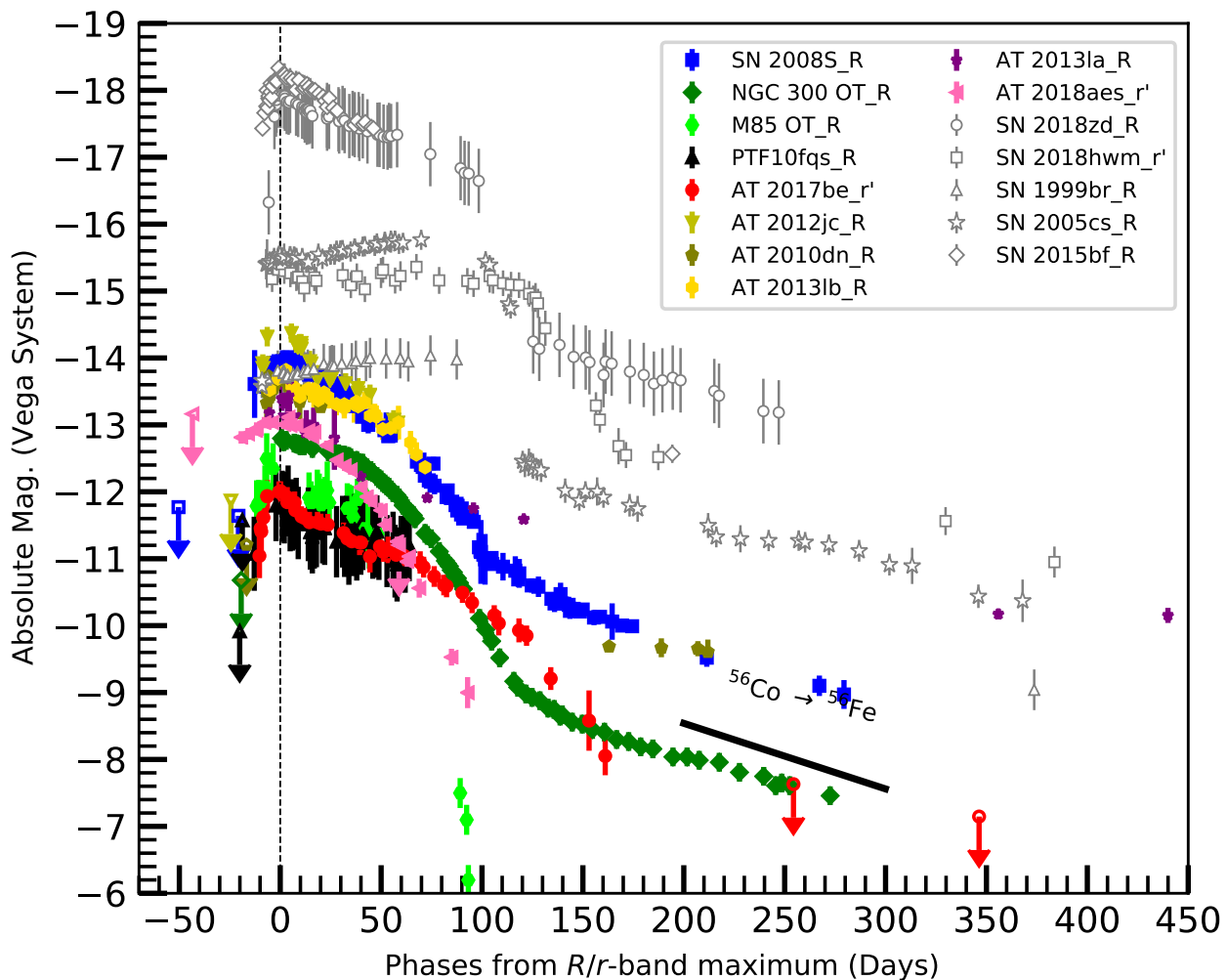
Fig. 4: Comparison of the R/r -band absolute light curves of ILRTs and SN 2018zd, SN 2018hwm, SN 1999br, and SN 2005cs. Reddenings and distance moduli of the comparison objects are taken from their respective papers (also see Table B.1 in Appendix B). The dashed vertical line indicates the time of r -band maximum light. Upper limits are marked by empty symbols with down arrows.
