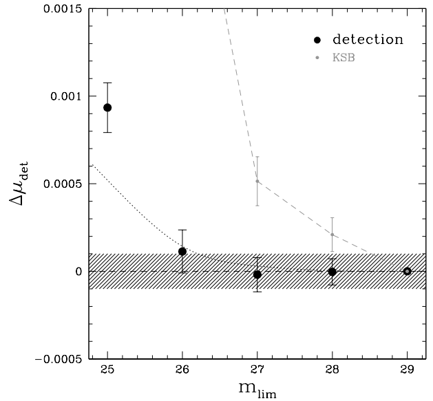
Fig. 9. Change in multiplicative detection bias \Delta\mu_{\text{det}} (with respect to \mu(m_{\text{lim}} = 29) ) for galaxies with 20 < m_{\text{AUTO}} < 24.5 as a function of m_{\text{lim}} , the magnitude of the faintest galaxies that are included in the simulation (black points). The dotted line shows the change in bias if we select galaxies based on their input magnitude ( 20 < m_{\text{input}} < 24.5 ). The change in multiplicative bias for the KSB algorithm is indicated by the light grey points. The hatched region indicates a tolerance of 10^{-4} .
