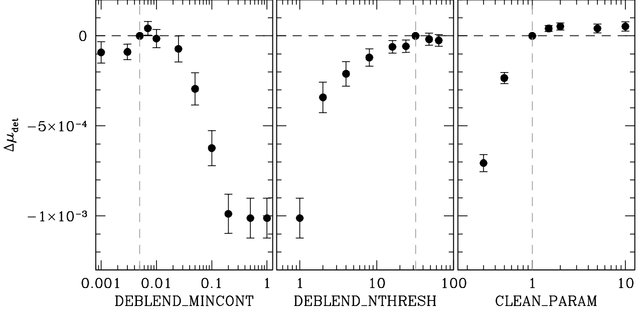
Fig. A.1. Change in multiplicative shear bias \Delta\mu as a function of the SECTRATOR parameters that affect the deblending of objects. The vertical grey dashed line indicates the baseline value (also see Table 1). These default values result in detection biases that are close to optimal.
