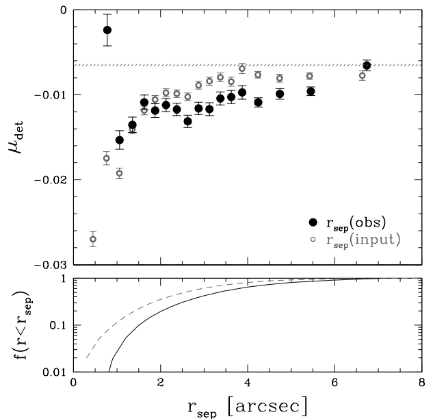
Fig. 3. Top panel: Detection bias for galaxies with 20 < m_{\text{AUTO}} < 24.5 as a function of r_{\text{sep}} , the distance to the nearest object detected by SEXTRACTOR (black points). The open grey points show the detection bias as a function of the nearest neighbour in the input catalogue brighter than m_{\text{input}} = 26 (grey open points). For reference, the hatched region indicates the detection bias for the grid-based simulations; Bottom panel: The fraction of galaxies that have a neighbour within a distance < r_{\text{sep}} in the input catalogue (grey dashed line) or detection catalogue (black line). For small separations many of the true blends are not recognised as such.
