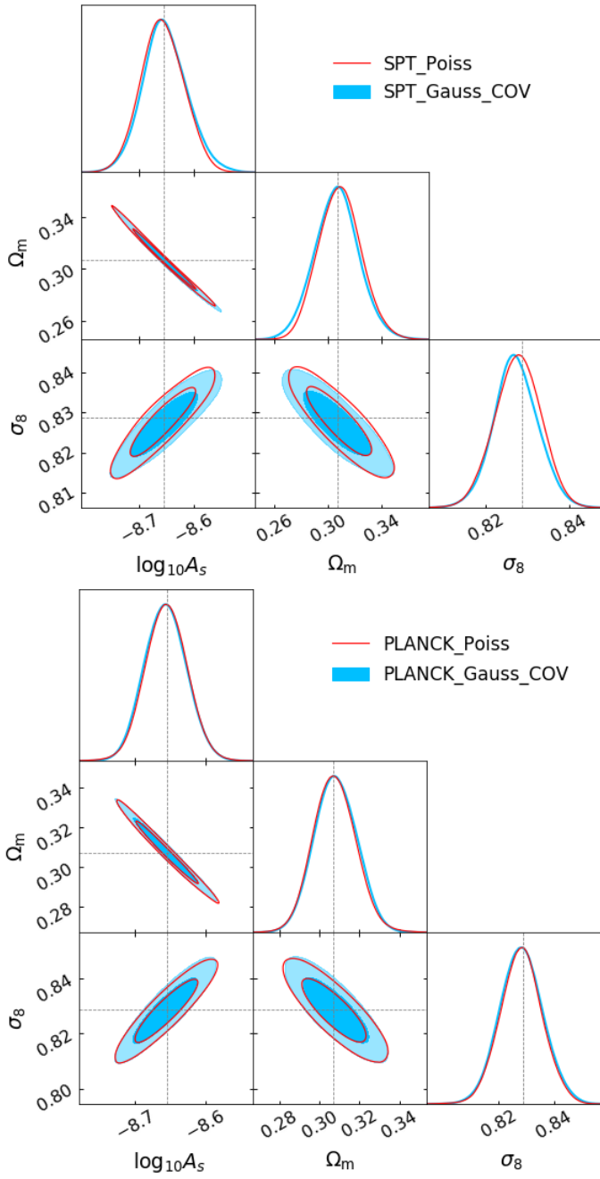
Fig. B.2. Contour plots at 68 and 95 per cent of confidence level for the Poissonian (red) and Gaussian (blue) likelihood for the SPT-like ( top ) and Planck -like ( bottom ) samples. The grey dotted lines represent the input values of parameters.
