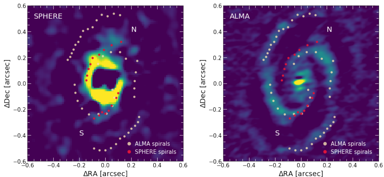
Fig. 6: Left : SPHERE Q_\phi image as described in Fig. 2 but with a Gaussian kernel of size 0.2 \times \text{FWHM} with the spiral arms retrieved from both the ALMA and this image overlotted. Right : ALMA continuum image generated as described in the Appendix C, with the overlotted spiral arms retrieved from both the SPHERE Q_\phi and this image. The “N” and “S” indicate the northern and southern spirals, respectively.
