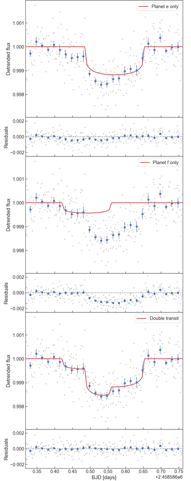
Fig. 13. Same as Figure 12, but considering the five-planet fit. The top and middle panels show the transits of HD 108236 e and HD 108236 f separately, while the bottom panel shows the results obtained with the combined model. The RMS of the binned residuals over the transit window is 137 ppm, which is lower than 168 ppm retrieved in the four-planet scenario, where HD 108236 f is absent.
