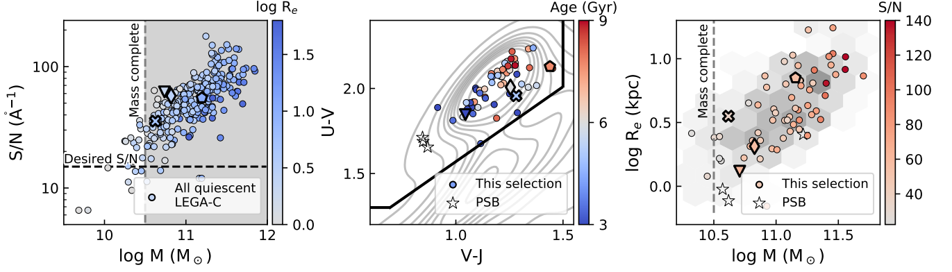
Figure 1. Left: The distribution of stellar mass and S/N at rest-frame 5000 Å of all available quiescent LEGA-C galaxies in the redshift range 0.6 < z < 0.75 colored by their half-light radius. The 95% mass completeness limit ( \log M_*/M_\odot = 10.5 ) and required rest-frame S/N ( = 15 \text{ Å}^{-1} ) are marked. Not all galaxies with S/N > 15 are included in the final sample, as we require that the spectra cover \lambda = 4800 - 5430 \text{ Å} . Center: The selected sample in UVJ space colored by stellar age, as derived from alf . The contours represent the full LEGA-C sample. Right: The selected sample in mass-size space colored by S/N at rest-frame 5000 Å. The density map of parent quiescent sample from the left panel is shown underneath. In all panels we highlight four galaxies using different symbols which correspond to the galaxies in Fig. 2.
