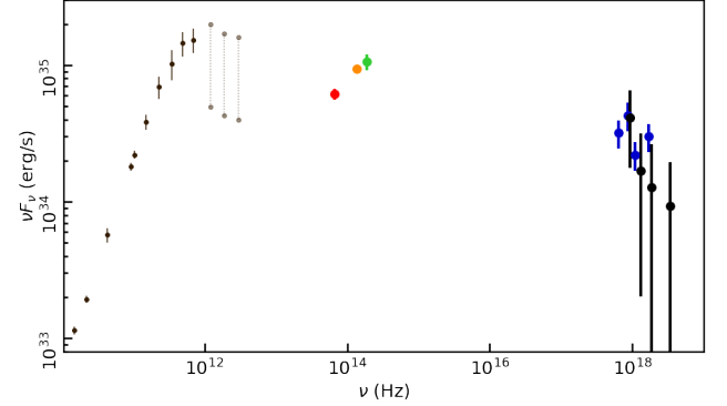
Fig. 4. The mean SED plotted together with the best fit power law slope. The sub-mm SED is plotted for orientation; the radio and sub-mm data are from Falcke et al. (1998); Bower et al. (2015); Brinkerink et al. (2015); Liu et al. (2016); Bower et al. (2019). The far infrared data are from Stone et al. (2016) and von Fellenberg et al. (2018).
