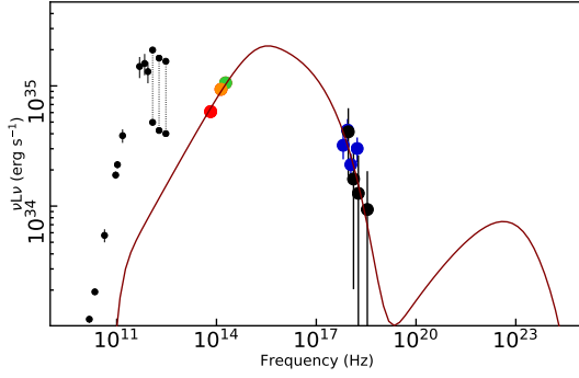
Fig. A.1. Mean SED of Sgr A* during the flare, including the synchrotron self-Compton component of the \text{PLCool}\gamma_{\text{max}} model. This component peaks at \nu \sim 10^{23} Hz.
