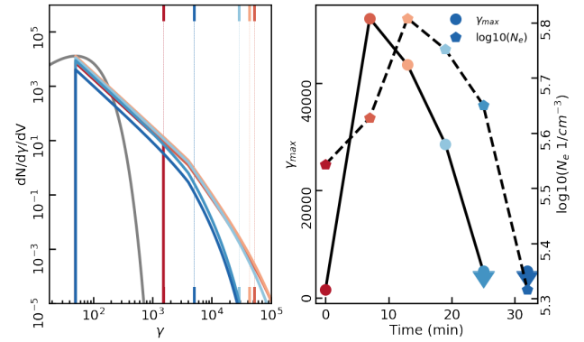
Fig. 10. Left: The evolution of the electron distribution during the flare. The different temporal steps are plotted dark red (T1), progressing to lighter reds (T3), to light blue (T4) to dark blue (T6). The dotted lines indicate the location of \gamma_{\max} . The grey line shows a thermal distribution of electrons, peaking at \gamma \sim 50 , which set the minimum acceleration of the electrons for the flare. Right: evolution of the distribution parameters \gamma_{\max} (shown by the solid line) and n_e (shown by the dashed line).
