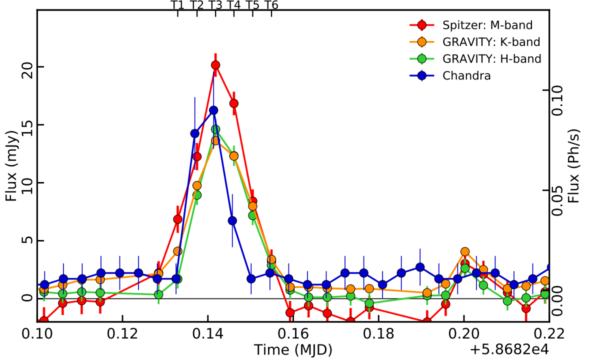
Fig. 2. X-ray and IR light curves of the flare detected on 2019 July 18 th . The blue points show the Chandra light curve in the 2–8 keV band. The red, orange and green points show Spitzer ( M -band), the GRAVITY K -band and H -band light curves corrected for extinction, respectively. The bold ticks on the top abscissa labeled T1, T2, T3, T4, T5, and T6 mark the times that will be used in the subsequent analysis.
