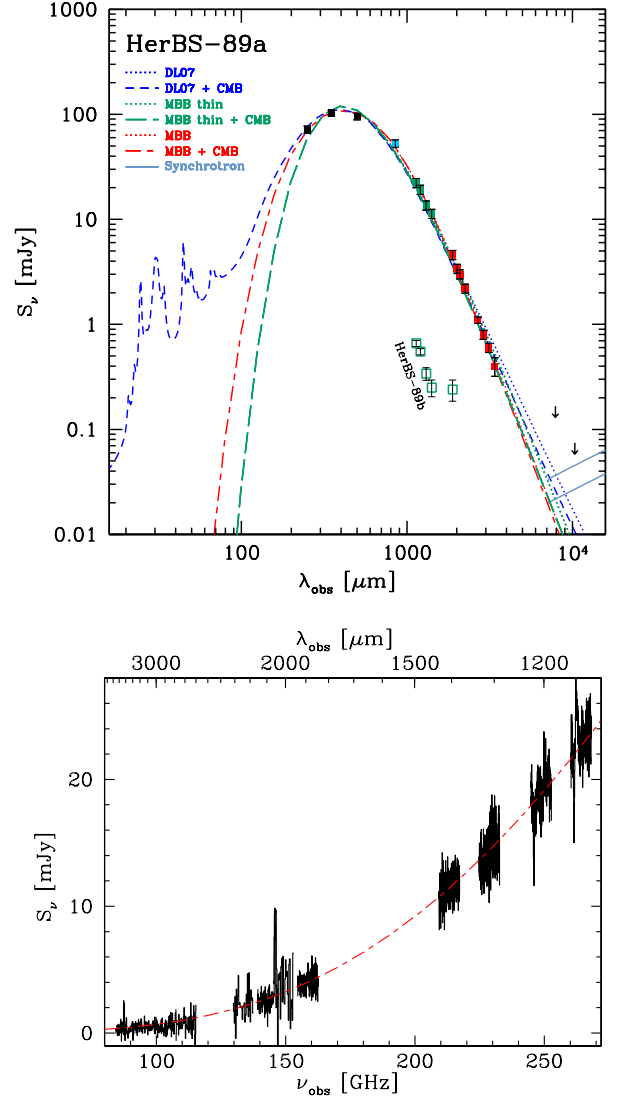
Fig. 13. Top panel: Observed spectral energy distribution of HerBS-89a (filled symbols) and 89b (open symbols). The HerBS-89a data are fit with three different dust models: DL07 (blue lines), optically-thin MBB (green lines); MBB in general form (red lines). The dotted lines represent the models as they are, and the dashed lines include the correction for the effects of CMB (see text for details). The light-blue continuous lines represent the synchrotron emission with a spectral index \alpha = -0.8 , normalized on the basis of the radio-FIR correlation subject to the redshift evolution found by Magnelli et al. (2015, upper line) and Delhaize et al. (2017, lower line). The data include SPIRE flux densities (black dots; from Bakx et al. 2018); SCUBA-2 photometry (blue dot; from Bakx et al. 2020); the NOEMA derived continuum flux densities at 1 mm continuum (green dots) from this work and 2 and 3 mm (red dots) from Neri et al. (2020); and 3\sigma upper limits at 29 and 38 GHz (10 and 7.8 mm, respectively) are derived from the VLA data (arrows). The data for HerBS-89b are taken from this paper for 1 mm and Neri et al. (2020) for 2 mm flux densities. Lower panel: HerBS-89a NOEMA spectra (Neri et al. 2020, and this work) compared to the general form MBB model with CMB correction.
