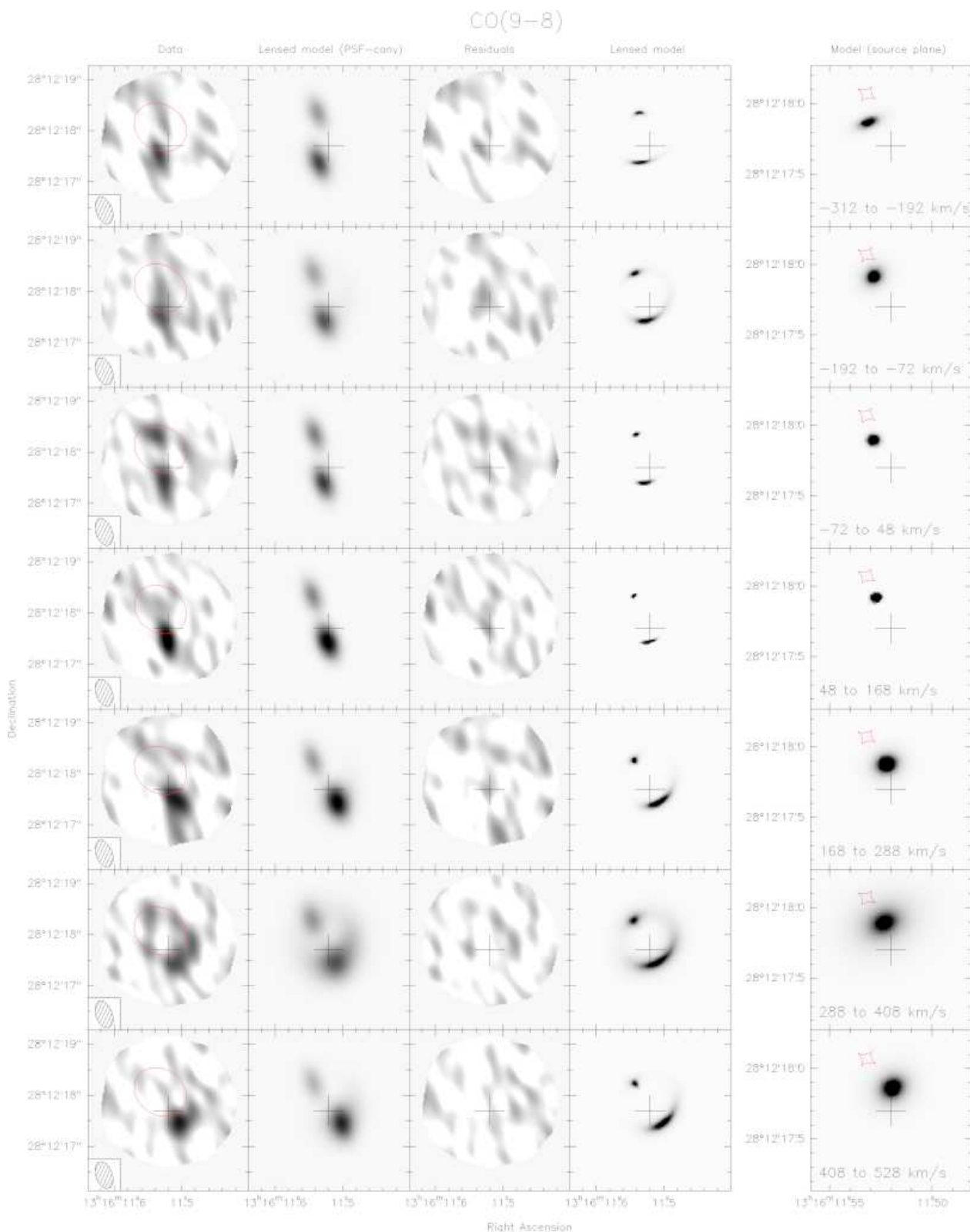
Fig. A.3. Lens modelling of the ^{12}\text{CO}(9-8) spectral channels. The velocity ranges covered by each channel are marked in the right-hand panels. From left to right: observed image (with the synthesized beam shown in the lower left corner) and critical curve (red line); reconstructed model image convolved with the PSF; residuals, reconstructed model image at full angular resolution; and, separated and with a different angular scale, reconstructed source-plane images and caustic curve. The cross shows the central coordinate R.A. 13:16:11.52 and Dec. +28:12:17.7 (J2000).
