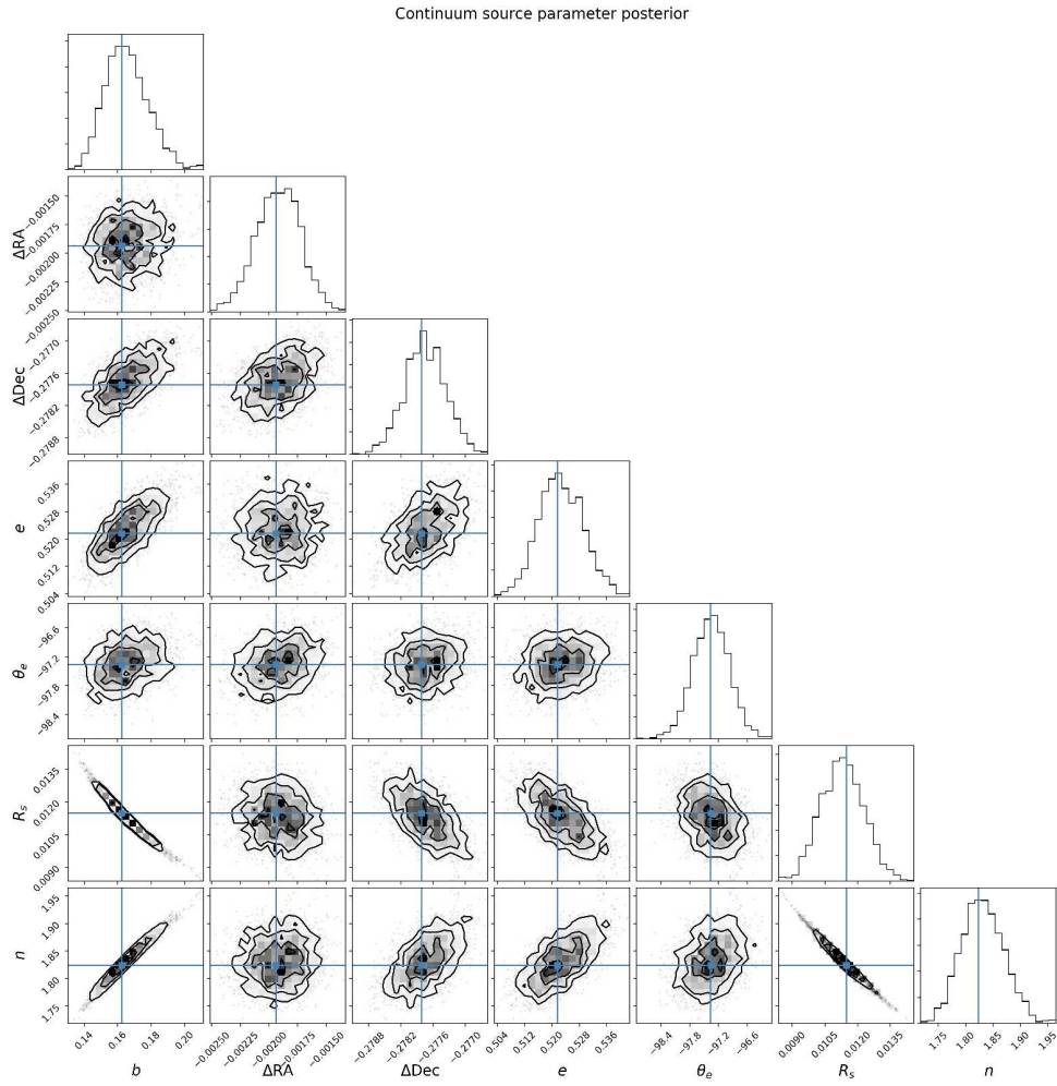
Fig. A.2. Posterior distribution of the parameters of the HerBS-89a lensed source, as obtained by the lens modelling and MCMC runs (see Sect. 5 for details). The constraints are given on the following parameters: the position ( \Delta\text{RA} and \Delta\text{Dec} in arcsec), the Einstein radius ( b ), the ellipticity ( e ), the scale radius ( R_s ), the position angle ( \theta_e ) with the orientation measured east of north and the Sérsic index ( n ). See Fig A.1 for further details.
