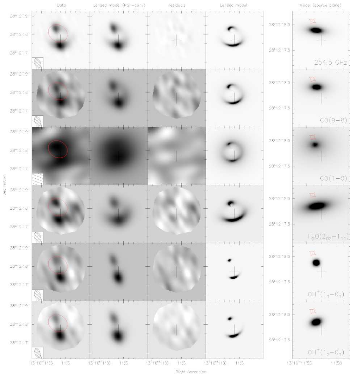
Fig. 12. Lens modelling results for the 1.2 mm dust continuum emission and spectral lines in HerBS-89a (identified in the right most panels). In each row, from left to right: observed image (with the synthesized beam shown in the lower left corner) and critical curve (red line); reconstructed model image convolved with the PSF; residuals; reconstructed model image at full angular resolution; and (separated and with a different angular scale) reconstructed source-plane image and caustic. The residuals are within \pm 2.5\sigma , showing that the model agrees well with the data. The cross shows the coordinates of the phase center of NOEMA observations (R.A. 13:16:11.52 and Dec. +28:12:17.7 in J2000). The \text{OH}^+ absorption lines have been inverted to allow for a positive normalization of the Sérsic profile reconstruction.
