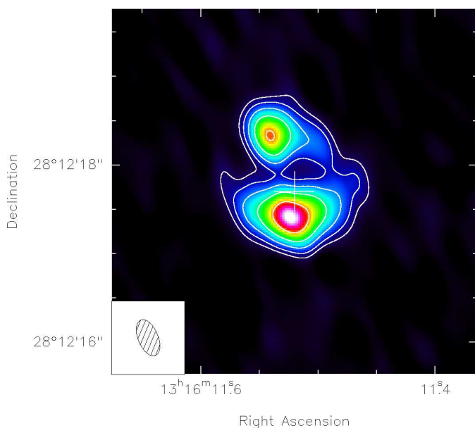
Fig. 2. Zoom-in of the continuum image of HerBS-89a at 254.6 GHz, obtained with uniform weighting, i.e. enhanced resolution, showing the details of the dust-continuum emission, in particular the faint extended emission of the \sim 1'' diameter partial Einstein ring. See caption of Fig.1 for further details.
