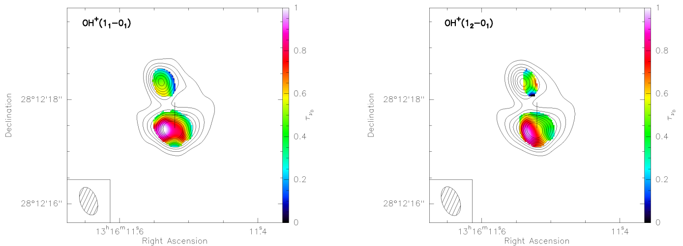
Fig. 6. Maps of the optical depth of the \text{OH}^+(1_1 - 0_1) and \text{OH}^+(1_2 - 0_1) absorption lines, evaluated as F_\nu/F_{\text{cont}} = -e^{-\tau_\nu} at the central frequency \nu_0 of each line.
