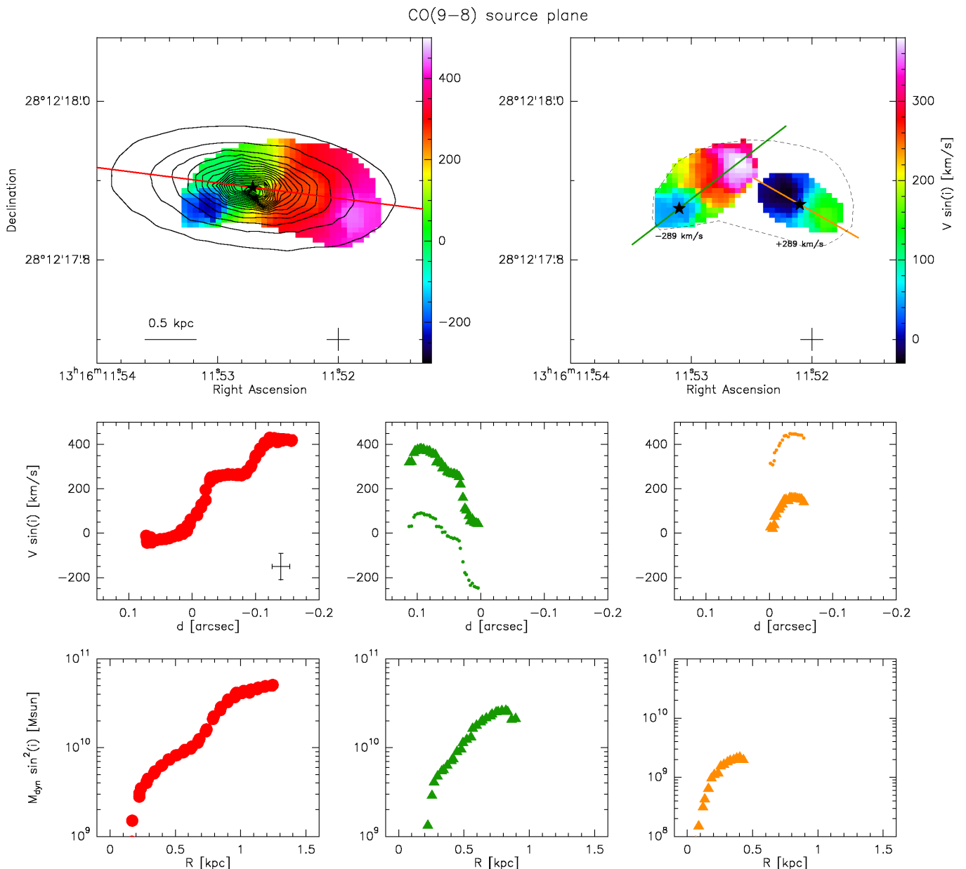
Fig. 18. Kinematic and dynamical analysis of the ^{12}\text{CO}(9-8) emission line in the source plane of HerBS-89a. Top panels: Left First moment map, compared to the Sérsic profile of the dust continuum emission. The contours start from 1/20 of the peak intensity with steps of 1/20^{\text{th}} . The red line marks the continuum major axis. The reference position is defined where the rest-velocity ( V = 0 \text{ km s}^{-1} ) and is denoted with a star. From this position we calculate the radial distance. The cross at the lower right corner marks the phase center of the NOEMA observations. Right: Based on Figs. A.3 and 17, two possible components are identified; the first moment maps of the two components are here shown, after shifting the velocity scale by \pm 289 \text{ km s}^{-1} for clarity. The axes of the two components are shown as green and orange lines. The dashed line marks the contour of the velocity field shown in the top-left panel. Middle panels: Velocity curves extracted along the axes marked in the top panels. Colors match those of the respective axes, with magenta points extracted from the top left moment map and the green and orange points extracted from the top right moment map. In the two right-most panels, the data are shown both before (small symbols) and after (large symbols) shifting by \pm 289 \text{ km s}^{-1} . The amplitude of the error bars is shown in the left-most panel. Bottom panels: Dynamical mass profile as a function of radius, as derived from the velocity curves.
