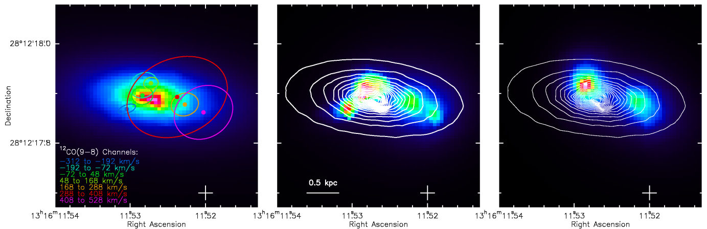
Fig. 17. Left panel: Positions (colored thick dots) and shapes (ellipses) of the reconstructed profiles of the individual ^{12}\text{CO}(9-8) channels, overplotted on the map of the dust continuum emission in the source plane. The ellipses are plotted at 1/20^{\text{th}} of the peak flux of each reconstructed channel map. Central panel: Zeroth moment map of the ^{12}\text{CO}(9-8) emission line derived from the reconstruction of the seven individual channels shown in the left panel. The contours show the dust continuum emission, starting at 1/20^{\text{th}} of the peak flux in steps of 1/20^{\text{th}} (see also Fig. A.3). Right panel: Zeroth moment map obtained splitting the ^{12}\text{CO}(9-8) in two halves, corresponding to the velocity ranges from -312 to 168 \text{km s}^{-1} and from 168 to 528 \text{km s}^{-1} , and reconstructing them separately. In all panels, the cross at the lower right corner marks the phase center of the NOEMA observations.
