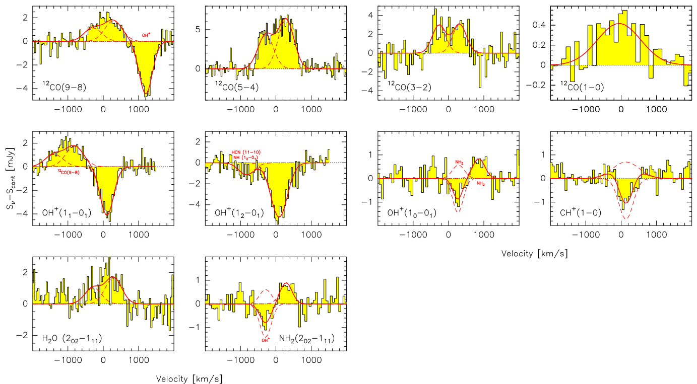
Fig. 5. The spectra of the molecular emission and absorption lines detected in HerBS-89a reported in this study, together with the ^{12}\text{CO}(5-4) and ^{12}\text{CO}(3-2) spectra from Neri et al. (2020). Each molecular line is identified in the lower corner of each panel (labeled in black) and, in the case of a line overlap, i.e., ^{12}\text{CO}(9-8)/\text{OH}^+(1_1-0_1) , \text{OH}^+(1_2-0_1)/\text{HCN}(11-10) and \text{OH}^+(1_0-0_1)/\text{o-NH}_2(2_{02}-1_{11}) , the second molecular line is labelled in red. The spectra are displayed with the continuum subtracted and, in each panel, the molecular line (labeled in black) is plotted relative to the zero velocity corresponding to its rest frequency. Fits to the emission and absorption molecular lines are shown as solid lines, and, when multi-component and/or multiple lines have been fitted, they are displayed individually as dashed lines (see text for details).
