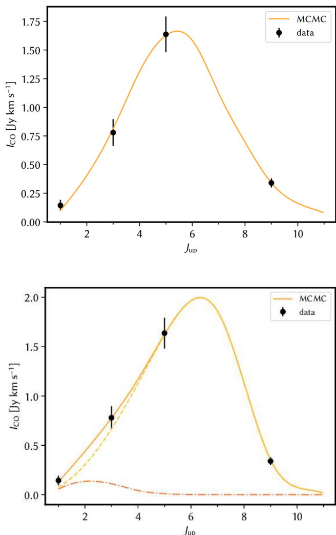
Fig. 15. Large Velocity Gradient (LVG) model fit to the ^{12}\text{CO} SLED of HerBS-89a (after correcting for lens magnification). Top Panel: The data are shown as black dots and the solid curve shows the best fit from the single component (MCMC) model corresponding to the maximum posterior possibility (see Sect. 6.3 for details). Bottom Panel: Two-components fit, including an additional cold and extended component (darker, dot-dashed line).
