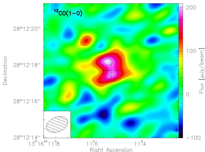
Fig. 8. ^{12}\text{CO}(1-0) emission in HerBS-89a. The 1\sigma sensitivity is 32.1 \mu\text{Jy}/\text{beam} and the beam size (shown in the lower left corner) is 1''.24 \times 0''.79 (P.A. -62.3^\circ , E of N). The emission is resolved in the east-west direction. Contours are in 1\sigma steps starting from the 3\sigma level.
