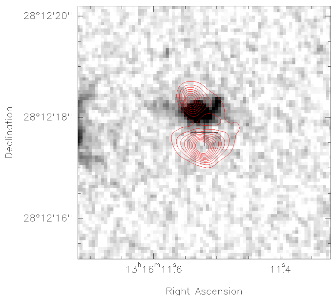
Fig. 9. View of the foreground lensing galaxy in the HST WFC3 F110W filter ( 1.15 \mu\text{m} ) image, with the 254.6 GHz dust continuum emission measured with NOEMA superposed as red contours.
