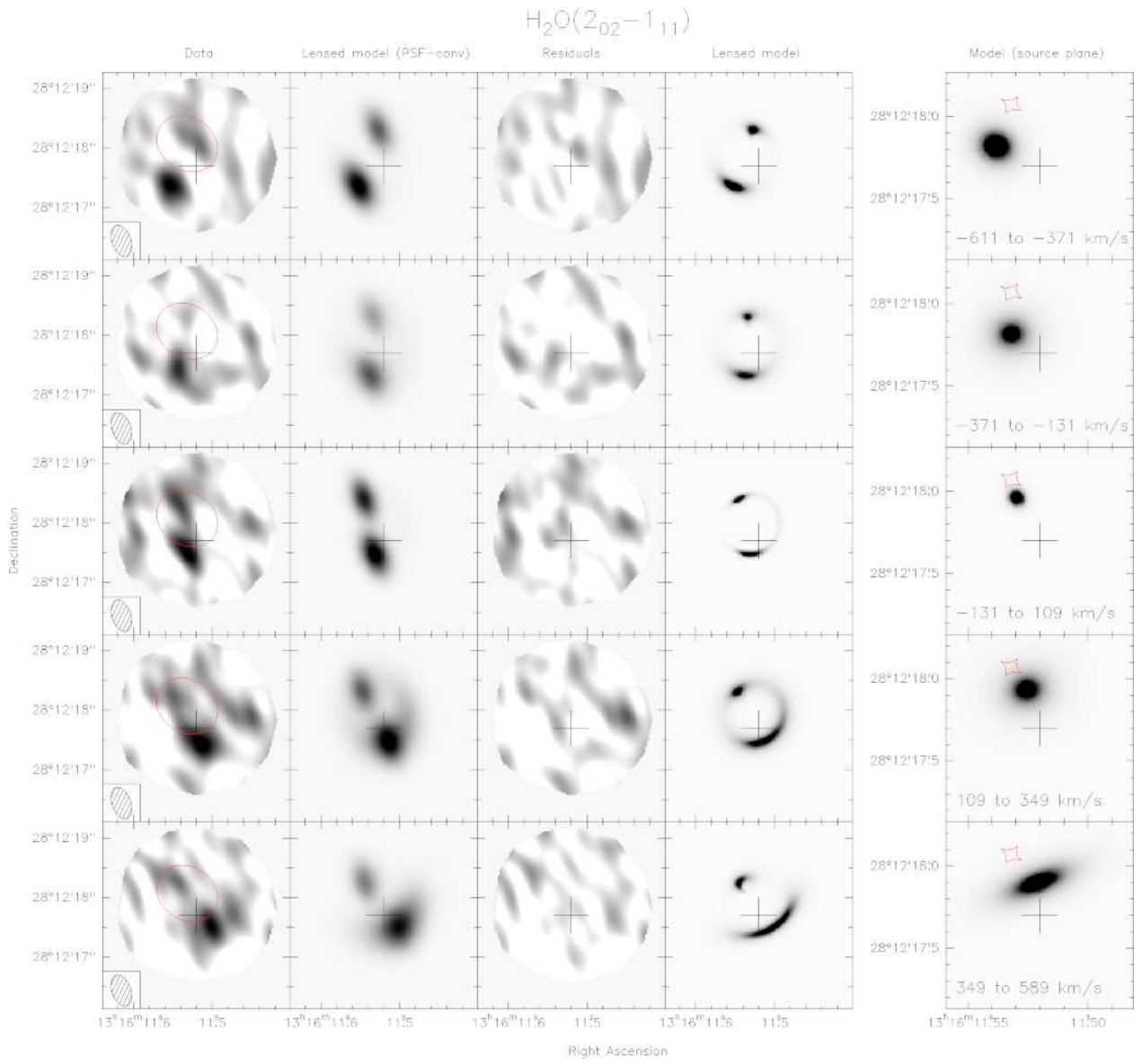
Fig. A.4. Lens modelling of the \text{H}_2\text{O}(2_{02}-1_{11}) spectral channels. The velocity ranges covered by each channel are marked in the right-hand panels. See Fig. A.3 for further details.
