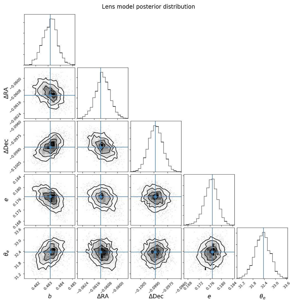
Fig. A.1. Posterior distribution of the parameters of the foreground lens object, as obtained by the lens modelling and MCMC runs (see Sect. 5 for details). The constraints are given on the following parameters: the position ( \Delta RA and \Delta Dec in arcsec), the Einstein radius ( b ), the ellipticity ( e ), and the position angle ( \theta_e ) with the orientation measured east of north. The contours show the 0.5, 1, 1.5, and 2\sigma of the integrated likelihood. The mean and the \pm 1\sigma interval around the mean are displayed as histograms along the diagonal of the plot.
