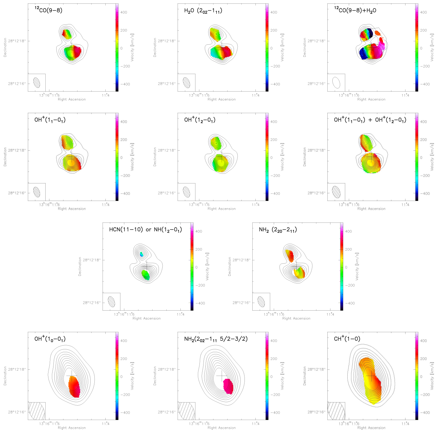
Fig. 7. Velocity field maps (shown in colors) in each of the molecular emission and absorption lines detected in HerBS-89a superimposed on the continuum at the individual frequencies of each molecular line (in contours of 10\sigma spacing). The velocity maps were obtained above 3\sigma thresholds in the zero-th moment map of the molecular lines. As in Fig. 4, the three top rows display the high-angular resolution data, whereas the lower row shows the lower-angular resolution images. The upper right panel presents the combined ^{12}\text{CO}(9-8) and \text{H}_2\text{O}(2_{02}-1_{11}) image that reveals the kinematics along the western arm of the partial Einstein ring. The right panel in the second row displays the combined velocity field of the two \text{OH}^+ absorption lines ( (1_1-0_1) and (1_2-0_1) ). The synthesized beam is shown in the lower left corner of each of the images.
