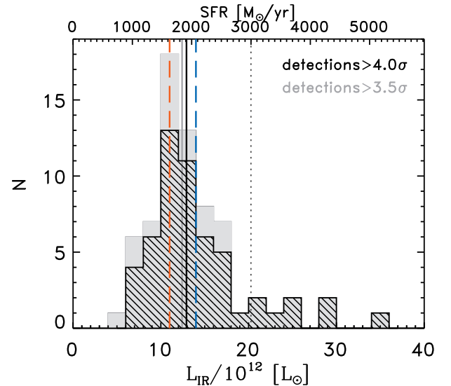
Figure 12. Histogram of IR luminosities and SFRs estimated for the AzTEC detections above 4\sigma (black line filled) and 3.5\sigma (light grey). The median values of both distributions are indicated with vertical lines, including the median luminosity for the 4\sigma single systems ( 1.4 \times 10^{13} L_{\odot} ; dashed blue) and the components of the multiple systems ( 1.1 \times 10^{13} L_{\odot} ; dashed orange). Eight sources in our sample show L_{\text{IR}} > 2 \times 10^{13} L_{\odot} and SFRs > 3000 \text{M}_{\odot} \text{yr}^{-1} (dotted vertical line), representing a population of extreme star-forming galaxies that cannot be explained within current physically plausible models, unless gravitational lensing effects are included.
