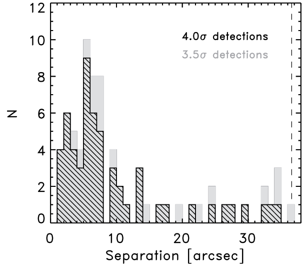
Figure 8. Histogram of the separations between the AzTEC detection and H-ATLAS targeted positions. Although a radius \theta_{500\mu\text{m}} = 36.6\text{ arcsec} (vertical dashed line) is used for our counterpart analysis, \sim 82 per cent (75 per cent) of the 4\sigma ( 3.5\sigma ) AzTEC sources are separated by \lesssim 15\text{ arcsec} off the H-ATLAS target, were the reliability of the detections is \gtrsim 98 per cent (90 per cent; see Fig. 6).
