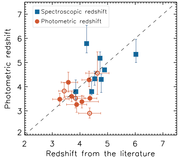
Figure 10. Comparison between the photometric redshifts derived in this work and those reported in the literature ( Iverson et al. 2016 ; Fudamoto et al. 2017 ; Duivenvoorden et al. 2018 ; Zavala et al. 2018a ; Ma et al. 2019 ), including both photometric (orange circles) and spectroscopic redshifts (blue squares; see Table 2 and §4.1 ). The open circles represent sources which are classified as multiple systems based on our AzTEC observations, while all the remaining sources correspond to single systems. In general, our estimated redshifts are in good agreement with those reported in the literature with a mean redshift deviation of \Delta z / (1 + z_{\text{ref}}) = 0.09 (considering only those sources with spectroscopic redshifts).
