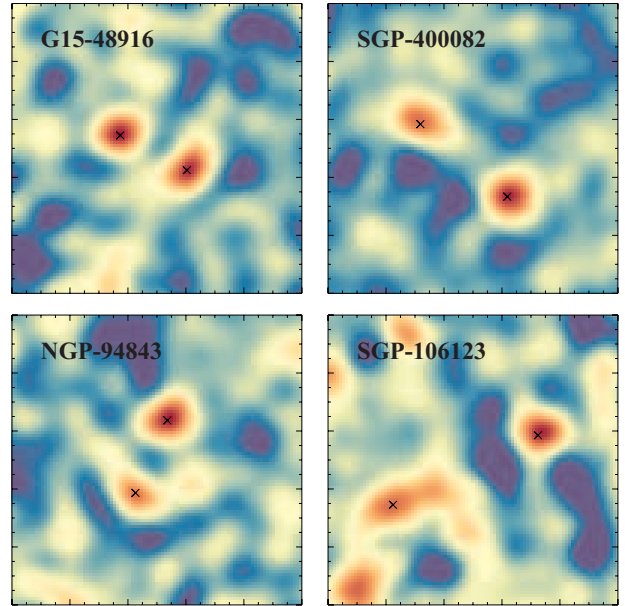
Figure 13. 76 \text{ arcsec} \times 76 \text{ arcsec} AzTEC 1.1 mm SNR maps of the four most likely physically interacting galaxy candidates in the sample. All the detected sources fall within 36.6 \text{ arcsec} of the original Herschel position (the beamsize at 500 \mu\text{m} ) and have individual photometric redshifts in agreement with each other within the error bars. These sources, which are typically missed in interferometric observations due to their small fields of view, are likely galaxy over-densities and/or pre-coalescence galaxy mergers.
