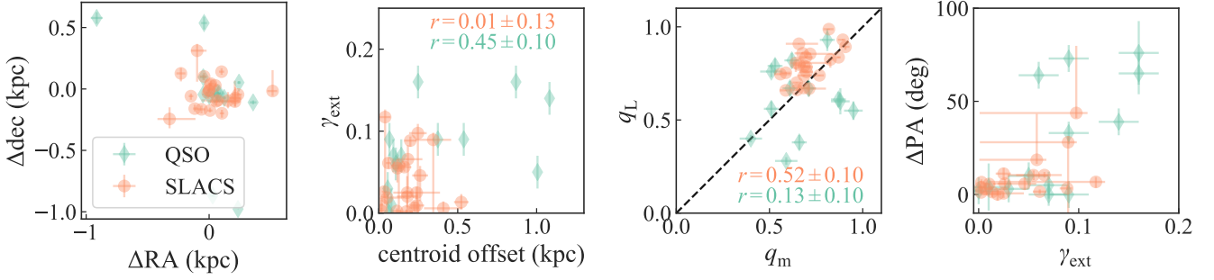
Figure A1. The alignment between mass and light distribution for SLACS lenses in our sample (orange) and quasar lenses from Shajib et al. (2019) , green). First panel: The angular offset between the centroids of mass and light. For our fiducial cosmology, the offset distribution for the SLACS lenses has a 95 per cent upper limit of 426 \pm 68 pc. Second panel: Distribution of the absolute centroid offsets and external shear. These two quantities are moderately correlated for the quasar lenses from Shajib et al. (2019) with biweight midcorrelation r = 0.45 \pm 0.10 , which indicates that the presence of nearby perturbers may cause an offset between mass and light centroids in the quasar lenses. However, there is no such correlation for the SLACS lenses. Although the shear distribution for the SLACS lenses is at a lower range than that of the quasar lenses, thus any such potential correlation is hard to identify given the measurement uncertainties. Third panel: The distribution of mass and light axis ratios. The axis ratios are weakly correlated with biweight midcorrelation r = 0.54 \pm 0.08 . Fourth panel: The distribution of major axis misalignment between mass and light and external shear. The 19 lenses from our sample of 23 that have q_L < 0.9 and q_m < 0.9 – and thus reliable position angle estimates – are plotted in this panel. For these SLACS lenses, misalignment angle \Delta PA > 12 deg are the systems with \gamma_{\text{ext}} \gtrsim 0.05 .
