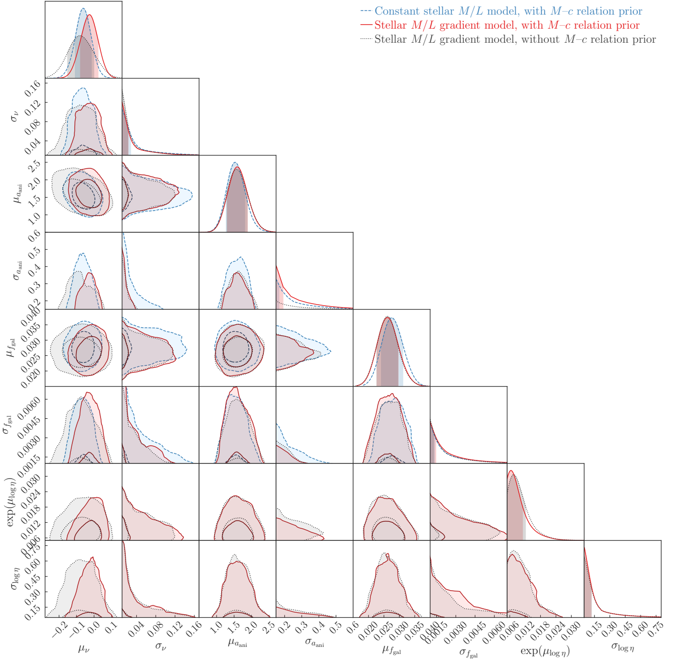
Figure 6. Distribution of population-level parameters assuming Gaussian distribution for the halo response parameter \nu , the anisotropy scaling parameter a_{\text{ani}} , fraction of the total mass that cools to form stars f_{\text{gal}} , and \log \eta where \eta is the M/L gradient's exponent. The three model setups illustrated are a constant stellar M/L model with the M-c relation prior (blue dashed line), a stellar M/L gradient model with the M-c relation prior (red solid line), and a stellar M/L gradient model without the M-c relation prior (dotted grey line). The darker and lighter regions represent 68 per cent and 95 per cent credible regions, respectively. The 2D contours and 1D distributions are smoothed with a Gaussian kernel of 1.5\sigma bandwidth. The point-estimate of these parameters are given in Table 2. Figure 7 highlights the central parameters in our model along with their interpretations.
