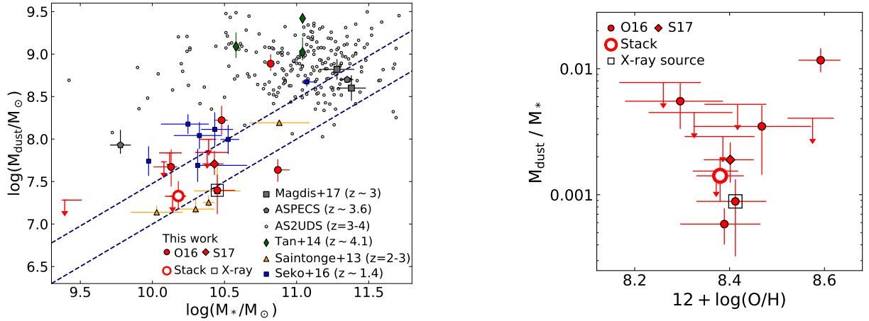
Figure 3. (Left) Relation between stellar mass and dust mass for the star-forming galaxies at z \sim 3.3 together with galaxies at z \sim 1.4\text{--}4 from the literature. The dashed lines correspond to constant dust-to-stellar mass ratios of M_{\text{dust}}/M_* = 1 \times 10^{-3} and 3 \times 10^{-3} . We show the galaxy samples of Tan et al. (2014), Magdis et al. (2017), and Saintonge et al. (2013) after dividing their dust masses by a factor of two to correct for the difference of the assumed \kappa_{\text{abs}} . The star-forming galaxies at z \sim 3.3 have similar dust-to-stellar mass ratios as more massive star-forming galaxies from Magdis et al. (2017) and ASPECS (Aravena et al. 2020). (Right) Relation between the gas-phase metallicity and dust-to-stellar mass ratio for the star-forming galaxies at z \sim 3.3 . We find no clear correlation between the gas-phase metallicity and dust-to-stellar mass ratio among our sample.
