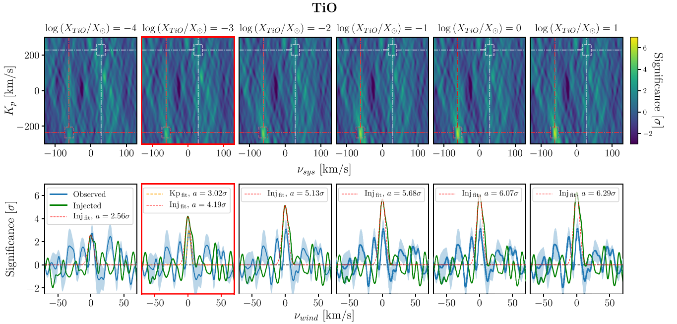
Figure 10. Same as Figs 8 and 9 but for TiO models. Again the panels with red borders represent the injection models calculated for the abundance value retrieved from the FORS2 transmission spectrum. In the second panel of the bottom row, an additional Gaussian model is fitted to the apparent peak detected at the K_p of planet (orange dashed line), with an amplitude of 3.02 \pm 0.15 \sigma , and centred on a radial velocity value 1.50 \pm 0.34 \text{ km s}^{-1} offset from the calculated \nu_{\text{sys}} .
