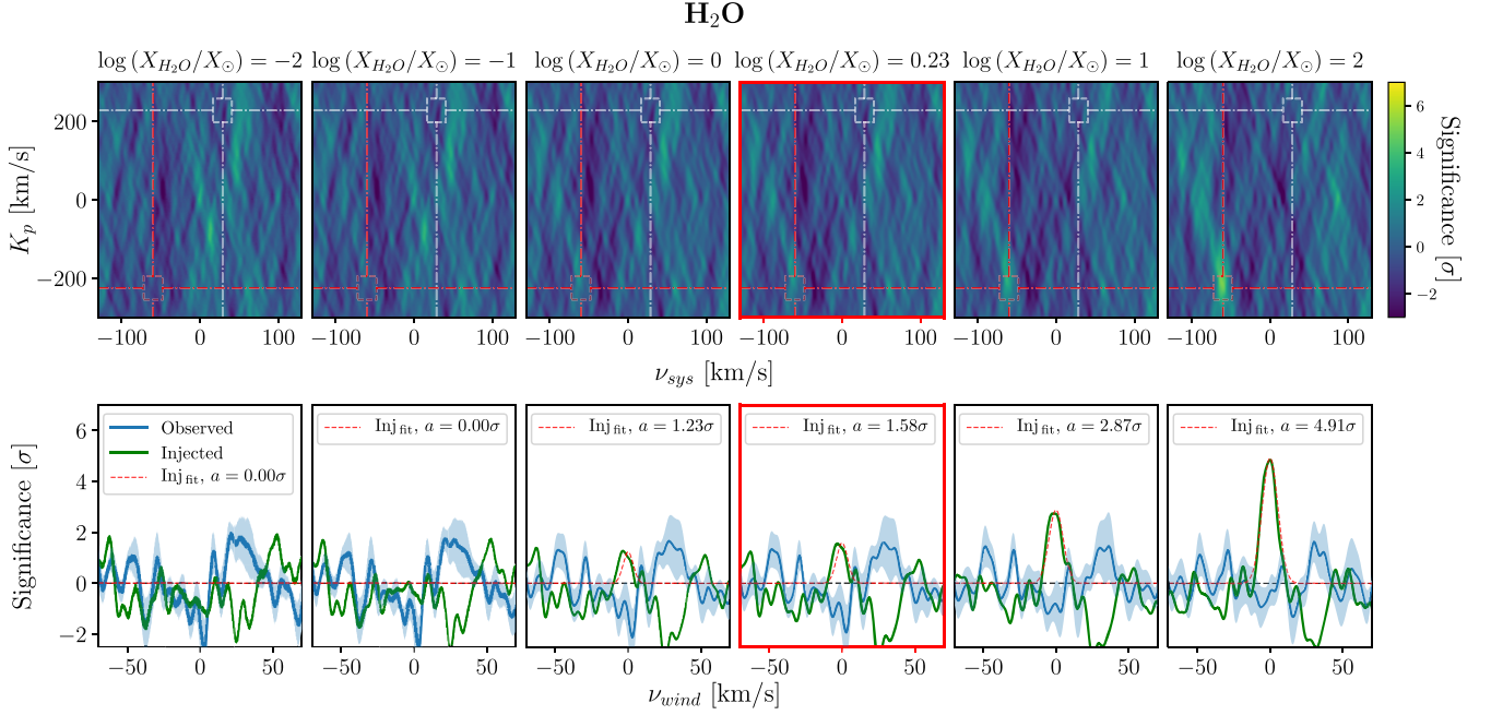
Figure 9. Same as Fig. 8 but for H 2 O template and injection models. The panels with red borders show the injected model representing the abundance value retrieved from the FORS2 low-resolution transmission spectrum in Sedaghati et al. (2017).
