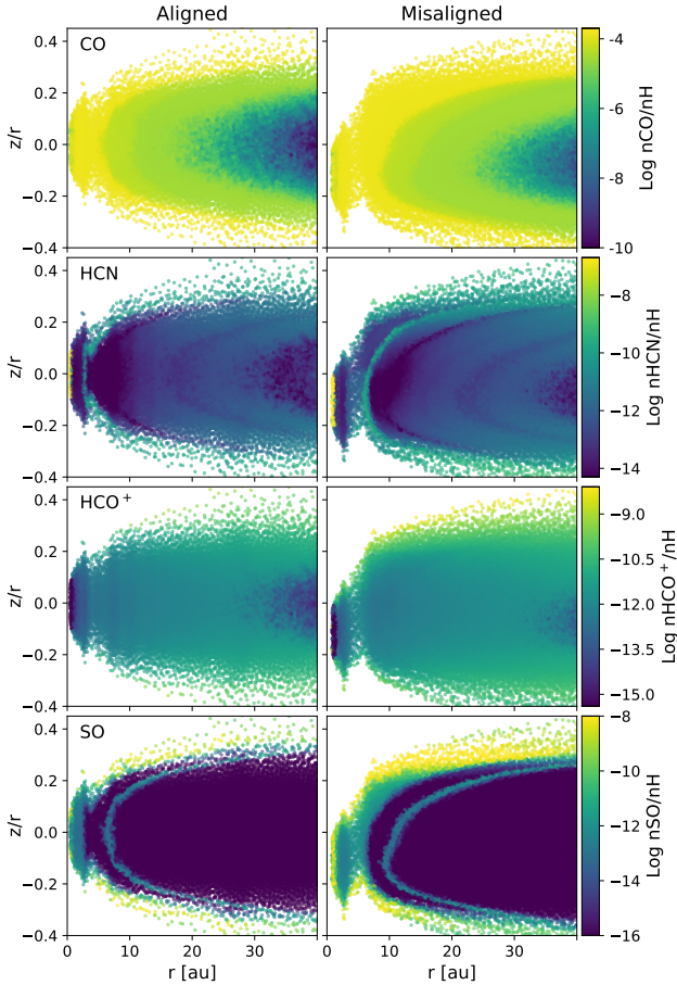
Figure 4. Selected molecular abundances for the same disc cross-sections as in Fig. 3. Left columns: aligned planet located at 5 au. Right columns: misaligned planet.
