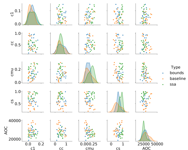
Figure 11: Distribution of the continuous hyperparameters from the elite configurations found in all three experiments.
