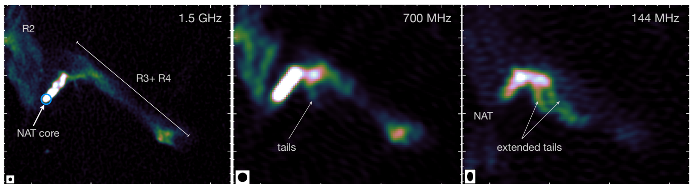
Fig. 4. NAT galaxy located at the center of the relic at 1.5 GHz (at 1.2'' resolution), 700 MHz (at 3.5'' resolution), and 144 MHz (at 4.5'' × 3.4'' resolution). To compare radio morphology of the NAT galaxy at different frequencies, the colors in these images were scaled manually. The image obtained with the new data evidently shows that both tails of the NAT bend down south rather fading or merging into the R3 region of the relic. The bent parts of tails are marginally visible in the VLA L-band image. As discussed in Sect. 5.4, the NAT and the southern part of the relic could be two different structures along the same line of sight seen in projection.
