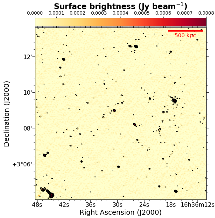
Fig. A.13. PSZ1 G019.12+3123 GMRT 610 MHz image. Contours start at 3-\sigma_{rms} and are spaced by a factor of two. 1-\sigma_{rms} = 0.035 mJy/beam with beam= 5.0'' \times 3.8'' .
