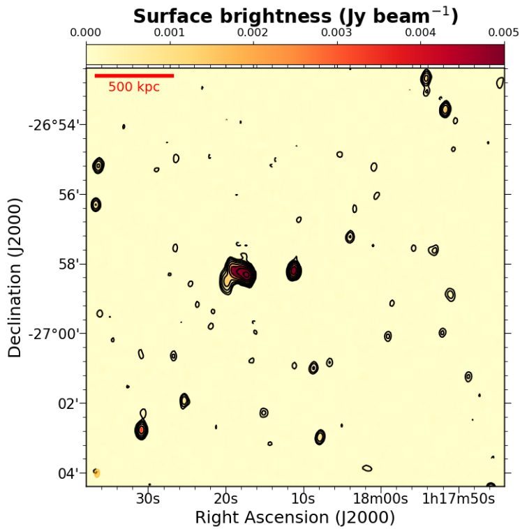
Fig. A.4. A2895 JVLA C array 1.5 GHz image. Contours start at 3-\sigma_{rms} and are spaced by a factor of 2. 1-\sigma_{rms} = 0.04 mJy/beam with beam= 14.6'' \times 9.0'' .
