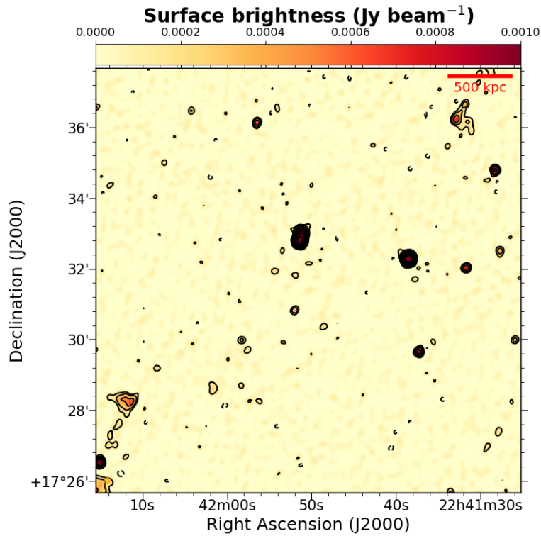
Fig. A.6. A2472 JVLA C array 1.5 GHz image. Contours start at 3-\sigma_{rms} and are spaced by a factor of two. 1-\sigma_{rms} = 0.04 mJy/beam with beam= 10.5'' \times 10.1'' .
