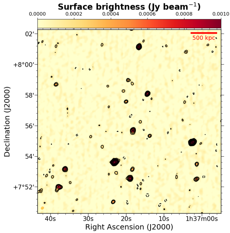
Fig. A.5. A220 JVLA C array 1.5 GHz image. Contours start at 3-\sigma_{rms} and are spaced by a factor of two. 1-\sigma_{rms} = 0.045 mJy/beam with beam= 11.6'' \times 9.8'' .
