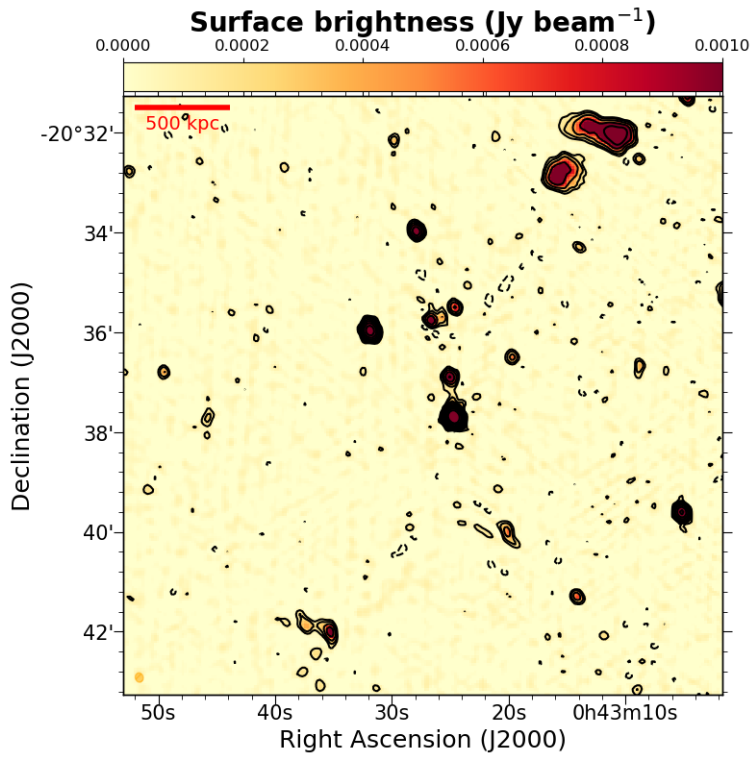
Fig. A.2. A2813 JVLA C array 1.5 GHz image. Contours start at 3-\sigma_{rms} and are spaced by a factor of two. 1-\sigma_{rms} = 0.035 mJy/beam with beam= 11.4'' \times 9.5'' .
