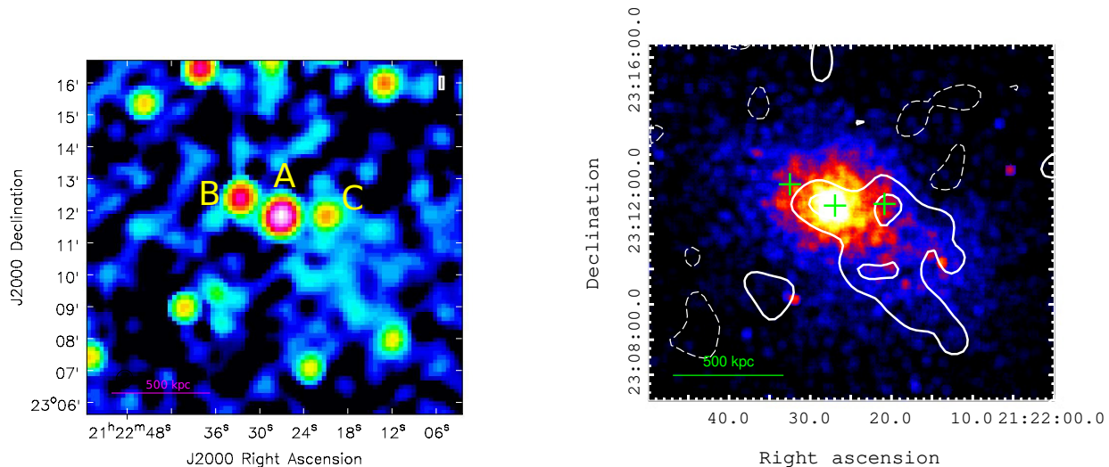
Fig. 5. JVLA image of the cluster Z2120. Left: JVLA D array image. The resolution is 33'' \times 30'' and the rms noise is 0.06 mJy/beam. Labels mark the discrete sources in the cluster field. Right: Low-resolution ( 55'' \times 54'' ) JVLA contours after the compact sources subtraction overlaid over the X-ray Chandra image. Contours are drawn at (3, 6, \dots) \times \sigma , with \sigma = 0.1 mJy/beam. The 2\text{-}\sigma negative contour is dashed. The green crosses mark the position of the three sources at the cluster centre, which have been subtracted.
