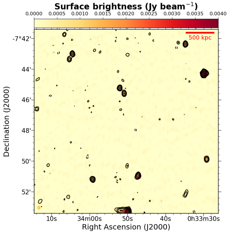
Fig. A.1. A56 JVLA C array 1.5 GHz image. Contours start at 3-\sigma_{rms} and are spaced by a factor of two. 1-\sigma_{rms} = 0.08 mJy/beam with beam= 13.'' \times 10.4'' .
