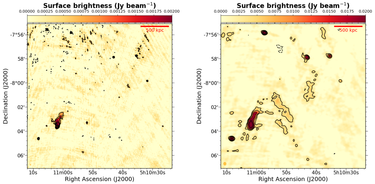
Fig. A.15. Images of the cluster RXC J0510.7-0801. Left panel: GMRT 610 MHz image. Contours start at 3-\sigma_{rms} and are spaced by a factor of two. 1-\sigma_{rms} = 0.2 mJy/beam with beam= 5.4 \times 4.8 . Right panel: RXC J0510.7-0801 GMRT 240 MHz image. Contours start at 3-\sigma_{rms} and are spaced by a factor of two. 1-\sigma_{rms} = 1.2 mJy/beam with beam= 15.7'' \times 13.1'' .
