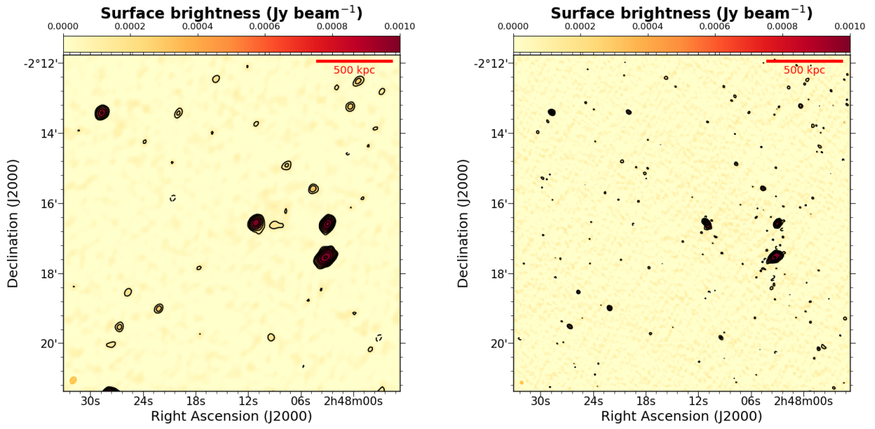
Fig. A.3. Images of the cluster A384. Left panel: JVLA C array 1.5 GHz image. Contours start at 3-\sigma_{rms} and are spaced by a factor of two. 1-\sigma_{rms} = 0.035 mJy/beam with beam= 13.5'' \times 10.4'' . Right panel: GMRT 610 MHz image. Contours start at 3-\sigma_{rms} and are spaced by a factor of two. 1-\sigma_{rms} = 0.05 mJy/beam with beam= 5.9'' \times 4.8'' .
