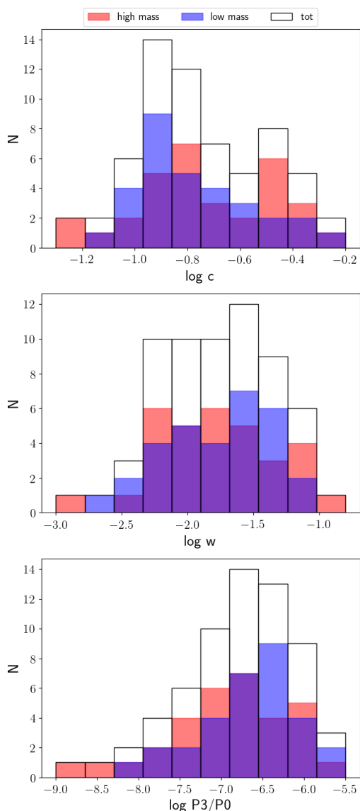
Fig. 11. Concentration parameter ( top ), centroid shift ( middle ) and power ratios ( bottom ) distribution of the clusters with available X-ray Chandra data. The red histogram refers to high mass clusters ( M_{500} \geq 7 \times 10^{14} M_{\odot} ), while the blue histogram refers to low mass ( M_{500} < 7 \times 10^{14} M_{\odot} ) clusters.
