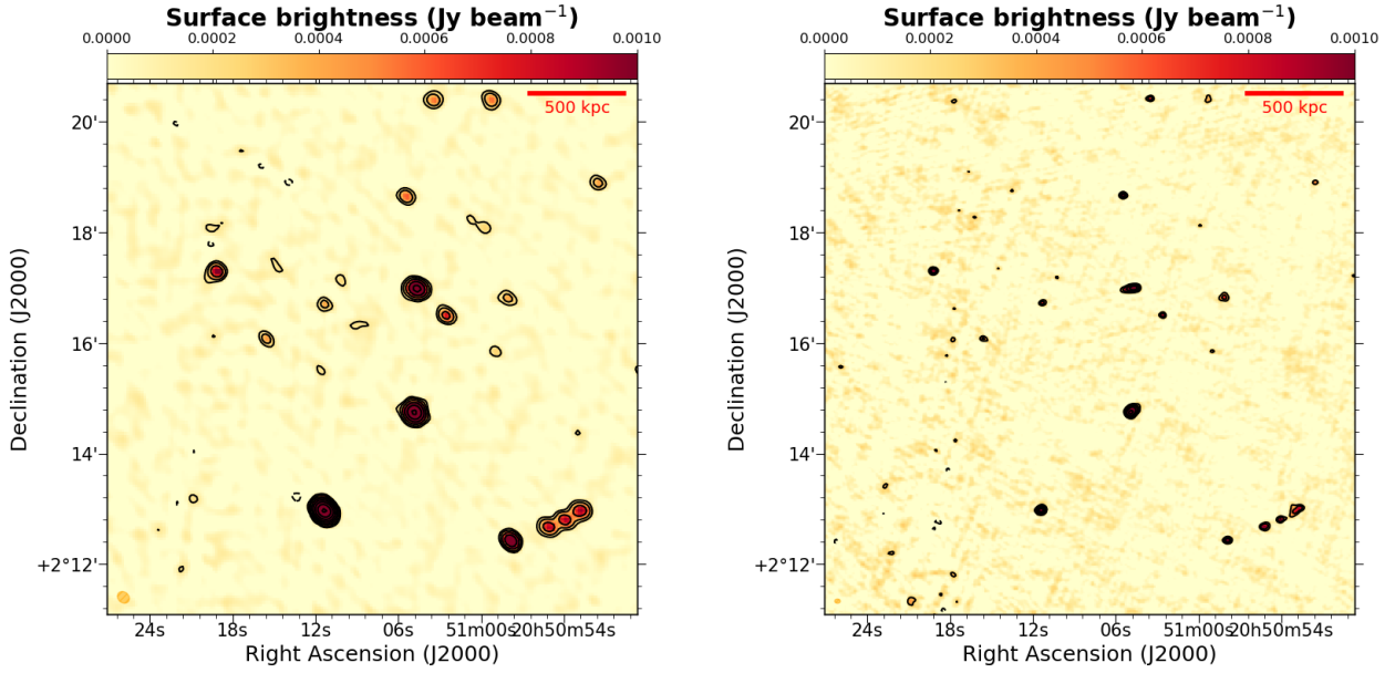
Fig. A.8. Images of the cluster RXC J2051.1+0216. Left panel: JVLA C array 1.5 GHz image. Contours start at 3-\sigma_{rms} and are spaced by a factor of two. 1-\sigma_{rms} = 0.05 mJy/beam with beam= 14.1'' \times 11.5'' . Right panel: GMRT 610 MHz image. Contours start at 3-\sigma_{rms} and are spaced by a factor of two. 1-\sigma_{rms} = 0.1 mJy/beam with beam= 6.0'' \times 4.8'' .
