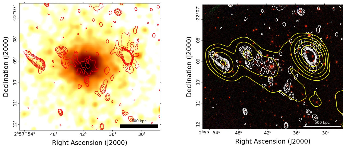
Fig. 8. Images of the cluster A402. Left: GMRT 330 MHz contours superimposed on the X-ray Chandra image of the cluster. Contours start at 0.35 mJy/beam and are spaced by a factor of two. The first negative contour is dashed. The beam is 13.4'' \times 8.6'' and the rms noise of the radio image is \sim 0.1 mJy/beam. Right: PanSTARRS optical image of the field of A402 with the same contours of the left panel (white) plus the low-resolution GMRT 330 MHz contours (yellow). Contours start at 3 mJy/beam and are spaced by a factor of two. The rms noise of the low-resolution image is \sim 1 mJy/beam with beam= 57'' \times 42'' .
