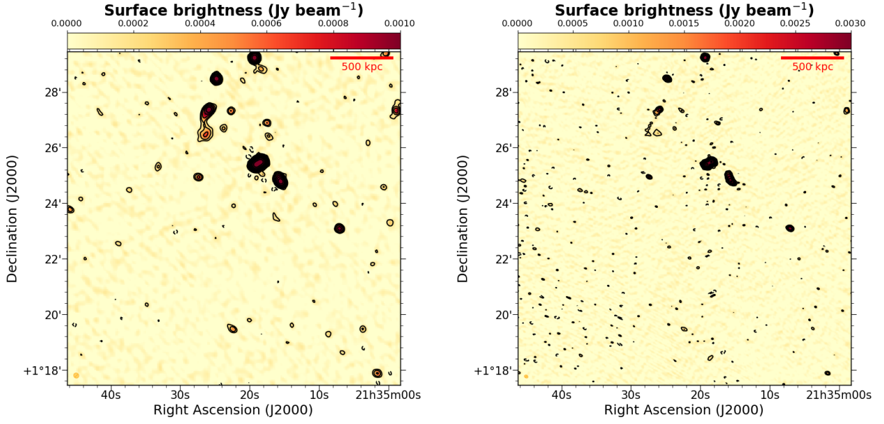
Fig. A.7. Images of the cluster A2355. Left panel: JVLA C array 1.5 GHz image. Contours start at 3-\sigma_{rms} and are spaced by a factor of two. 1-\sigma_{rms} = 0.04 mJy/beam with beam= 11.6'' \times 10.8'' . Right panel: GMRT 610 MHz image. Contours start at 3-\sigma_{rms} and are spaced by a factor of two. 1-\sigma_{rms} = 0.13 mJy/beam with beam= 8.3'' \times 6.1'' .
