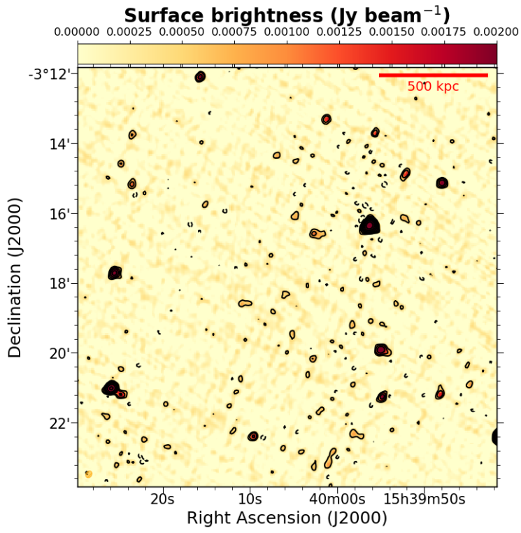
Fig. A.17. A2104 GMRT 240 MHz image. Contours start at 3-\sigma_{rms} and are spaced by a factor of two. 1-\sigma_{rms} = 0.13 \text{ mJy/beam} with \text{beam} = 13.3'' \times 10.4'' .
