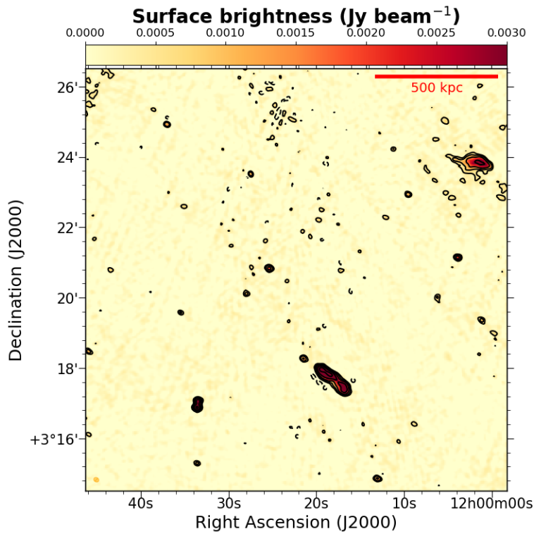
Fig. A.16. A1437 GMRT 330 MHz image. Contours start at 3-\sigma_{rms} and are spaced by a factor of two. 1-\sigma_{rms} = 0.4 mJy/beam with beam= 9.0'' \times 7.4'' .
