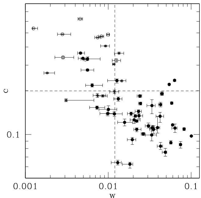
Fig. 12. c - w morphological diagram. Filled dots are clusters classified as merging from the visual inspection, empty dots are visually classified as relaxed and asterisks are visually classified as intermediate. Black lines are adapted from Cassano et al. (2010) and are c = 0.2 and w = 0.012 .
