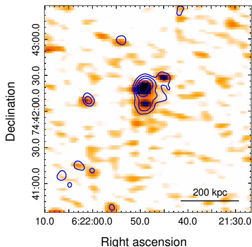
Fig. 4. JVLA C array 10.3'' \times 5.1'' resolution image of the center of PSZG139.61+2420 with GMRT 610 MHz contours overlaid. Contours are (\pm 3, 6, 9, 12, \dots) \times \sigma_{rms} with \sigma_{rms} = 0.03 mJy/beam and beam = 7'' \times 7'' (Giacintucci et al. 2017).
