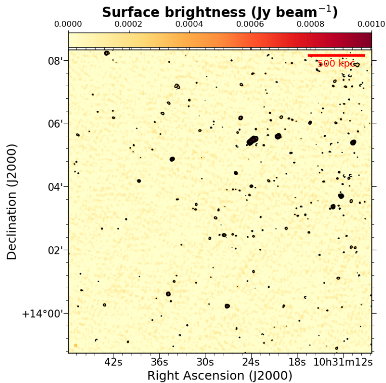
Fig. A.10. Zwcl 1028.8+1419 GMRT 610 MHz image. Contours start at 3-\sigma_{rms} and are spaced by a factor of two. 1-\sigma_{rms} = 0.056 mJy/beam with beam= 5.3'' \times 4.8'' .
