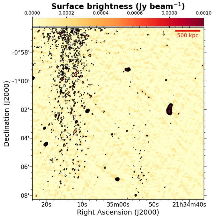
Fig. A.14. MACS J2135-010 GMRT 610 MHz image. Contours start at 3-\sigma_{rms} and are spaced by a factor of two. 1-\sigma_{rms} = 0.08 mJy/beam with beam= 7.8'' \times 5.8'' .
