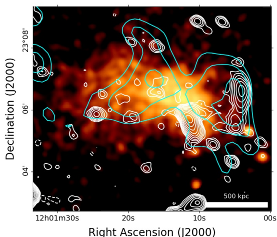
Fig. 3. X-ray Chandra image of A1443 with JVLA high-resolution (white) and low-resolution (cyan) contours overlaid. Contours start at 3-\sigma and are spaced by a factor of two. 1-\sigma rms noise is 0.02 mJy/beam with beam= 15'' \times 12'' (white contours) and it is 0.08 mJy/beam with beam= 55'' \times 54'' (cyan contours).
