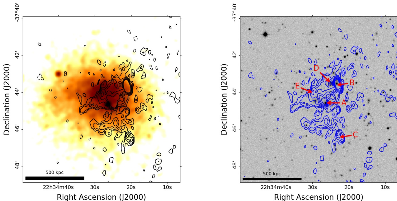
Fig. 2. Images of the cluster A3888. Left: X-ray Chandra image (colours) with GMRT 330 MHz contours superimposed. Contours start from 0.9 mJy/beam and are spaced by a factor of two. The -0.9 mJy/beam contour is dashed. Right: Same contours as in the left panel superimposed on the optical DSS image. Labels mark the position of discrete radio sources (A to D) and E indicates a patch of diffuse emission with no optical counterpart that we consider to be part of the halo.
