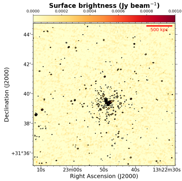
Fig. A.11. RXC J1322.8+3138 GMRT 610 MHz image. Contours start at 3-\sigma_{rms} and are spaced by a factor of two. 1-\sigma_{rms} = 0.06 mJy/beam with beam= 5.7'' \times 4.4'' .
