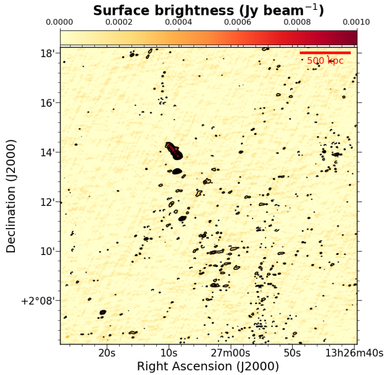
Fig. A.12. A1733 GMRT 610 MHz image. Contours start at 3-\sigma_{rms} and are spaced by a factor of two. 1-\sigma_{rms} = 0.06 mJy/beam with beam= 7.9'' \times 5.0'' .
