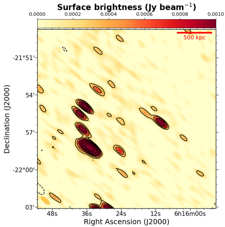
Fig. A.9. RXC J0616.3-2156 JVLA DnC array 1.5 GHz image. Contours start at 3-\sigma_{rms} and are spaced by a factor of 2. 1-\sigma_{rms} = 0.08 mJy/beam with beam= 55.4'' \times 19.9'' .
