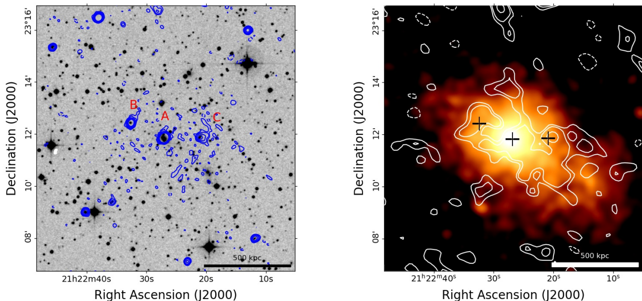
Fig. 6. GMRT images of the cluster Z2120. Left: DSS optical image with GMRT high-resolution contours overlaid. Contours start at 0.1 mJy/beam and are spaced by a factor of two. The first negative contour is dashed. Labels mark the position of discrete sources. Right: GMRT 330 MHz low-resolution ( 32.7'' \times 28'' ) contours after the subtraction of compact sources superimposed on the Chandra X-ray image. Contours are (2, 3, 6, \dots) \times \sigma , with \sigma = 0.3 mJy/beam. The position of the discrete sources is marked with a black cross.
