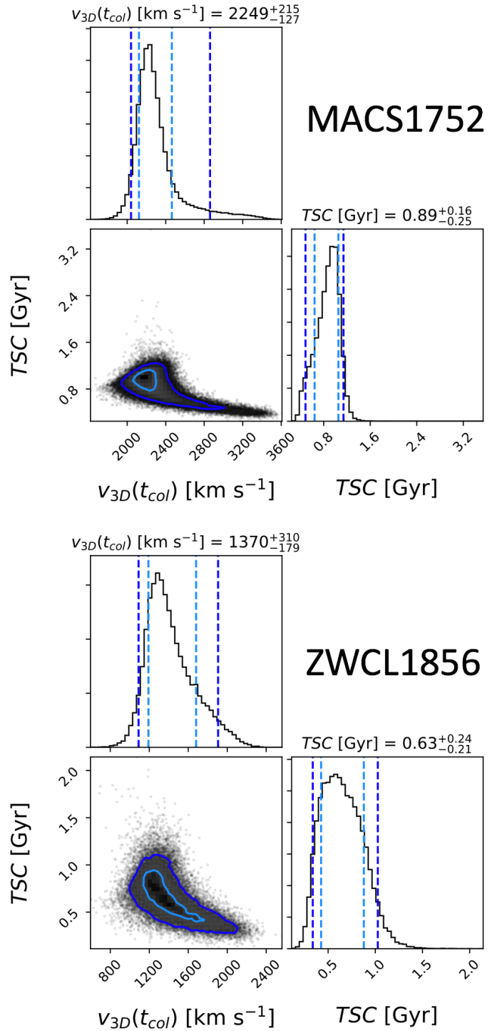
Figure 11. MCMAC results for MACS1752 (top) and ZWCL1856 (bottom). TSC is the time since collision and v_{3D} is the 3D velocity at the time of collision. Light blue lines denote the 1 \sigma level and dark blue denote the 2 \sigma level.
