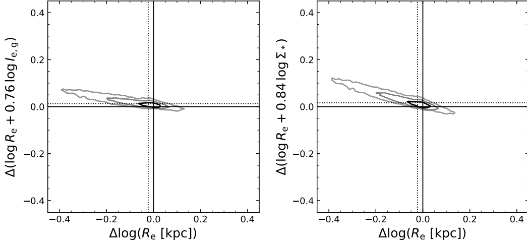
Figure 16. The change in the g -band FP (left) and mass FP (right) due to differences in the size estimates between the Simard et al. (2011) and Meert et al. (2015) catalogs, assuming a fixed tilt from Hyde & Bernardi (2009). Contours enclose 50%, 80% and 90% of the total sample, respectively, and dotted lines indicate the median values. Even a large change in the effective radius results in only a minor difference in the FP, which demonstrates that the uncertainties in \log R_e and \log I_{e,g} or \log \Sigma_* are largely correlated along the FP. As a result, the tilt of the g -band and mass FP depend only very weakly on the choice of the structural parameter catalog used.
