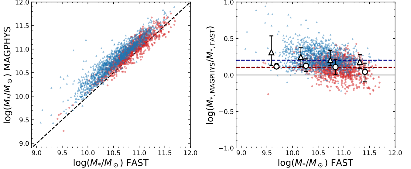
Figure 14. Comparison between the best-fit stellar mass from FAST (van der Wel et al. 2016) and the median of the stellar mass likelihood distribution from MAGPHYS for the primary sample of LEGA-C galaxies. Blue triangles and red circles indicate star-forming and quiescent galaxies respectively. In the right-hand panel, white markers show the median and 16 th and 84 th percentiles, with dashed lines indicating the median offset between the two mass estimates for the two populations. Stellar masses estimated with MAGPHYS are systematically larger than those from FAST, due to significant differences in the assumed star formation histories and dust attenuation model. The offset in stellar mass decreases slightly toward higher (FAST-derived) stellar mass and is larger for star-forming galaxies than quiescent galaxies, consistent with the findings by Leja et al. (2019b).
