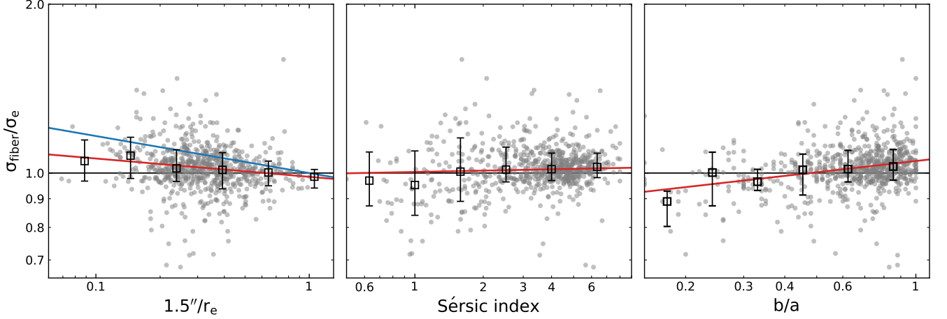
Figure 17. Ratio of the integrated velocity dispersion from the 3'' SDSS fiber spectra and the MaNGA spectra within an aperture of one effective radius, calculated as the flux-weighted second velocity moment. Different panels show the dependence of this ratio on the effective radius, Sérsic index, and axis ratio in gray. Black squares and error bars represent the median and 16 th and 84 th percentiles. Red lines are the best-fit power laws for each parameter. For comparison, the left-hand panel also shows the result by Cappellari et al. (2006) in blue.
