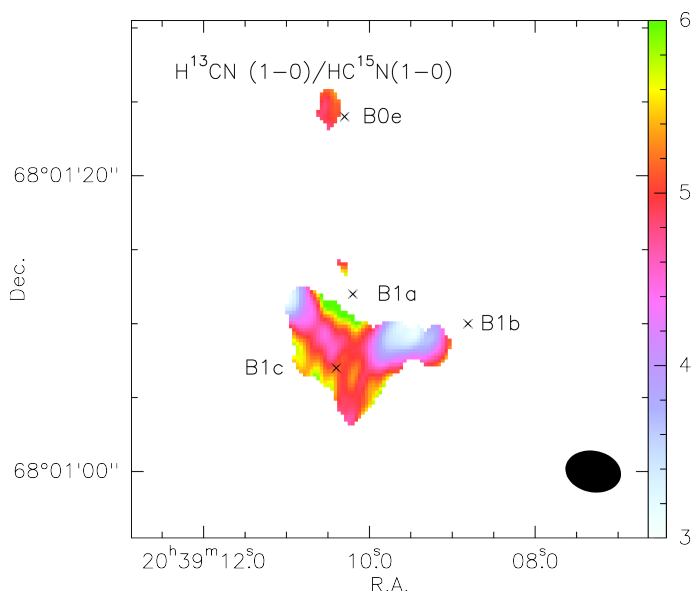
Fig. 4. \text{H}^{13}\text{CN} (1-0)/\text{HC}^{15}\text{N} (1-0) line intensity ratio, only pixels where both lines have signal-to-noise ratio > 5 are considered. The synthesized beam, 3''.8 \times 2''.8 ( \text{PA} = -168^\circ ), is shown in the bottom-right corner.
