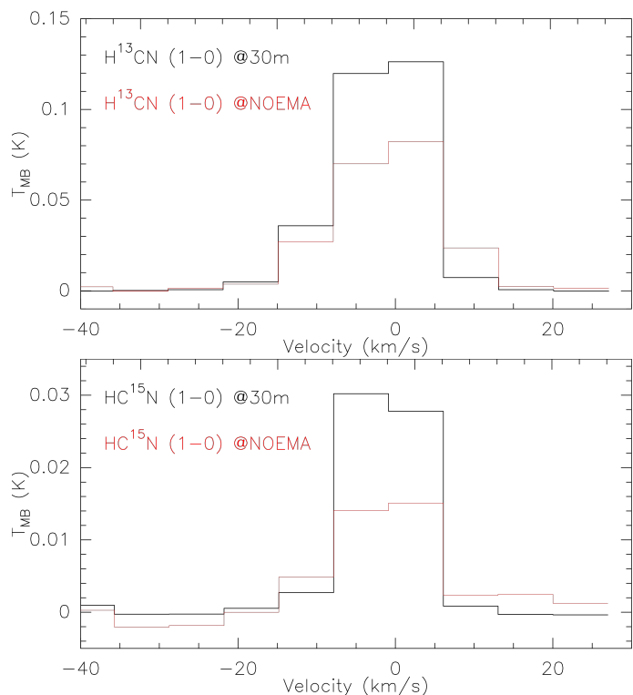
Fig. 1. Top panel: spectra of the \text{H}^{13}\text{CN} (1–0) line as observed with the single dish IRAM 30m telescope towards L1157-B1 (black) and as extracted from the NOEMA cube (red) in a circle equivalent to the HPBW = 28''.5 of the IRAM 30 m telescope and centered in B1. Bottom Panel: the same for the \text{HC}^{15}\text{N} (1–0) line.
