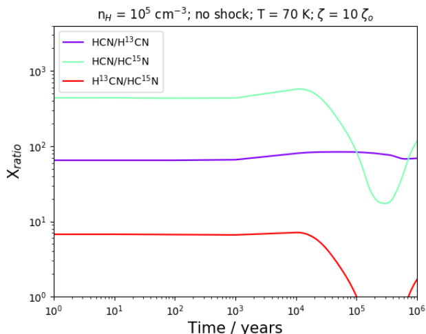
Fig. 6. Chemical abundance ratios of HCN, \text{H}^{13}\text{CN} and \text{HC}^{15}\text{N} as function of time derived from a model where no shock is present but a gas with density n_{\text{H}} = 10^5 \text{ cm}^{-3} was warmed up to 70 K. The cosmic ray ionization rate is \zeta = 3 \times 10^{-16} \text{ s}^{-1} . The time = 0 yr corresponds to the beginning of Phase II when the temperature is increased.
