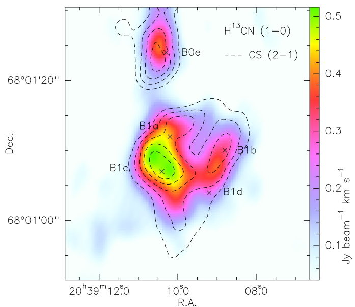
Fig. 3. Maps of the CS (2–1) integrated intensity (black dashed contours, Benedettini et al. 2007) overplotted over the \text{H}^{13}\text{CN} (1–0) integrated intensity (color). For CS level steps are equivalent to 3\sigma , corresponding to 0.026 \text{ Jy beam}^{-1} \text{ km s}^{-1} .
