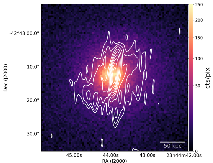
Fig. 4. X-ray (0.7-2 keV) image by Chandra (McDonald et al. 2015). The white contours indicate the L-band emission as observed with the Very Large Array , and are drawn at [-1, 1, 2, 4, 8, \dots] \times 4\sigma_{\text{rms}} , where \sigma_{\text{rms}} = 10.8 \mu\text{Jy beam}^{-1}
