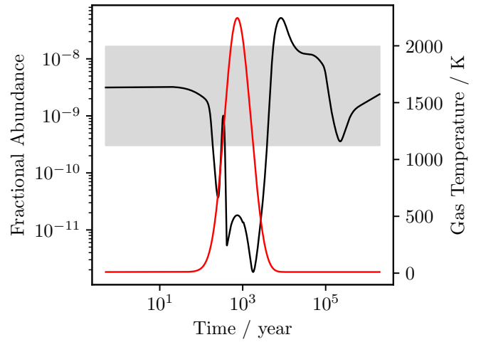
Fig. 9. Fractional abundance of C 2 H through time for a 20 km s -1 shock propagating through gas with a pre-shock density of 10^4 \text{ cm}^{-3} plotted in black, temperature through the shock plotted in red. The range of observed C 2 H abundances is shown in grey.
