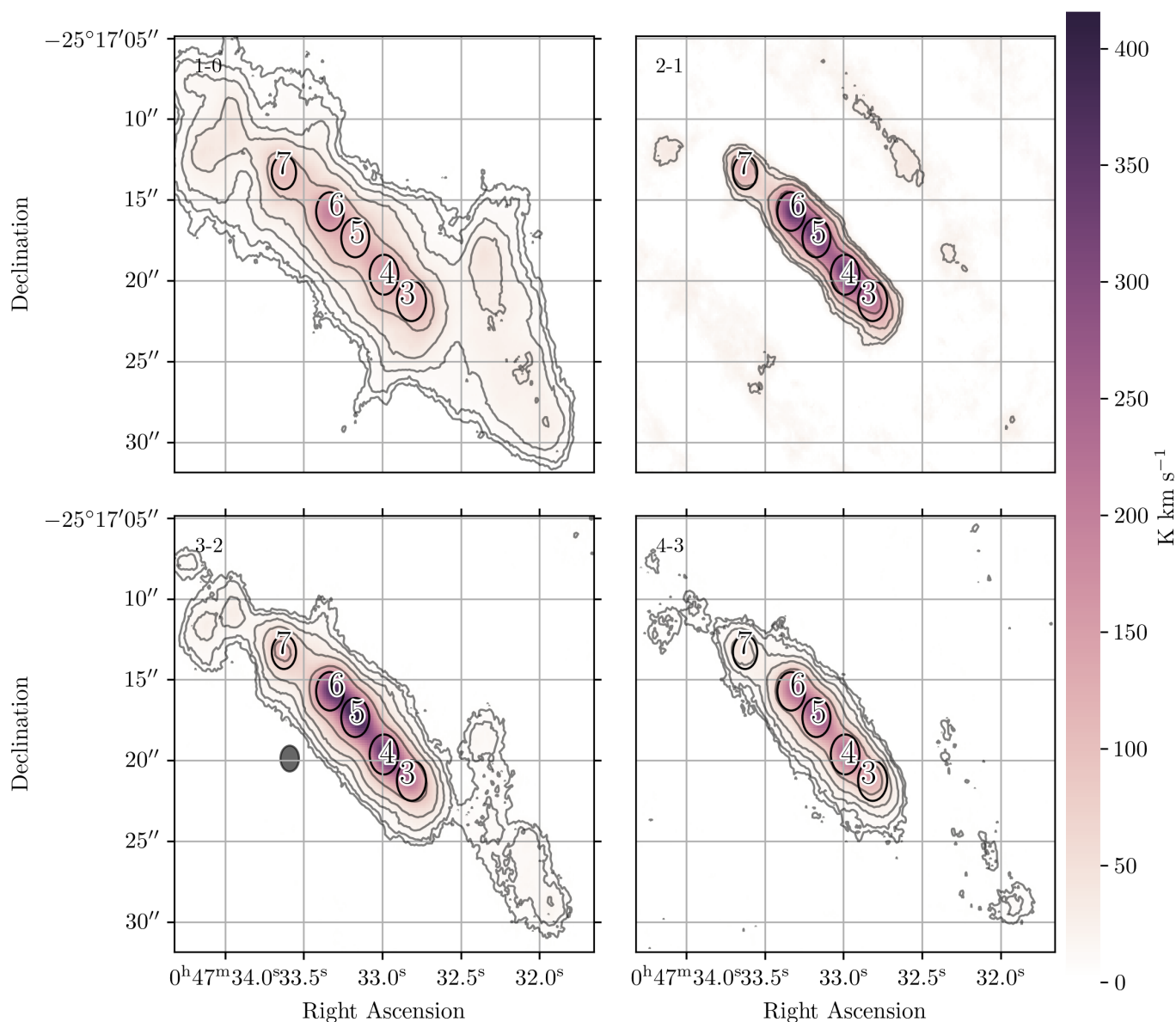
Fig. 1. Integrated emission maps of C_2H in NGC 253. The beam size for all panels is 1.6'' and is shown in the bottom left panel. Since the beam size is shared, the wider spatial distribution of the N=1-0 emission is not caused by a beam size effect. Contours at the 3, 5, 10, 20 and 50\sigma level are drawn in black. The noise levels in order of increasing N are 1.4, 8.5, 2.0 and 1.6 \text{ K km s}^{-1} . Each ellipse shows the position and size of the Gaussian fits to the four individual clumps described in section 3.1. The numbers indicate the position of the GMCs in Leroy et al. (2018)
