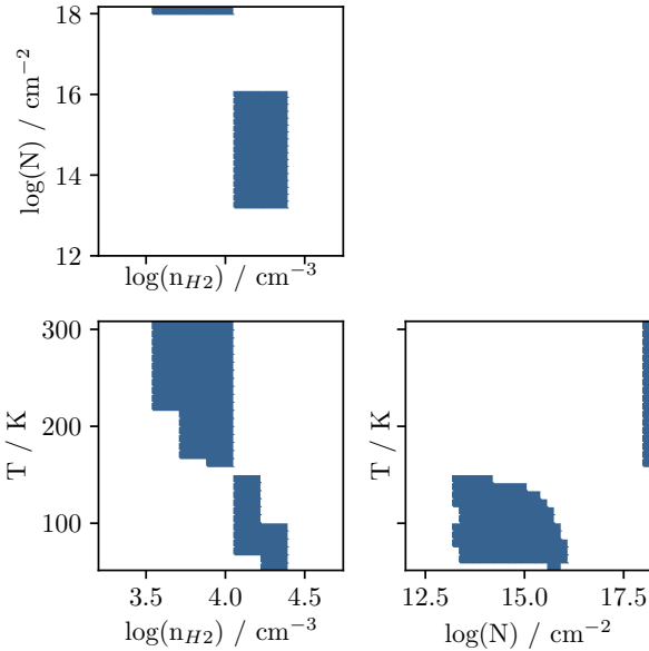
Fig. 4. Model parameters that fit constraints from the extended emission of the CMZ. Each point represents the parameters of a model where the N=1-0 line was the strongest line and was above noise.
