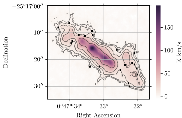
Fig. 2. Integrated emission map of the C 2 H N=1-0 multiplet as in Figure 1 but showing the full extent of the emission. Contours are shown at the 3, 5, 10, 20 and 50 \sigma levels for noise level of \sigma=1.5 K km s -1 . Black squares indicate the positions sampled for spectra in Figure 3.
