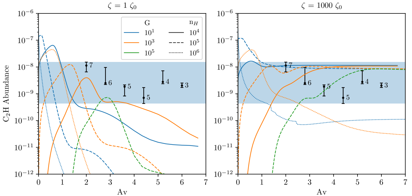
Fig. 6. Fractional abundance as a function of depth into the cloud from PDR modelling and observations. The depth into the cloud is given as the equivalent visual extinction. The black dots are numbered according to the GMC they represent and error bars show the observed abundance towards that GMC, their position on the x-axis is arbitrary and does not represent the cloud sizes. The lines show UCL_PDR models with different parameters. The shaded band covers the abundance range of all GMC measurements. In the low cosmic-ray ionization rate models (left), the abundance decreases with distance into the cloud so the total column density is less than the observed column density despite the high abundances reached at low A_v .
