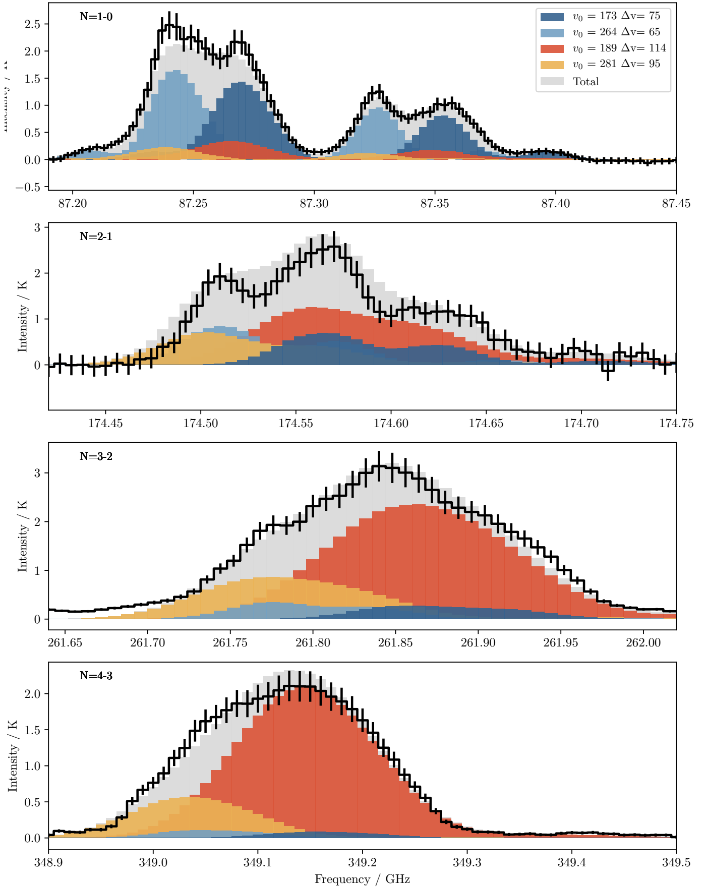
Fig. 5. Best fit model for GMC 5. The black trace shows the measured spectra with error bars. The histograms show the spectral model components in colour and their total in grey. The legend gives the central velocity ( V_0 ) and linewidth ( \Delta V ) of each component. The two blue components are the low density CMZ contribution and the others are the high density GMC components.
