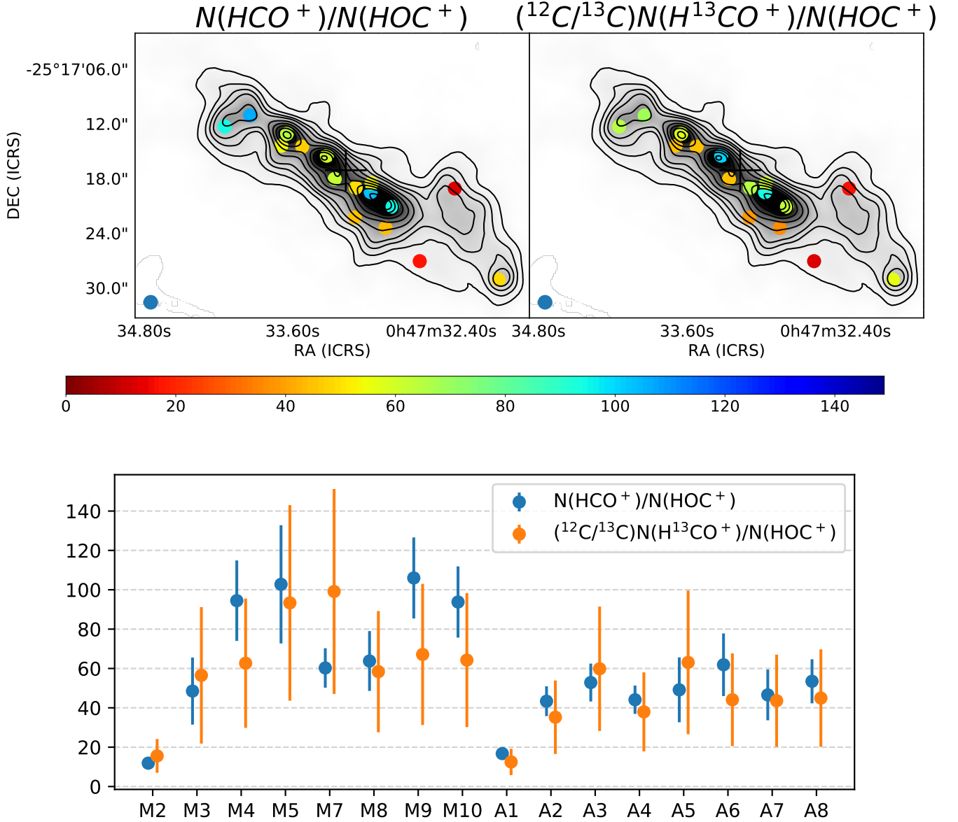
Figure 7. Abundance ratios of \text{HCO}^+/\text{HOC}^+ plotted as colored dots over \text{HCO}^+ moment 0 images (greyscale + contours) using N(\text{HCO}^+)/N(\text{HOC}^+) (Method 1, top left) and (^{12}\text{C}/^{13}\text{C})N(\text{H}^{13}\text{CO}^+)/N(\text{HOC}^+) (Method 2, top right). The \text{HCO}^+/\text{HOC}^+ abundance ratios estimated from two methods in top panels are shown for individual positions together with error bars (bottom).
