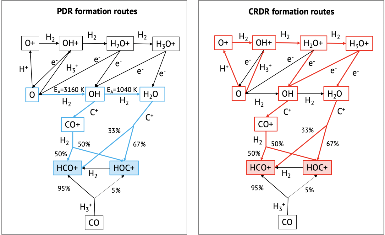
Figure 8. Graphical presentation of formation routes of \text{HCO}^+ and \text{HOC}^+ in the cases of PDRs and CRDRs. The blue boxes and arrows are species and reactions involved in the formation of \text{HCO}^+ and \text{HOC}^+ in PDRs, while red boxes and arrows are the ones in CRDRs. The activation barriers in the gas-phase formation of OH and water are indicated as E_A .
