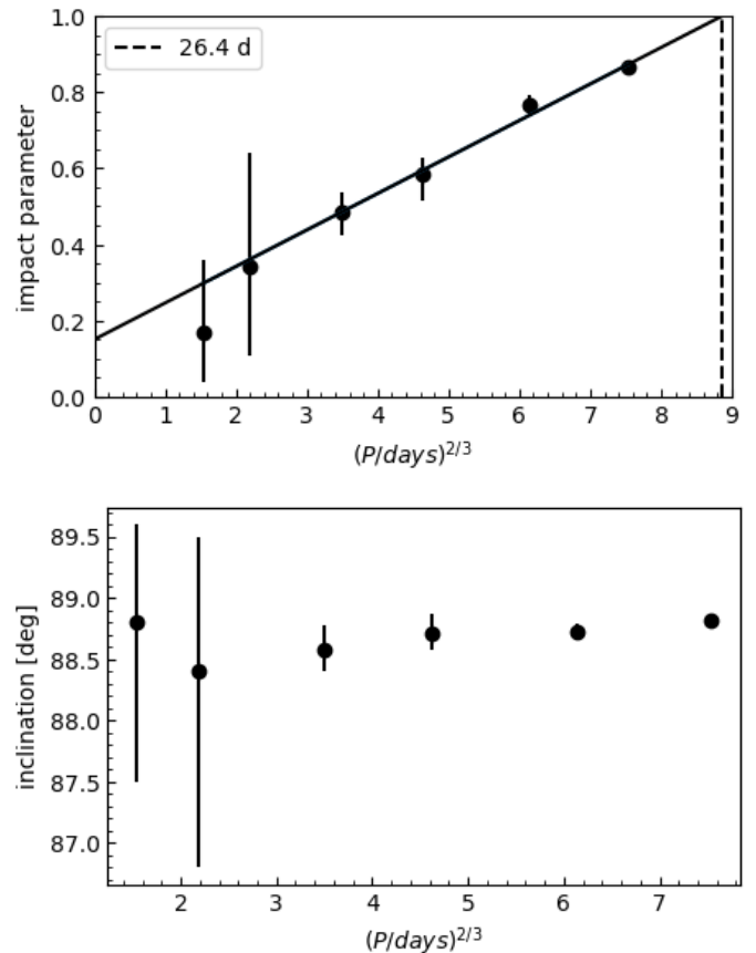
Fig. 8. Impact parameter (top) and inclination (bottom) of the six planets of the TOI-178 system. In the top panel, the solid line shows the evolution of the impact parameter as a function of the period assuming that all planets are in the same plane (obtained by linear fit). The dashed line shows that an outer planet in the same plane will not transit if its period is above 26.4 d.
