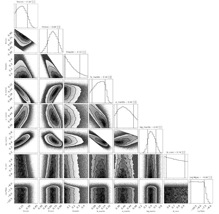
Fig. D.2. Corner plot showing the main parameters of the internal structure of planet b . The parameters are: the core mass fraction; the mantle mass fraction; the water mass fraction (all relative to the solid planet); the molar fractions of Fe, Si, and Mg in the mantle; the molar fraction of Fe in the core; and the mass of gas (log scale). The dashed lines give the positions of the 16% and 84% quantiles, and the number at the top of each column gives the median and the 16% and 84% quantiles.
