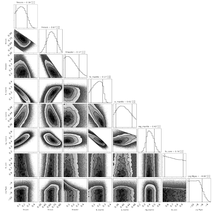
Fig. D.3. Same as Fig. D.2 but for planet c .
