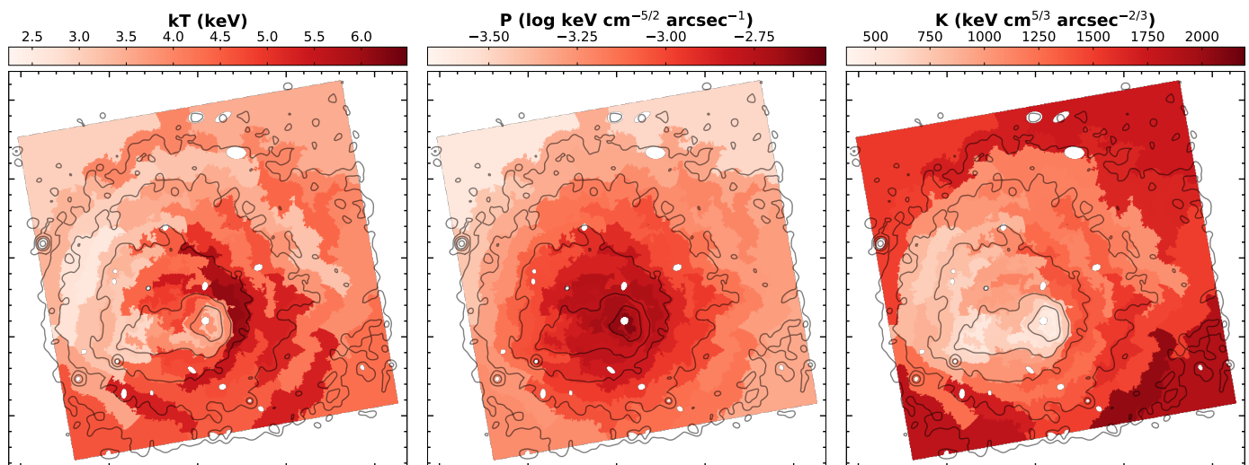
Fig. 3. Temperature ( left ), pseudo-pressure ( center ), and pseudo-entropy ( right ) maps with overlaid the Chandra contours. The white ellipses mark the regions where point sources were removed. The typical fractional error in each region is in the range \sim 5 - 10\% . The temperature error map is shown in Appendix B.
