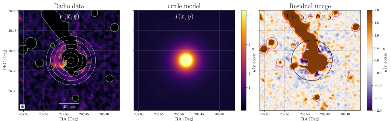
Fig. 11. Fitting result obtained with HALO-FDCA (Boxelaar et al., submitted). Left: LOFAR low-resolution image used for the fit. Contaminating regions are masked out and contoured in green. The circular contours show the model at [1, 2, 4, \dots, 32] \times \sigma levels. Center: image of the best-fit circular model. Right: residual image of the fit. The circle shows the 2\sigma level of the model. The red contours shows the masked regions. The \chi^2/\text{d.o.f.} of the fit is 1422.35/828. The MCMC corner plot of the fit is reported in Appendix B.
