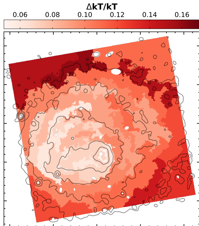
Fig. B.1. Temperature error map corresponding to Fig. 3.
