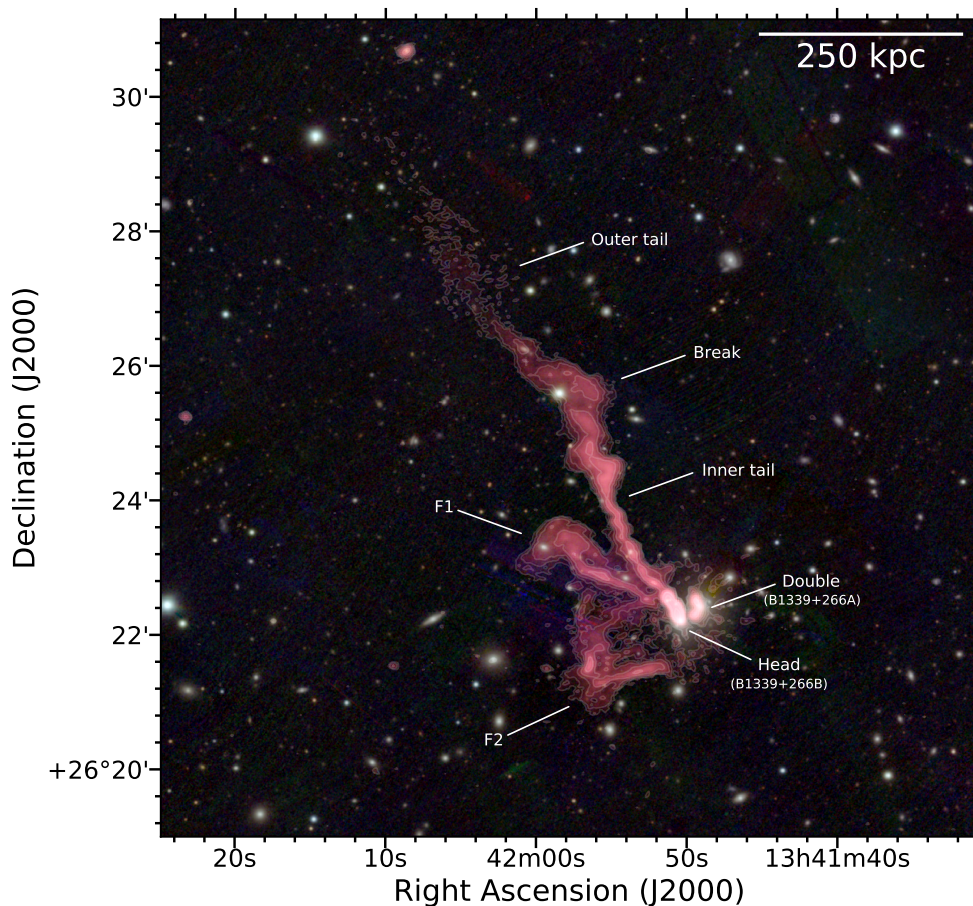
Fig. 6. Composite radio/optical image obtained from Pan-STARRS g, r, i and LOFAR 144 MHz high-resolution ( 5'' \times 3'' ) data. Radio contours start from 3\sigma , where \sigma = 148 \mu\text{Jy beam}^{-1} , and are spaced by a factor of 2. The main features discussed in the text are labeled in the figure.
