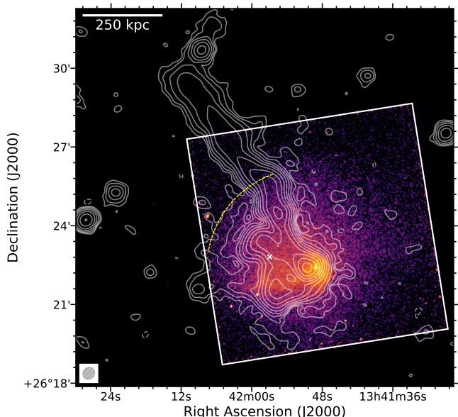
Fig. 10. The low-resolution ( 29'' \times 26'' ) LOFAR contours overlaid on the Chandra image. Contours are spaced by a factor of 2 starting from 3\sigma , where \sigma = 255 \mu\text{Jy beam}^{-1} . The beam is shown in the bottom left corner. The dashed yellow arc marks the position of the cold front traced by the X-ray surface brightness discontinuity of Fig. 4 while the white cross denotes the center the circular model shown in Fig. 11.
