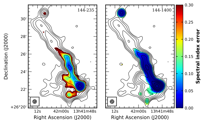
Fig. B.2. Spectral index error maps corresponding to Fig. 9.
