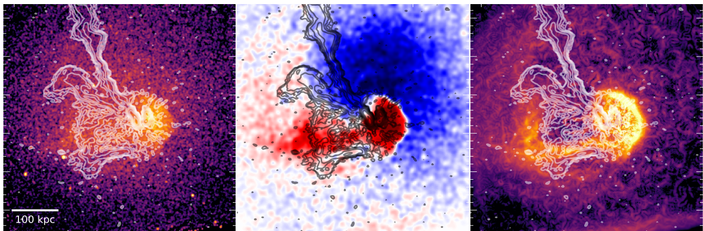
Fig. 12. Zoom-in of the central cluster region. From left to right, the LOFAR high-resolution contours of Fig. 6 are overlaid on the Chandra X-ray image, residual map, and GGM-filtered image of Figs. 1 and 2.
