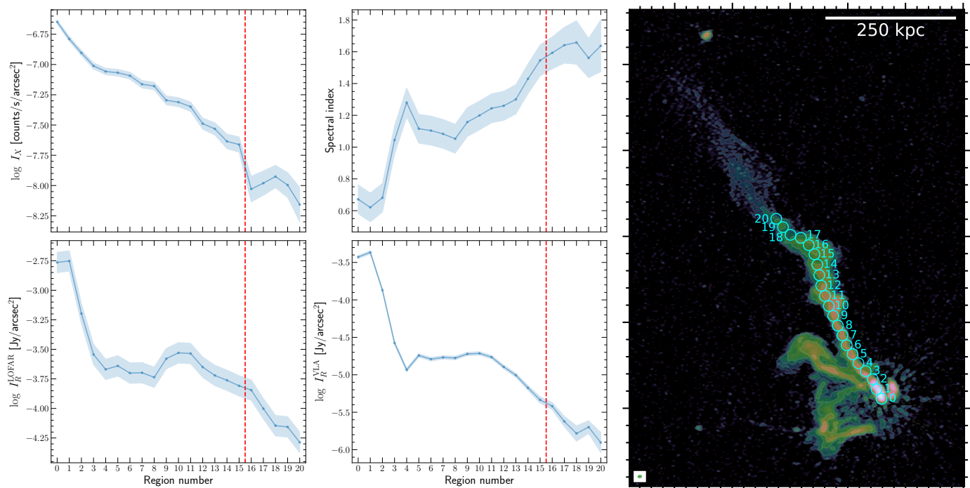
Fig. 13. Spectral index, LOFAR and VLA radio surface brightness ( I_R ), and Chandra X-ray surface brightness ( I_X ) trends along the head-tail radio galaxy. Radio surface brightnesses and spectral index were computed from LOFAR and VLA C-array images with a beam of 15'' \times 15'' . Measurements were performed in the cyan beam-sized circular regions reported in the right panel, which depicts the same LOFAR high-resolution image of Fig. 6 only for visualization purposes (the beam is shown in the bottom left corner). Regions are numbered from 0 (head of the tail) to 20 (last region where the VLA emission is > 3\sigma ). The red dashed vertical line on the left panels denotes the location of the arc-shaped cold front.
